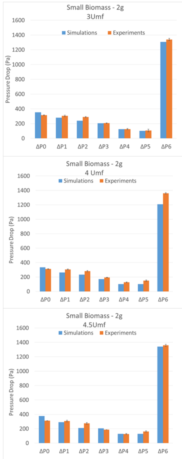
Figure 15: Comparison of the pressure drops for the small size biomass (2 g) – experiments vs. DEM simulations.
