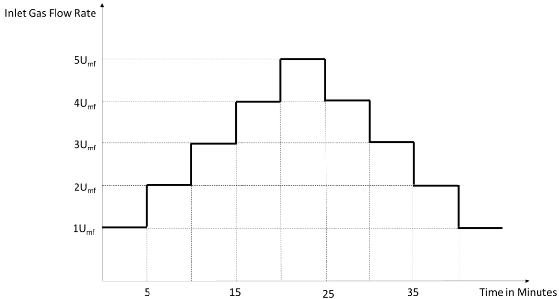
Figure 8: Variation of the inlet gas flow rate (velocity) during the laboratory fluidization tests.
