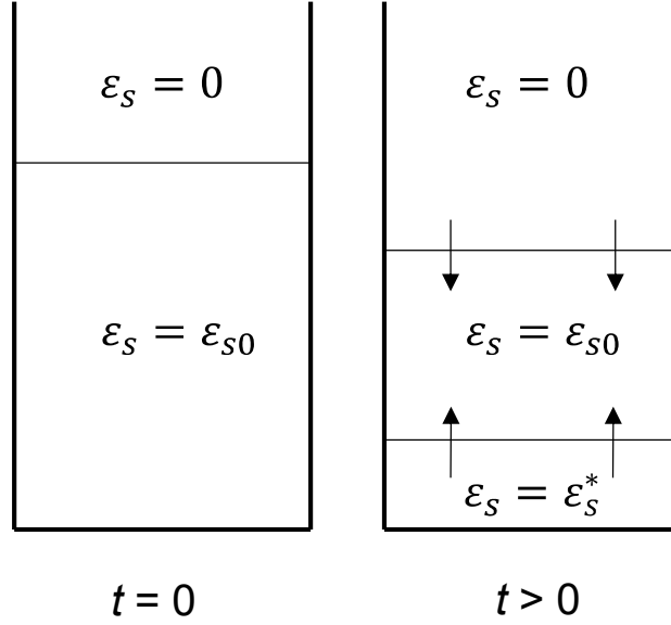
Figure 15: Schematic showing the settling problem.
