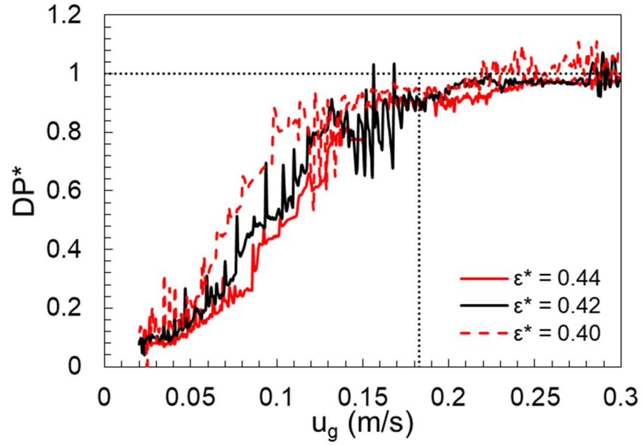
Figure 12: Effect of varying volume fraction at packing.
