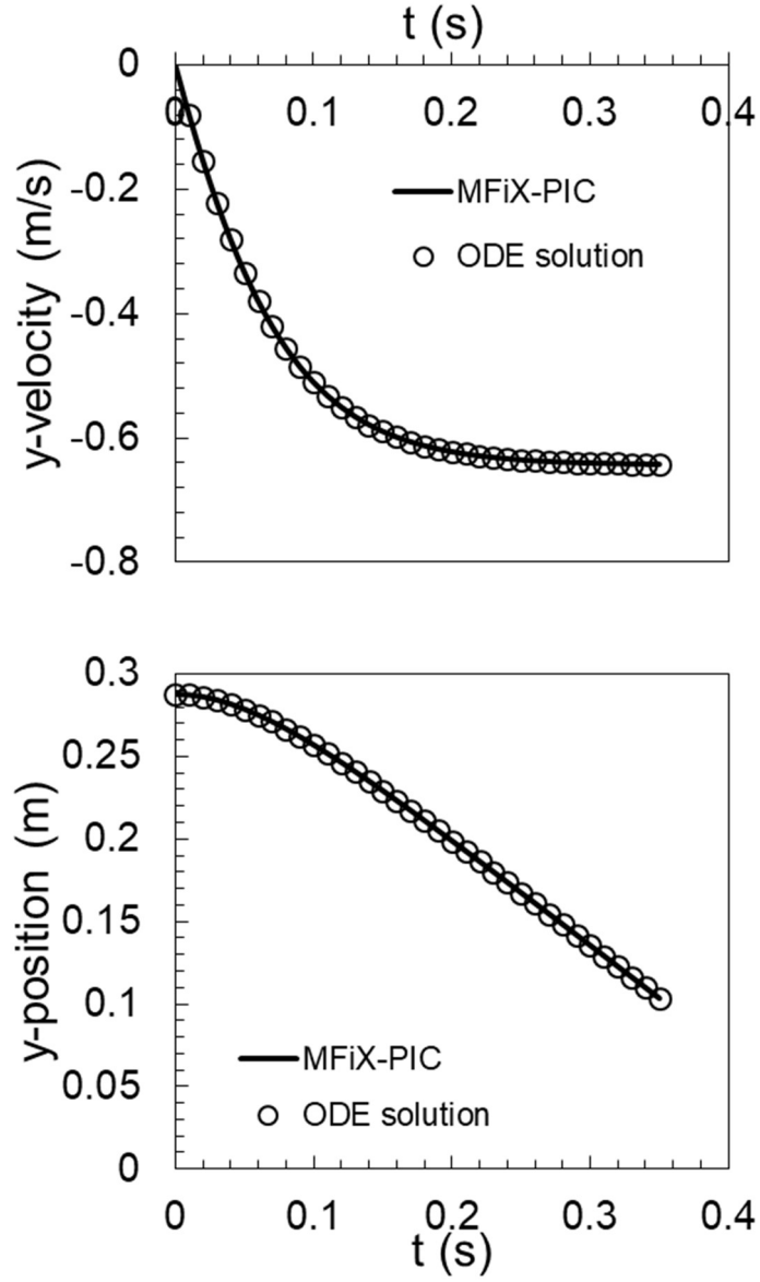
Figure 1: Predictions using MFiX-PIC: velocity (top) and position (bottom).
