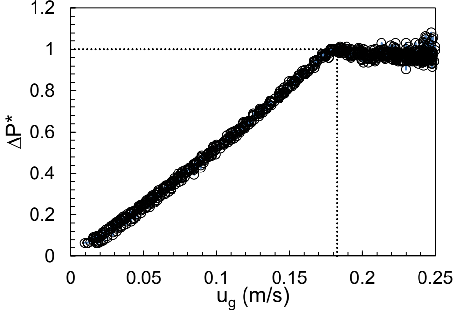
Figure 9: Normalized pressure drop as a function of inlet gas velocity.
