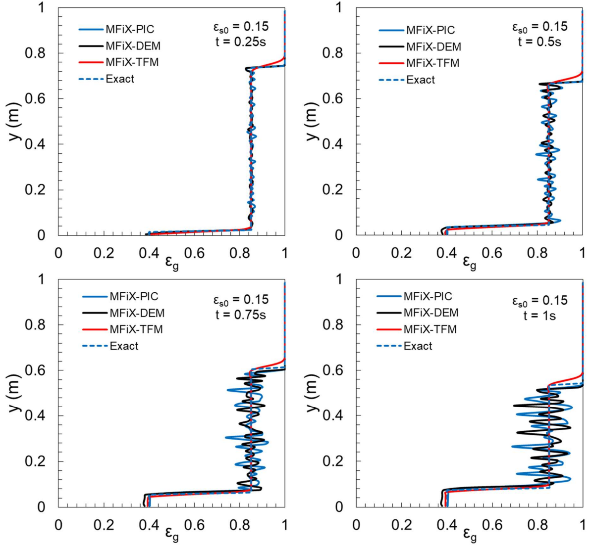
Figure 5: Time evolution of shock fronts, initial particle concentration \varepsilon_{s0} = 0.15 .
