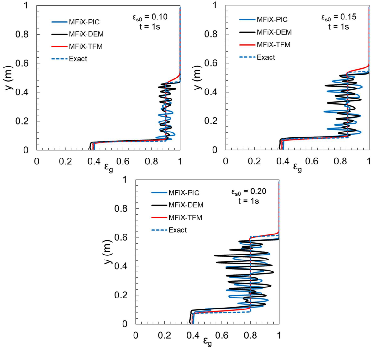
Figure 4: Solutions for different initial particle concentration \epsilon_{s0} = (a) 0.10, (b) 0.15, (c) 0.20.
