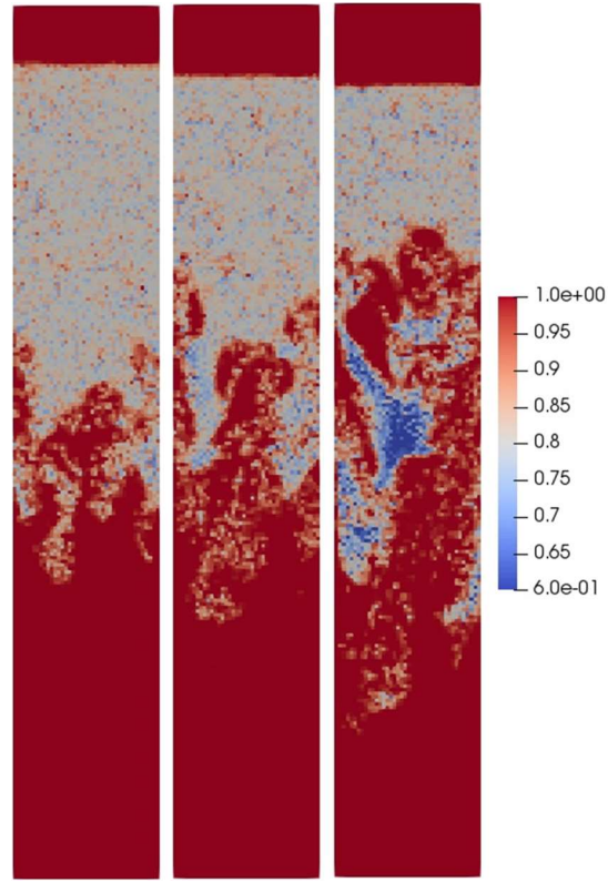
Figure 7: Sectional view of volume fraction contour of the lighter phase at t = 0.8s ; A = 0.1667, 0.2857 , and 0.4737 (left to right).
