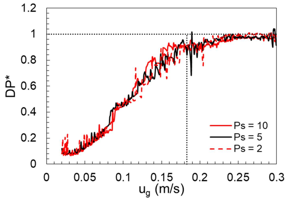
Figure 11: Effect of varying P_s .
