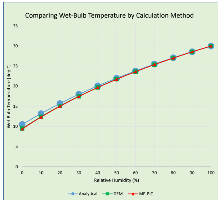
Figure 6: Comparison of wet bulb temperatures between data, MFIX-DEM and MFIX-PIC.
