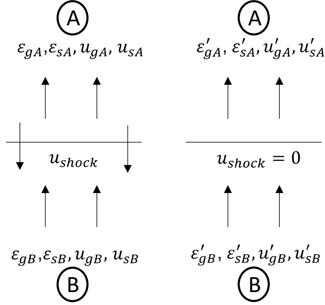
Figure 16: Laboratory (left) and traveling (right) frame of references for the kinematic shock wave.
