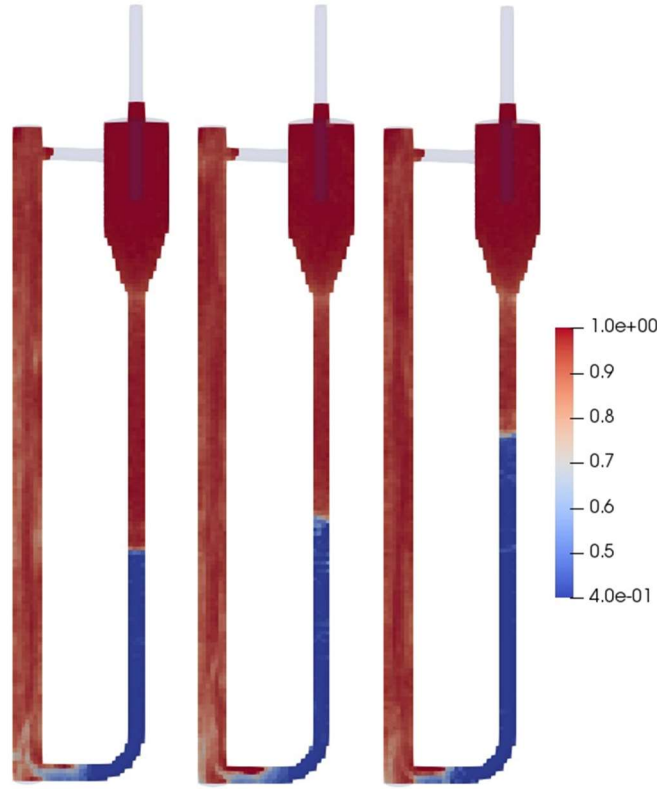
Figure 14: Cross-sectional view (Z-normal) of gas volume fraction contours at t = 20 seconds for Case 1, 2 and 3 (left to right).
