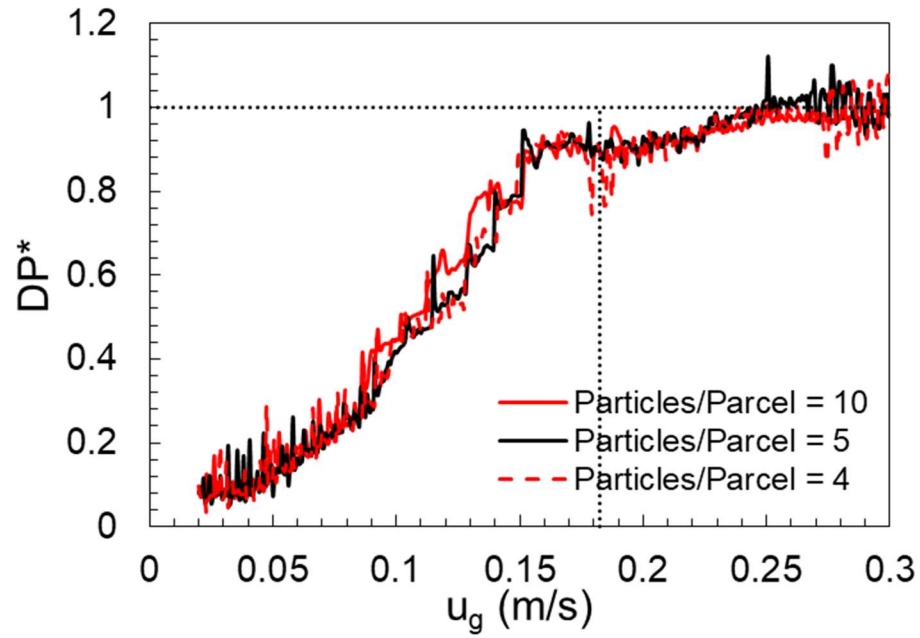
Figure 10: Effect of statistical weight (particles per parcel) on fluidization curve using MFIX-PIC.
