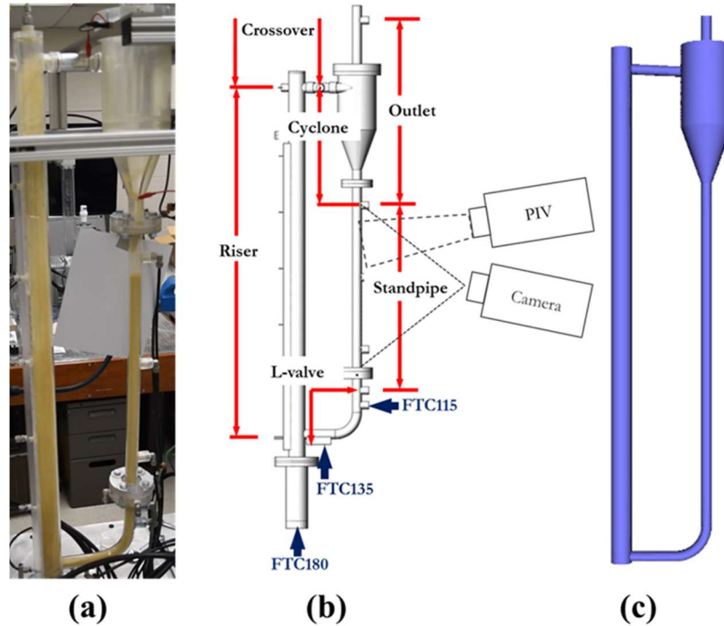
Figure 13: Circulating fluidized bed experiments and computational set-up: (a) snapshot of the experimental facility, (b) schematic of the experimental set-up, and (c) geometry used for simulations.
