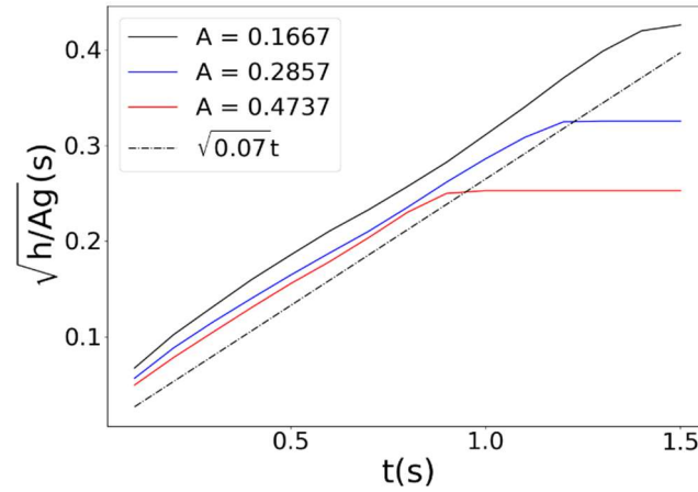
Figure 8: Evolution of mixing layer for A = 0.1667, 0.2857 , and 0.4737 . The dashed line is the theoretical solution, Equation (28) where \alpha = 0.07 .
