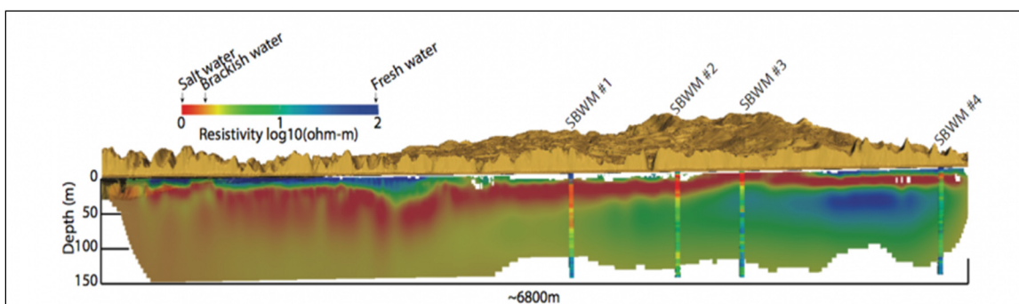
Figure 3.3.3. A surface geophysical method, electrical resistivity tomography (ERT), is used to image seawater intrusion along the coast of Monterey Bay, California. Imaging reveals a complex distribution of subsurface fresh and saltwater, influenced by geology, groundwater pumping, recharge, and land use.
