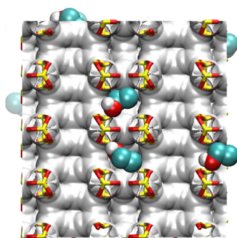
Figure 3.1.6. Model predictions and comparison with experimental data for ethanol adsorption in zeolites from an aqueous solution. (Courtesy of Ilja Siepmann.)
