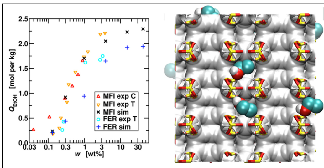
Figure 2.1.6. Experimental adsorption data provide validation for the prediction that zeolite FER (ferrierite) is a highly selective sorbent for the extraction of ethanol from aqueous solution. The snapshot on the right illustrates that ethanol molecules are preferentially adsorbed in sites that do not allow for water molecules to hydrogen bond with multiple ethanol molecules.
