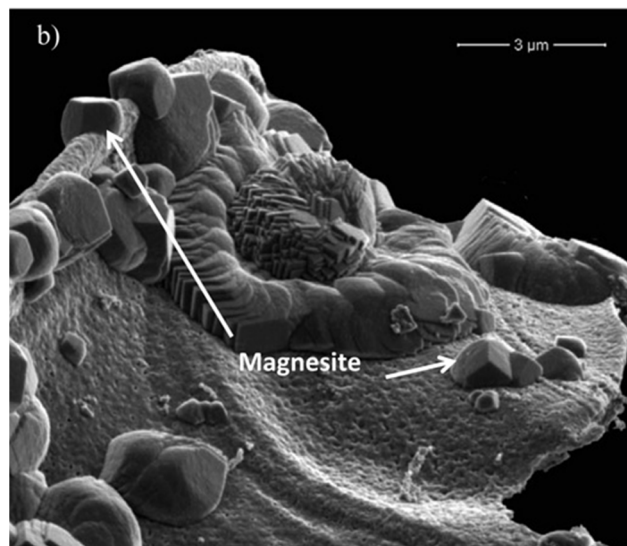
Figure 2.1.5. SEM image of the products of the reaction of forsterite, \text{Mg}_2\text{SiO}_4 , in water saturated at \text{CO}_2 35°C and 90 atm pressure for 14 days. The formation of magnesite, \text{MgCO}_3 , must involve mineral reactions in thin surface water films.
