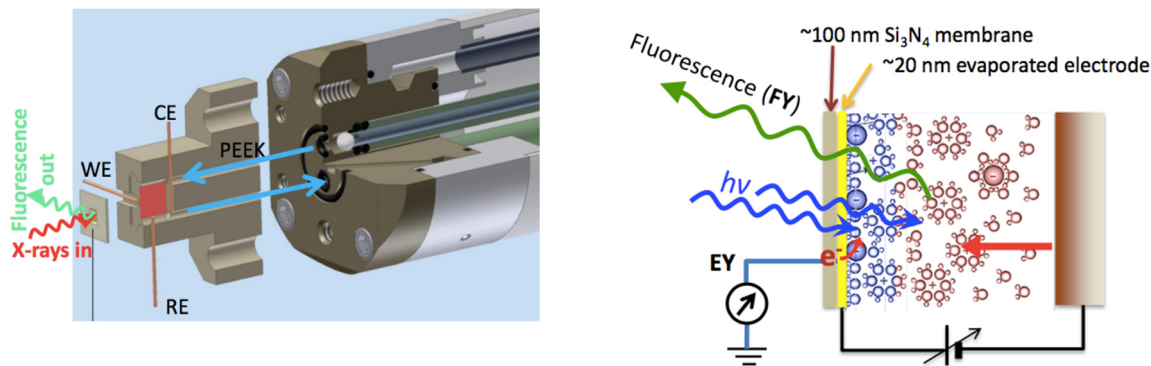
Figure 2.2.5. Synchrotron measurements can be performed on an electrochemical cell in operando. New approaches, based on the combined interrogation of the sample using high-intensity x-rays available at synchrotrons, and UV-visible photons ( h\nu ), have the potential, via simultaneous measurement of fluorescence, to provide new information on the structure of water at the interface. WE, RE, and CE are working, reference, and counter electrodes, respectively. FY and EY are fluorescence and electron yields. PEEK is polyetheretherketone, which is the material that makes up the flow cell.
