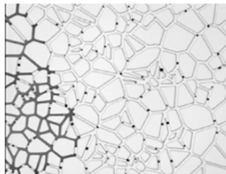
Figure 3.4.3. Microfluidic porous media models for pore size of 4–8 \mu\text{m} .
