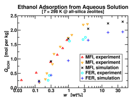
Figure 3.1.6. Model predictions and comparison with experimental data for ethanol adsorption in zeolites from an aqueous solution. (Courtesy of Ilja Siepmann.)
