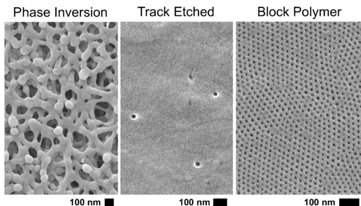
Figure 3.1.3. Meso- to nano-porous membrane structures with tunable pore entries and walls. (Courtesy of William Phillip.)
