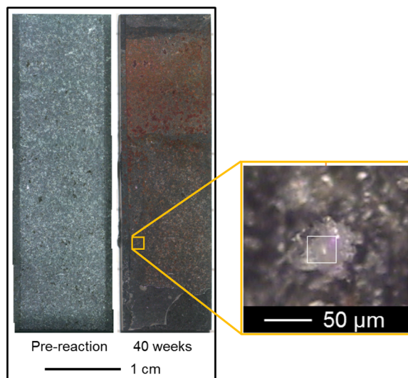
Figure 3.2.3. Surface of a 100-μm-wide fracture of a Columbia River flood basalt before and after reaction in water-saturated supercritical CO 2 at 100 C and 100 bar. The top of the fracture was open to the wet CO 2 , and the bottom of the fracture was sealed. Upon reaction with the wet CO 2 , iron(II) in silicate minerals was oxidized to form red iron oxide products and calcium carbonate (aragonite shown in the electron micrograph) precipitated from reaction of the wet CO 2 with calcium released from the basalt. Data from W. Xiong, 2017, Ph.D. thesis, Washington University in St. Louis.
