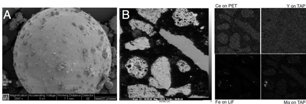
Figure 2.2.4. A – SEM of an amorphous particle obtained from coal ash. (Courtesy of H. Hsu-Kim.) B – SEM of sections of glass fly ash particles from a coal power plant (left panel) and associated elemental distribution maps (right panels).
