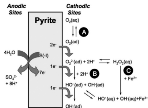
Figure 2.4.4. Mineral-induced reactive oxygen species (ROS) formation: Pyrite is an example of a mineral that can be useful for water treatment. Pyrite spontaneously produces hydrogen peroxide and hydroxyl radical ROS when dispersed in water through a series of stepwise reactions involving dissolved oxygen. The formation of ROS can be leveraged in strategies to kill waterborne pathogens and to degrade persistent organic pollutants. Other natural materials known to spontaneously produce ROS include specific clays, olivine, and magnetite. The figure illustrates the stepwise reduction pathway.
