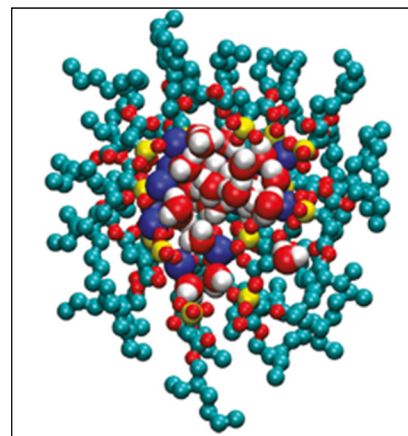
Figure 3.1.4. Simulation of water confined within a surfactant reverse micelle.
