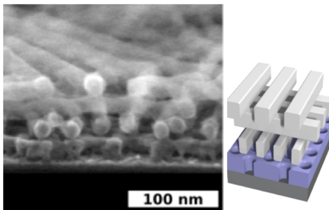
Figure 3.4.1. Three-dimensional block-copolymer morphologies that may be leveraged for the development of multi-functional membranes.
