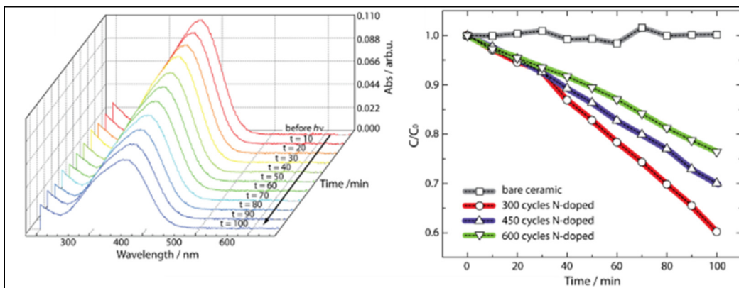
Figure 2.3.4. Visible-light photocatalytic degradation of organic molecules using novel doped semiconductor coatings.
