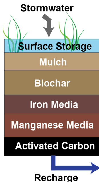
Figure 3.3.5. Example of engineered in situ geomaterial strategy for treating urban stormwater (modified from [18]). Existing systems typically rely on infiltration through native soil or sand/soil mixtures. Large variations in moisture content and the need to control the timescales of infiltration relative to the timescales of the chemical reactions pose challenges for treatment. Significant opportunities exist to develop new materials for in situ water treatment that are finely tuned on the basis of fundamental understanding of infiltration and reaction processes and their timescales.
