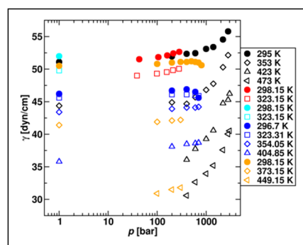
Figure 2.1.8. Compilation of experimental data for the interfacial tension of the water/ n -decane system over a wide range of pressures and temperatures. The colors distinguish five literature sources, and the symbol types correspond to different temperature intervals (with filled symbols highlighting data at T \approx 298 K). A significant data spread is found even at ambient conditions, and high-pressure data do not agree on whether the interfacial tension increases or decreases with pressure.
