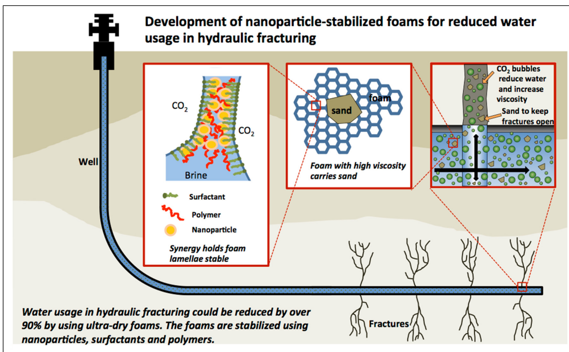
Figure 2.1.9. Replacement of standard hydraulic fracturing fluids by ultra-dry foams, composed primarily of CO 2 and organic or inorganic surfactants, could reduce water use for tight shale gas extraction by up to 90%. (Courtesy of Maša Prodanović, The University of Texas at Austin.)
