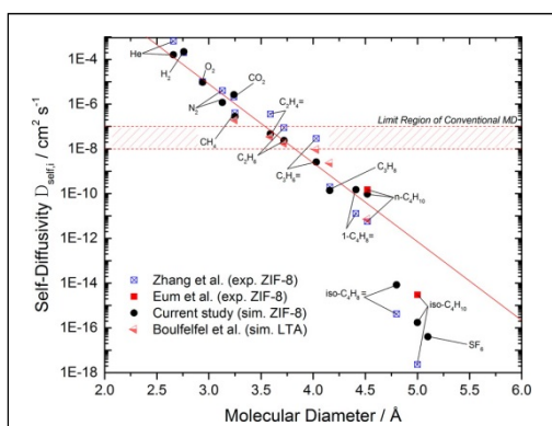
Figure 2.1.7. Comparison of measured and predicted infinite-dilution self-diffusion coefficients for small molecules and light key hydrocarbons at 308 K as a function of molecular diameter in ZIF-8, a prototypical metal-organic framework material.
