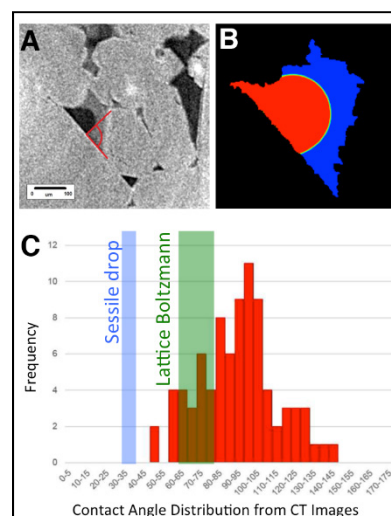
Figure 2.2.9. Measurement and prediction of the wetting angle of a CO 2 bubble within a brine-saturated porous rock. A — X-ray computed tomography image. B — Predicted contact angle from lattice Boltzmann simulation. C — Comparison of observed and predicted wetting angles. (Courtesy of J. Tudek et al.)
