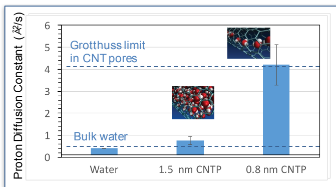
Figure 2.2.7. Confinement effects can enhance transport, such as in the significant increase in proton diffusion through small-diameter carbon nanotubes.
