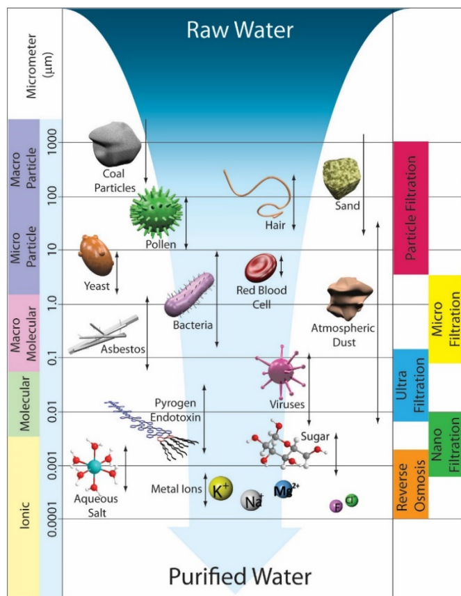
Figure 2.2.8. Size regimes of membranes.
