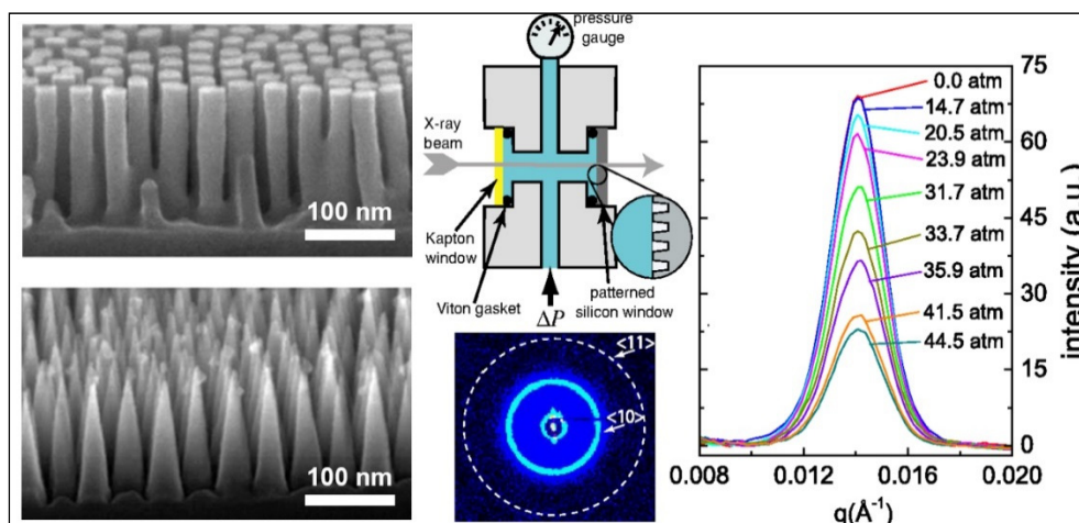
Figure 2.3.3. Small-angle x-ray scattering (SAXS) characterization of water infiltration. The study of new materials for the energy-water issues requires the development and leveraging of techniques to study buried and hydrated interfaces in realistic conditions at relevant time and concentration levels.
