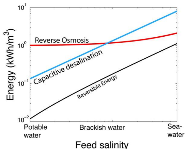
Figure 2.2.12. Calculated energy demands for desalinating water with varying salt concentrations using CDI or RO, compared to the thermodynamic limit. (Courtesy of M. Stadermann.)
