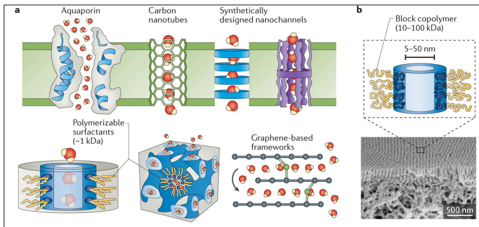
Figure 2.3.5. Molecular design of selective membranes through the insertion of various types of amphiphilic molecules pore-forming structures.
