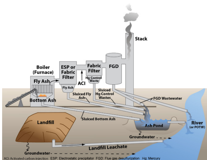
Figure 3.1.1. Key waste streams in coal-fired steam electric power plants.
