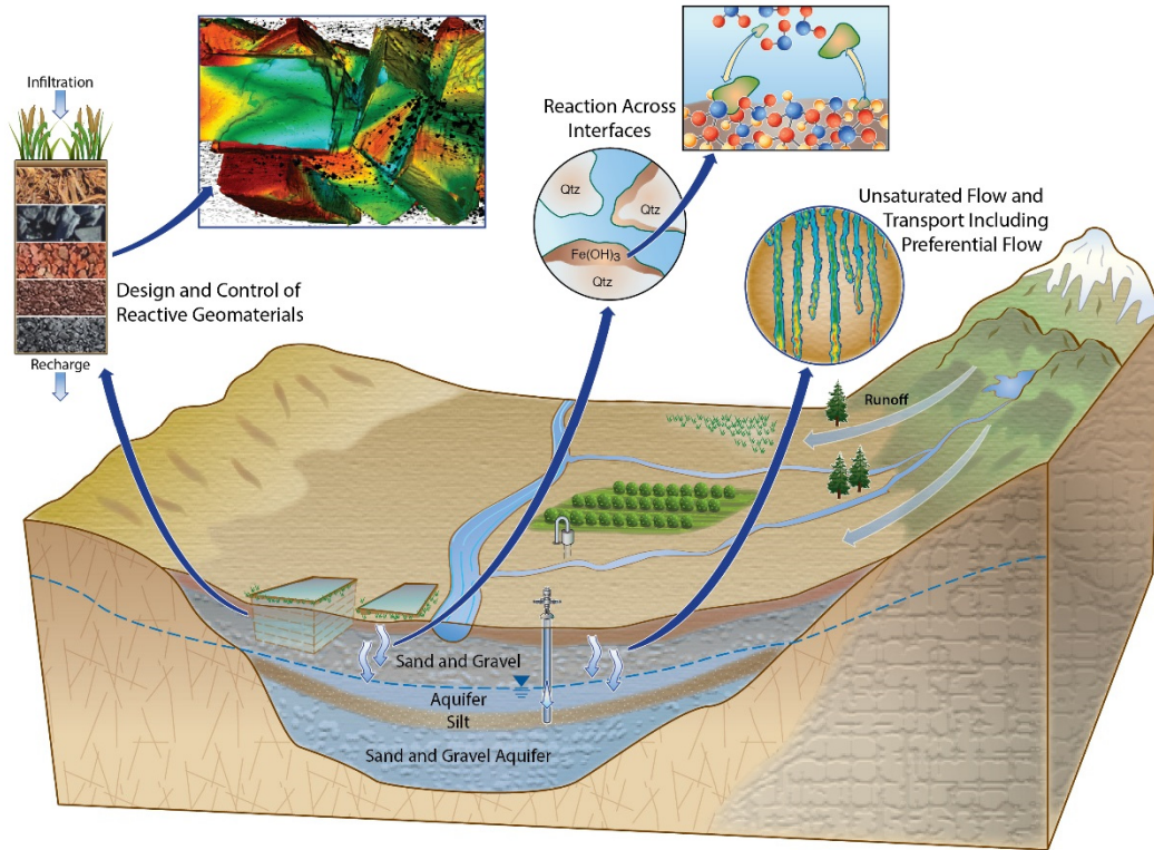
Figure 2.4.1. Advancing predictive control of the subsurface for in situ water storage and treatment requires quantification of complex fluid behavior, control of reactions across interfaces, and design of material-fluid interactions — all of the PRD challenges described above — as well as their manifestation in the context of natural heterogeneity and large-scale hydrological and geochemical gradients and transients. Quantifying and predicting coupled geochemical, hydrological, geomechanical, and biological processes that occur at native scales, their cumulative influence on the behavior of natural aquifer systems, and the design of in situ approaches that can lead to game-changing water treatment or storage benefits are grand challenges. (Courtesy of Susan Hubbard, Lawrence Berkeley National Laboratory.)
