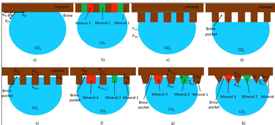
Figure 2.3.2. The wetting of mineral surfaces by immiscible fluids is strongly affected by structural, compositional, and surface chemical heterogeneity.
