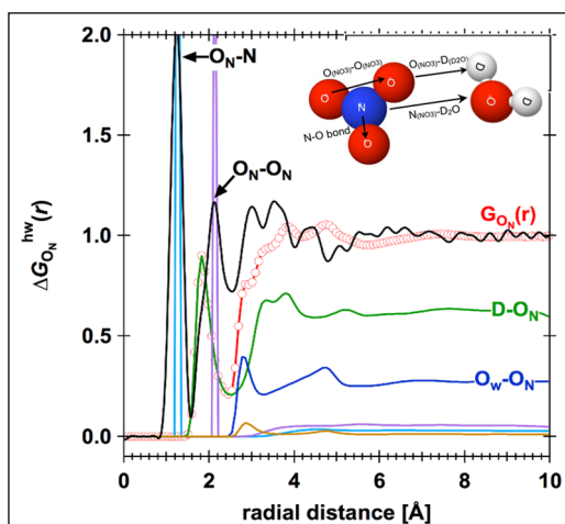
Figure 2.1.3. Combined computational simulation with neutron/x-ray scattering. Neutron pair distribution function analysis and molecular dynamics simulation of aqueous nitrate ion. The experimental data, in black, are directly compared and interpreted using the computational simulation, including peak assignments, position, and ion pair formation. New algorithm developments are enabling simulation of combined x-ray and neutron scattering data in order to understand solvation phenomena such as ion pair structure and stability. Since water is a polarizable environment, the description of some features on anion hydration behavior are improved by the use of models involving induced-dipole polarization. These data also provide an opportunity for force-field development and optimization.
