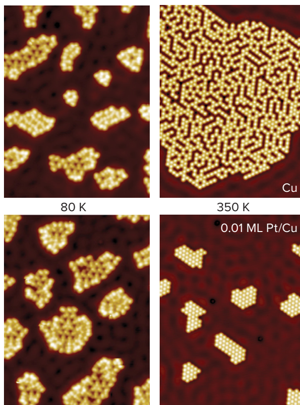
Figure 1.6. STM images, recorded at 5 K, show \text{CH}_3\text{I} adsorbed on \text{Cu}(111) and 0.01 ML \text{Pt}/\text{Cu}(111) surfaces (top and bottom rows, respectively), after annealing to 80 K (left, showing clusters of intact \text{CH}_3\text{I} molecules), and 350 K (right, dissociated iodine atoms appear as brighter protrusions, while methyl groups appear as darker protrusions). The loss of methyl groups from the Pt-containing surface is a consequence of C–H activation and formation of methane. Reprinted with permission from Nature Chemistry , 10, 325–332, 2018, Pt/Cu single-atom alloys as coke-resistant catalysts for efficient C–H activation, Marcinkowski et al. Copyright © 2018, Springer Nature.
