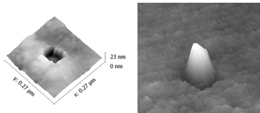
Figure 2.6. AFM images of \text{La}_{0.4}\text{Sr}_{0.4}\text{Ti}_{0.97}\text{Ni}_{0.03}\text{O}_{3-\delta} , showing a strain-induced pit formed during initial \text{Ni}(0) exsolution upon reduction in \text{H}_2 at 600^\circ\text{C} (left), and a “socketed” \text{Ni}(0) nanoparticle after further reduction in \text{H}_2 at 900^\circ\text{C} (right). Reprinted with permission from Journal of Physical Chemistry Letters , Evidence and Model for Strain Driven Release of Metal Nanocatalysts from Perovskites during Exsolution, T-S. Oh et al. Copyright © 2015, American Chemical Society.
