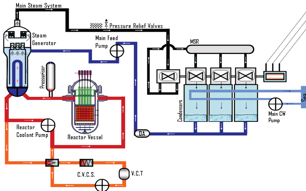
Figure 2. Diagram of a pressurized water reactor (PWR). Source: Nuclear Energy Technology – Knowledge Transfer Workshop, Idaho National Laboratory, Nov. 15-17, 2016.
