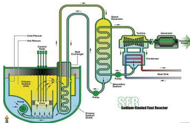
Figure 7. Concept diagram for the Sodium-Cooled Fast Reactor. Gen-IV International Forum, https://www.gen-4.org .
