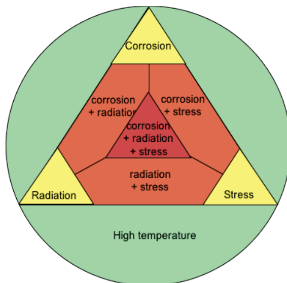
Figure 12. The reactor environment includes four primary components that affect performance of materials; radiation, corrosion, stress and high temperature. Courtesy of Gary Was, University of Michigan.
