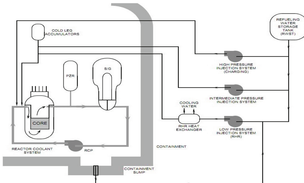
Figure 3. Pressurized water reactor (PWR) high-level layout. Source: Nuclear Energy Technology – Knowledge Transfer Workshop, Idaho National Laboratory, Nov. 15-17, 2016.
