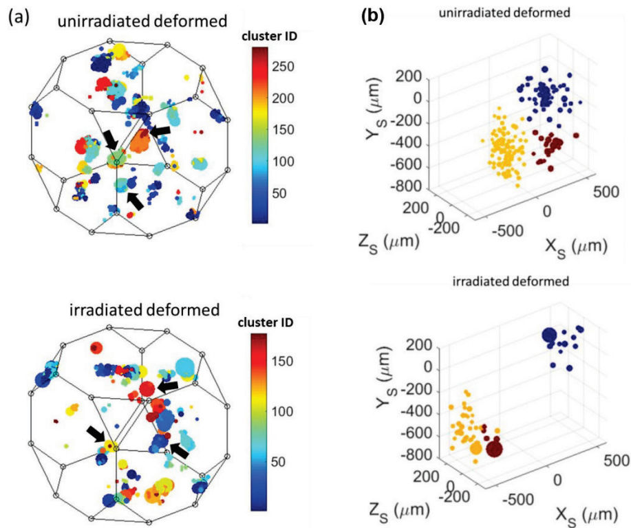
Figure 11. (a) Grain mapping in the Rodrigues-Frank orientation space and (b) maps of three representative subgrains (pointed by arrows in (a)) plotted in the sample coordinates, for the deformed regions of the unirradiated and neutron-irradiated (0.01 dpa/450°C). Image courtesy of Meimei Li, Argonne National Laboratory
