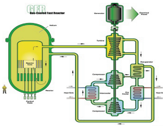
Figure 6. Concept diagram for the Gas-Cooled Fast Reactor. Gen-IV International Forum, https://www.gen-4.org .
