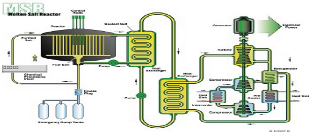
Figure 4. Concept diagram for a liquid-fueled molten salt reactor. Gen-IV International Forum, https://www.gen-4.org .
