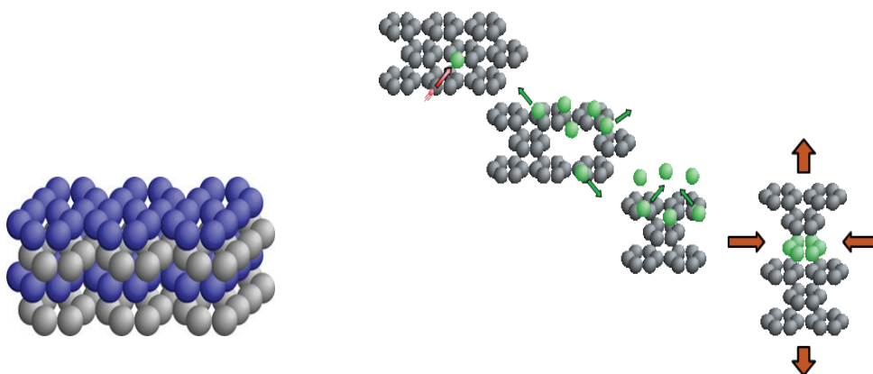
Figure 10. Sub-plane formation and vacancy collapse in irradiated graphitic structures. Assumed to be the underlying mechanisms for irradiation shrinkage (a-axis direction collapse) and growth (c-axis direction expansion) of irradiated nuclear graphite components. Image courtesy of William E. Windes, Idaho National Laboratory
