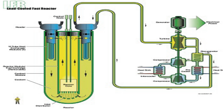
Figure 8. Concept diagram for the Lead-Cooled Fast Reactor. Gen-IV International Forum, https://www.gen-4.org .
