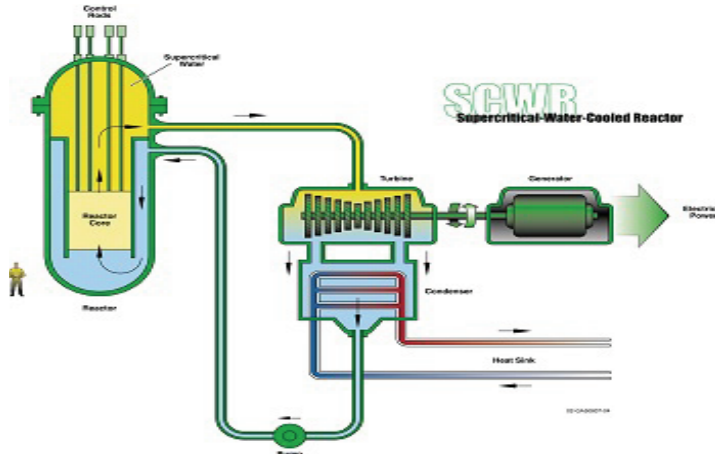
Figure 9. Concept diagram for the Supercritical-Water-Cooled Reactor. Gen-IV International Forum, https://www.gen-4.org .
