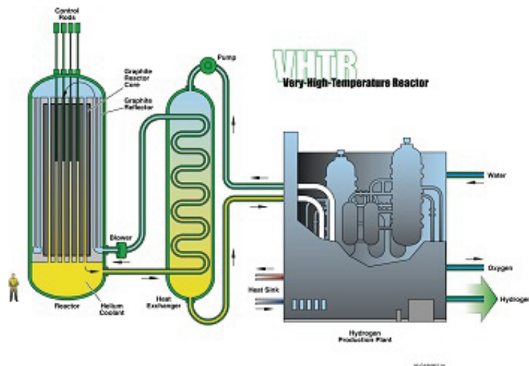
Figure 5. Concept diagram for the Very High Temperature, a Gas-Cooled High-Temperature Reactor. Gen-IV International Forum, https://www.gen-4.org .
