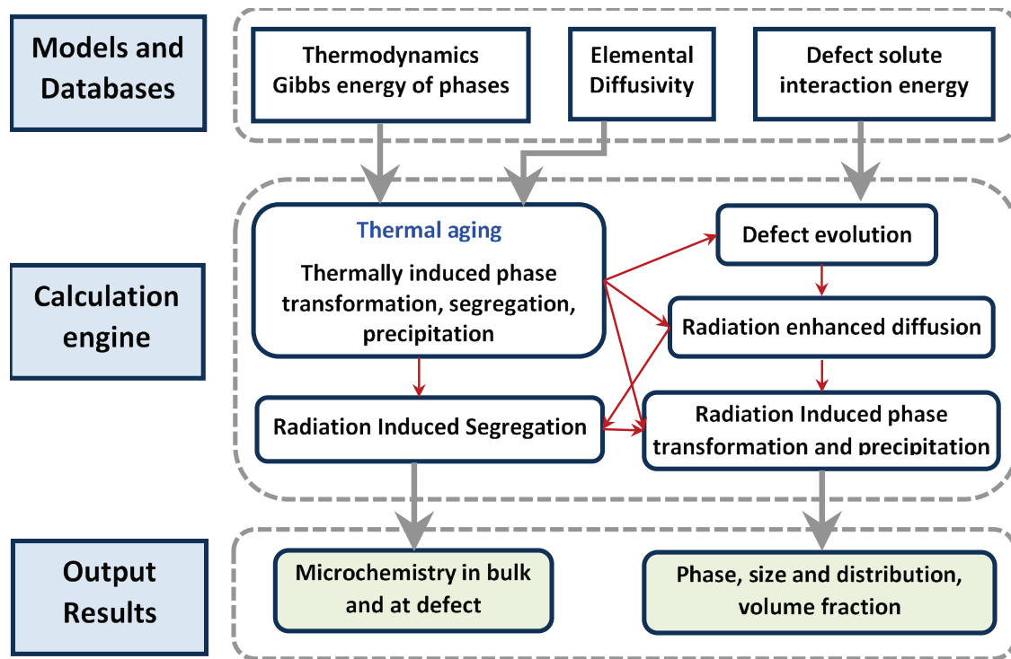
Figure 13. Schematic diagram showing integrated modeling framework on precipitate evolution in irradiated materials. Courtesy of Ying Yang, Oak Ridge National Laboratory.
