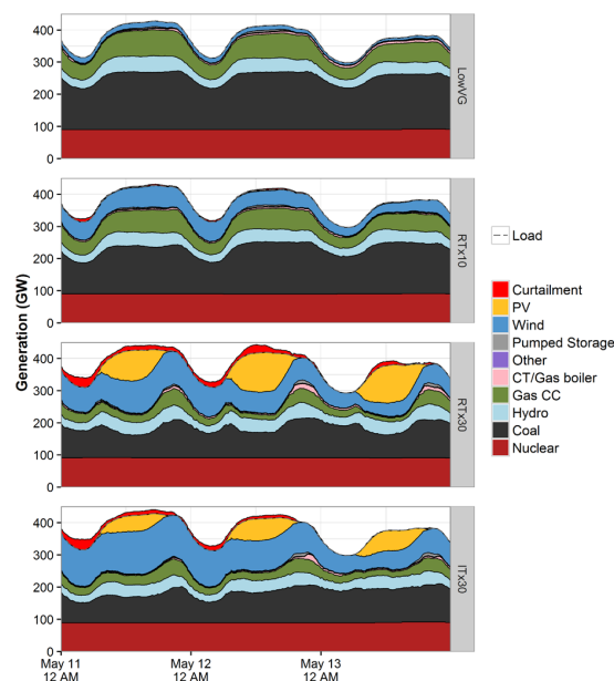
Figure 14. Projected energy dispatch in the eastern interconnect simulated for low (top) to high (bottom) penetrations of variable sources such as photovoltaic and wind. Traditional sources such as gas must ramp up and down two times per day to cope with the daily variation in solar generation. From Bloom et al. (2016). Figure courtesy of National Renewable Energy Laboratory.
