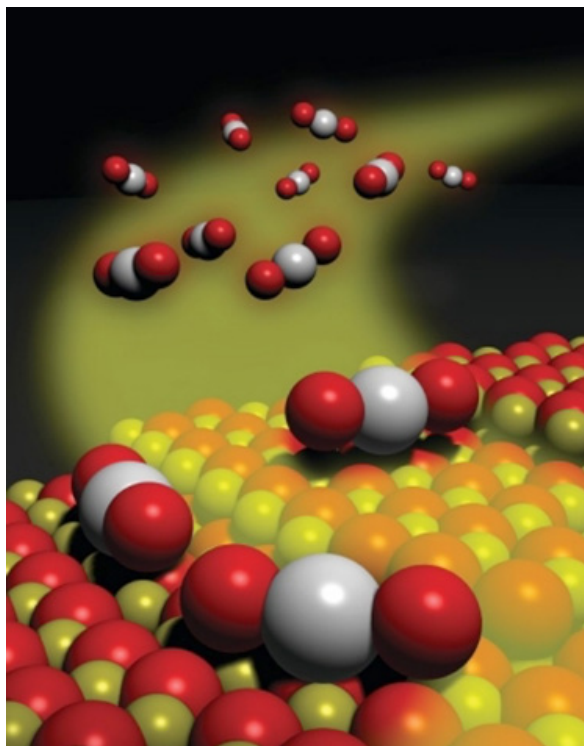
Figure 16. When exposed to high temperature in air, platinum desorbs from Pt nanocrystals as \text{PtO}_2 (grey and red), and can be trapped on \text{CeO}_2 (gold and red). Figure from Jacoby 2016; courtesy of Abhaya Datye (University of New Mexico); artist Cortland Lewis (Pacific Northwest National Laboratory).
