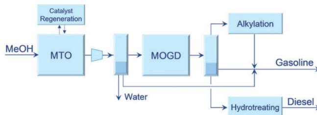
Figure 10. ExxonMobil Olefins to Gasoline and Distillate Process (MOGD). From Olsbye, U., S. Svelle, M. Bjorgen, P. Beato, T. Janssens, F. Joensen, S. Bordiga, and K. Lillerud, Conversion of Methanol to Hydrocarbons: How Zeolite Cavity and Pore Size Controls Product Selectivity, Angewandte Chemie International Edition , 2012, 51: 5810–5831. Copyright Wiley-VCH Verlag GmbH & Co. KGaA. Reproduced with permission.
