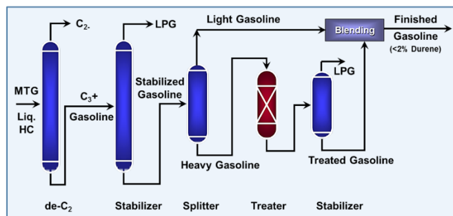
Figure 9. MTG plant design. Image from ExxonMobil "Proven Process. Proven Plants. Proven Performance." Brochure No. L0617-056E49, Courtesy of ExxonMobil (2016).
