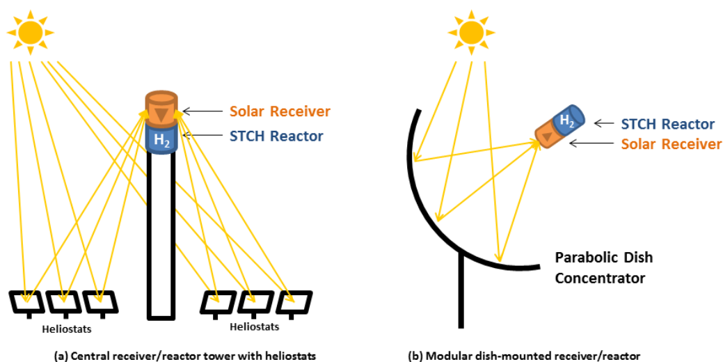
Figure 19. Two mirror-based approaches for focusing sunlight on a solar thermochemical (STCH) reactor to produce temperatures up to 2,000 °C: (a) Field of heliostat mirrors concentrates sunlight onto a central reactor tower, and (b) dish mirrors focus sunlight onto an attached reactor module. Image from U.S. Department of Energy, Office of Energy Efficiency and Renewable Energy (2018).
