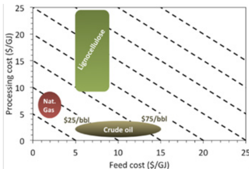
Figure 12. Feed cost vs. processing cost for fuel production from natural gas, crude oil, and lignocellulosic biomass. From Ruddy et al. (2014). Copyright The Royal Society of Chemistry.
