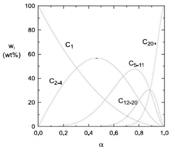
Figure 8. Weight fraction of a hydrocarbon product as a function of chain growth probability ( \alpha ). From James (2012). Reproduced by permission of The Royal Society of Chemistry.
