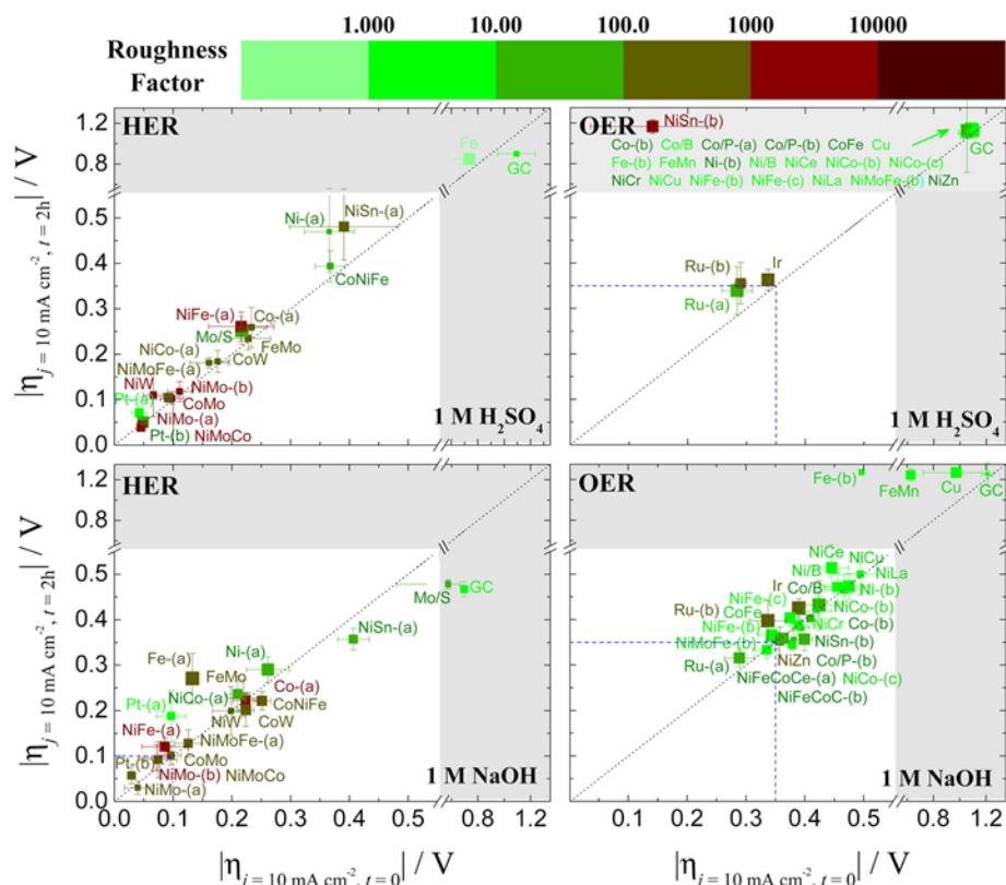
Figure 17. Overpotentials before and after two-hour continuous testing of HER and OER catalysts in aqueous base (pH 14) or acid (pH 0). Reprinted with permission from Journal of the American Chemical Society , Benchmarking Hydrogen Evolving Reaction and Oxygen Evolving Reaction Electrocatalysts for Solar Water Splitting Devices, McCrory et al. (2015). Copyright © 2015, American Chemical Society.
