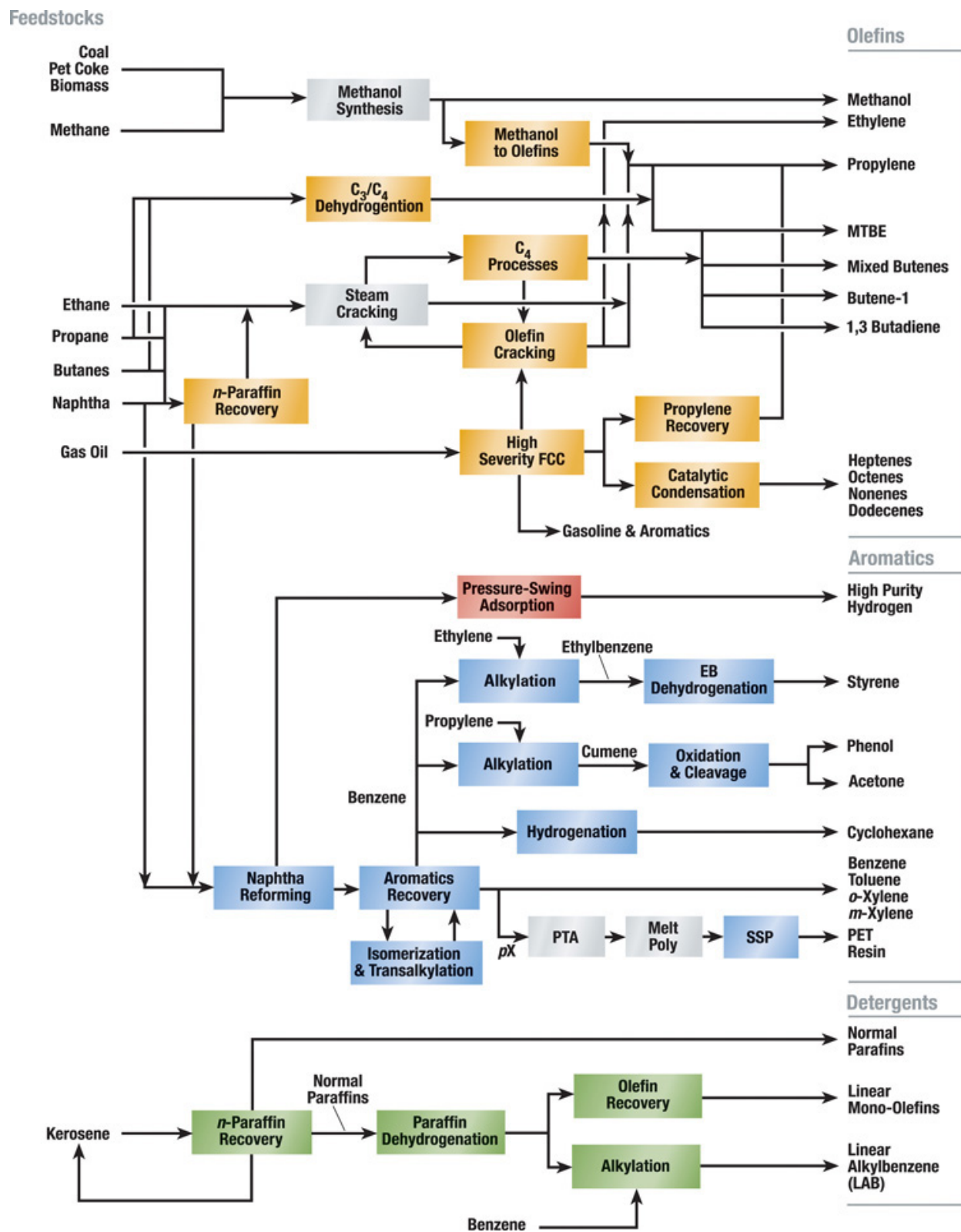
Figure 3. Varieties of feedstock, catalysts, and processes in the production of chemicals. From Honeywell UOP, "Petrochemicals Flow Scheme" (Honeywell UOP 2018a), Courtesy of Honeywell UOP.
