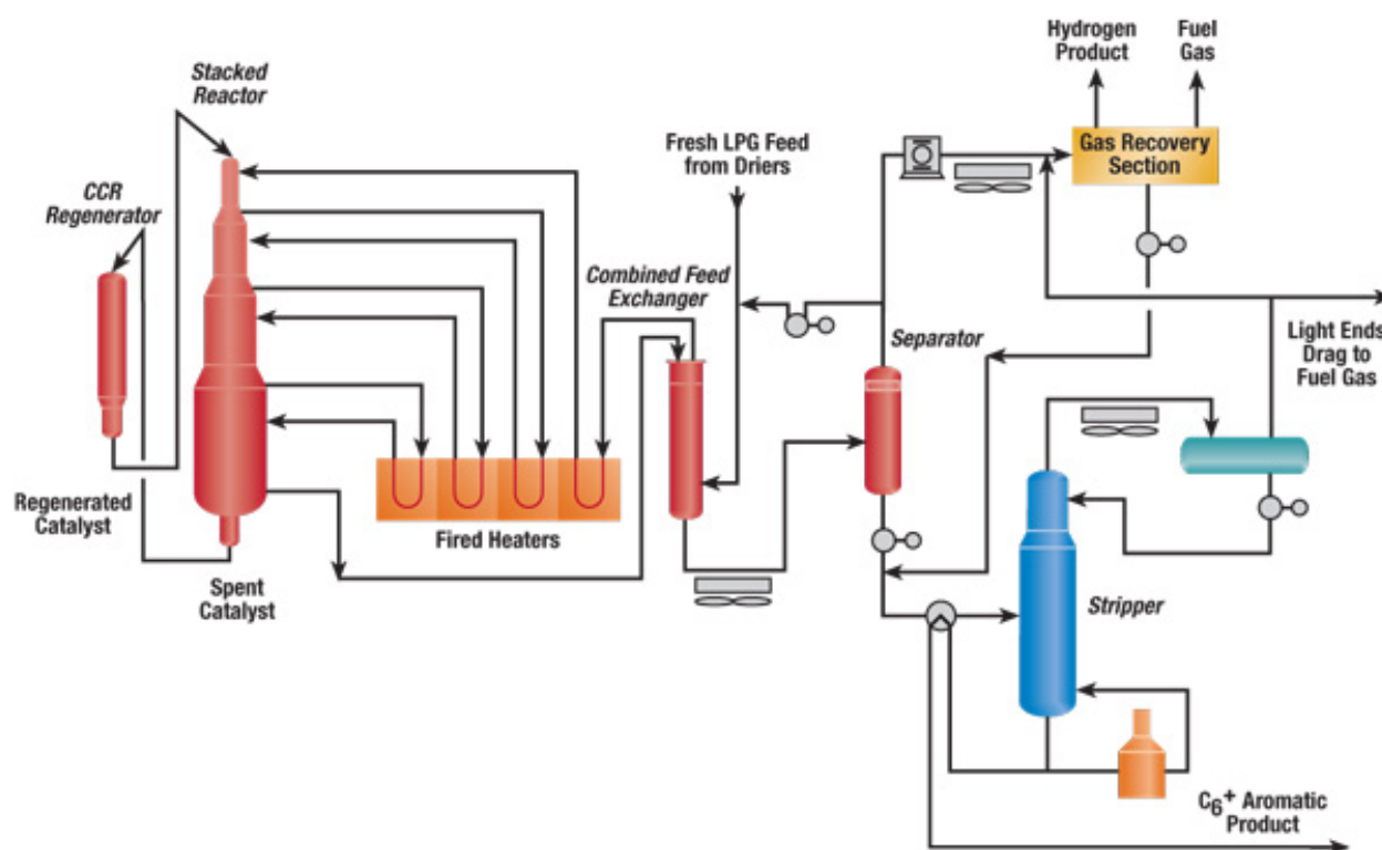
Figure 6. Honeywell UOP's Cyclar™ process layout. From Foley, "CYCLAR™ Process Produces High-Quality Aromatic Products" (Foley 2013). Courtesy of Honeywell UOP.
