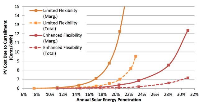
Figure 15. Projected cost of PV electricity as a function of average annual solar penetration. Curtailment, depending on the flexibility of the grid, increases the cost of solar electrons considerably. From Denholm et al. (2016). Figure courtesy of National Renewable Energy Laboratory.
