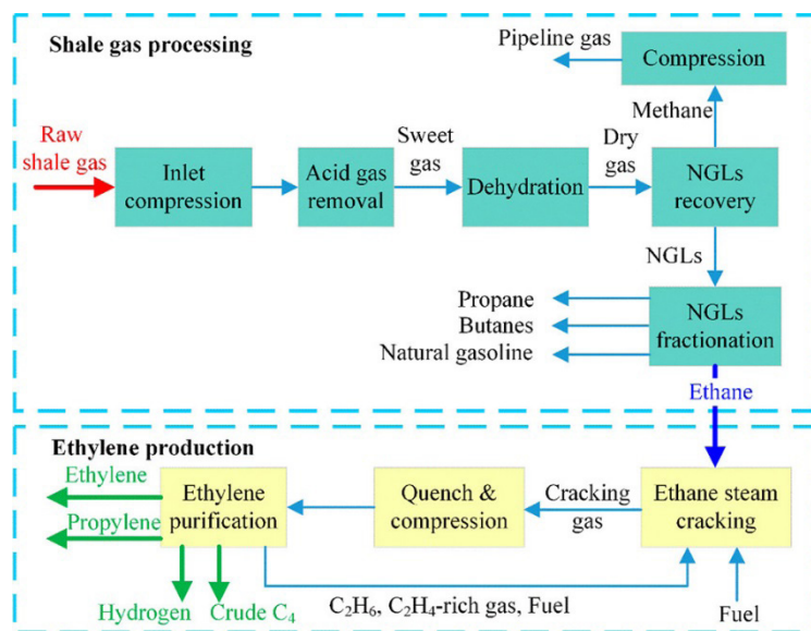
Figure 7. Flow diagram for manufacturing ethylene from ethane-rich natural gas. Reprinted with permission from Industrial & Engineering Chemistry Research, Manufacturing Ethylene from Wet Shale Gas and Biomass: Comparative Technoeconomic Analysis and Environmental Life Cycle Assessment, Yang et al. Copyright © 2018, American Chemical Society.
