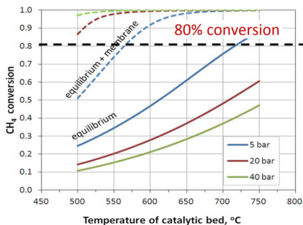
Figure 22. Predicted CH 4 conversion achieved for SMR as a function of temperature and pressure with and without a H 2 membrane. From Saric (2015). Reproduced with permission.
