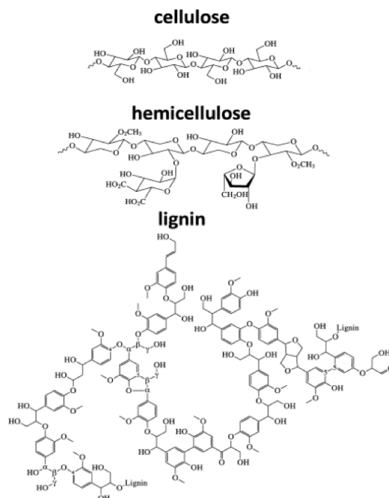
Figure 11. Polymeric structures of cellulose, hemicellulose, and lignin.
