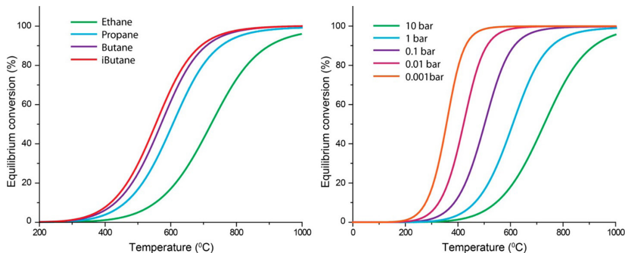
Figure 4. Equilibrium conversion of C2–C4 light alkanes to olefins as a function of temperature at 1 bar (left), and pressure dependence of the dehydrogenation of propane as a function of temperature (right). Reprinted with permission from Chemical Reviews , Catalytic Dehydrogenation of Light Alkanes on Metals and Metal Oxides, Sattler et al. Copyright © 2014, American Chemical Society.
