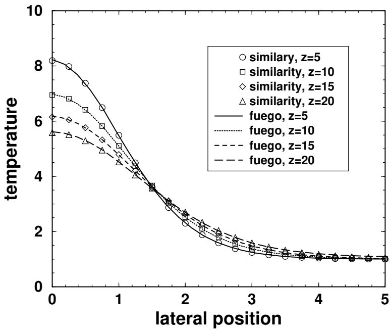
Figure 3.7-13.. Lateral profiles of temperature for the laminar, buoyant plume. Temperature equation with Pr=2 , Re=16.7 , Ra=85000 .
