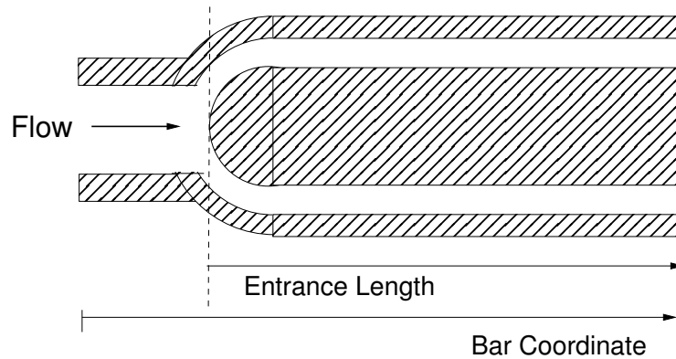
Figure 33.12-2.. Flow Entrance Effect Coordinate
