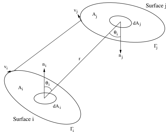
Figure 22.5-6.. View Factor Configuration
