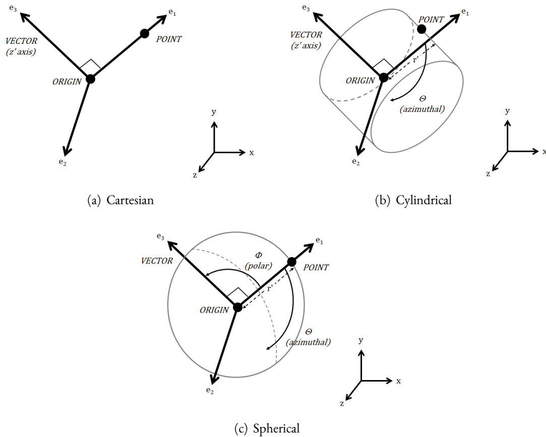
Figure 30.1-1.. A depiction of the available local coordinate system options and how they are constructed given ORIGIN, VECTOR, and POINT.
