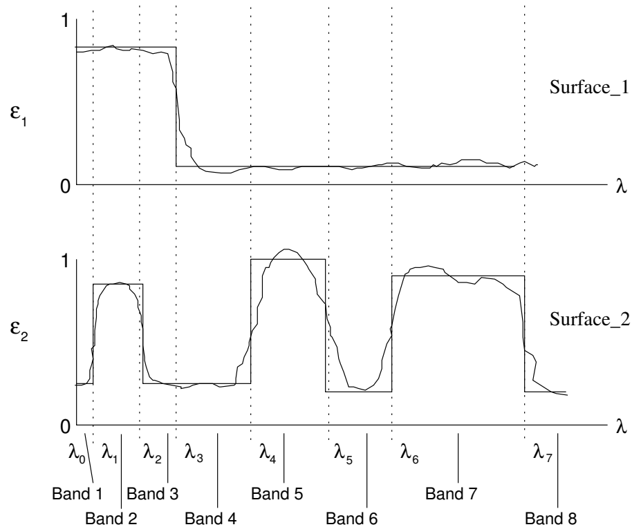
Figure 22.4-1.. Emissivity Bands For Two-Surface Problem
