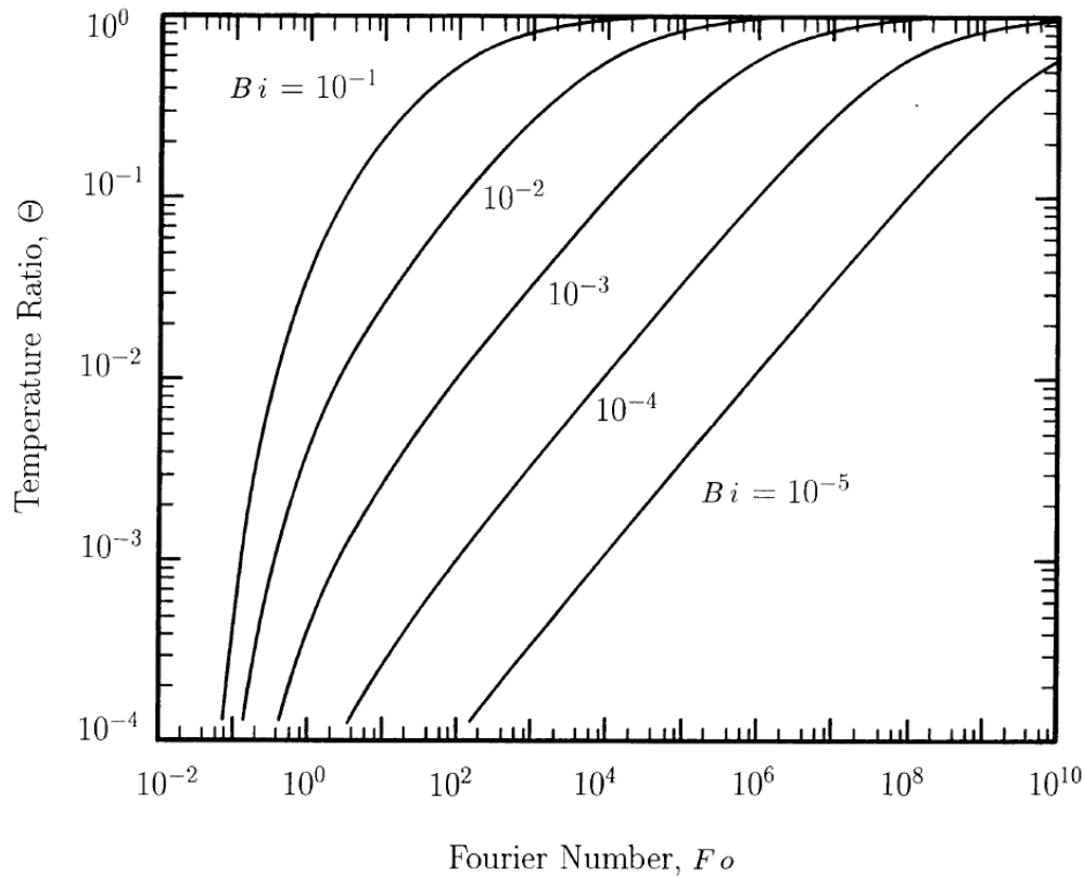
Figure 16.2-3.. Temperature ratio versus Fourier number for various Biot numbers.
