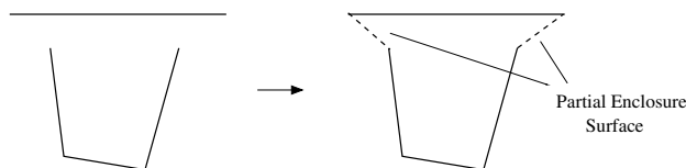
Figure 22.5-2.. Discretization and Associated Partial Enclosure Surface.
