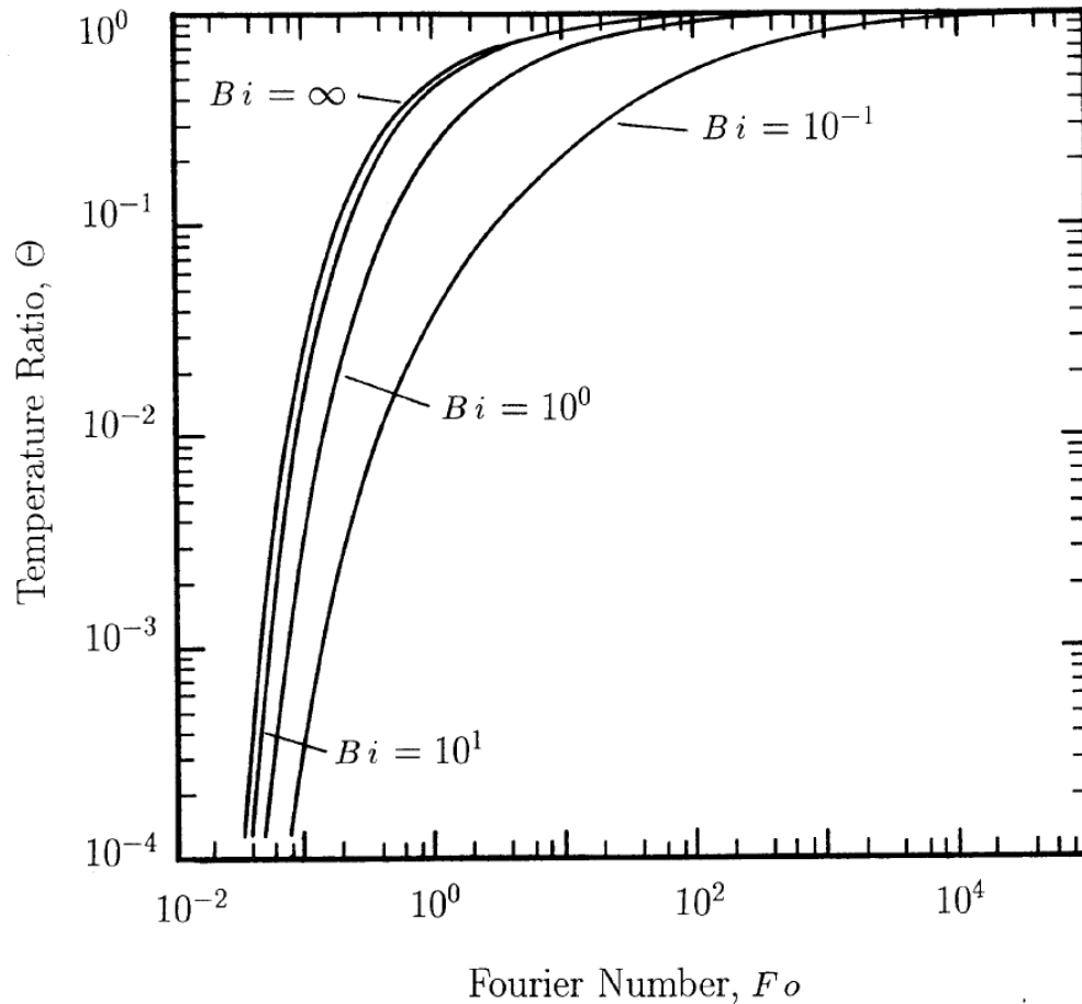
Figure 16.2-2.. Temperature ratio versus Fourier number for various Biot numbers.
