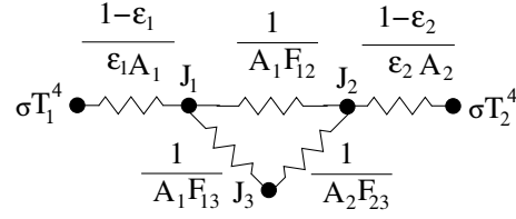
Figure 22.5-9.. Three Surface Network Model ( \varepsilon_3 = 0 and \varepsilon_3 = 1 )
