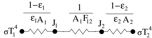
Figure 22.5-5.. Two Surface Network Model
