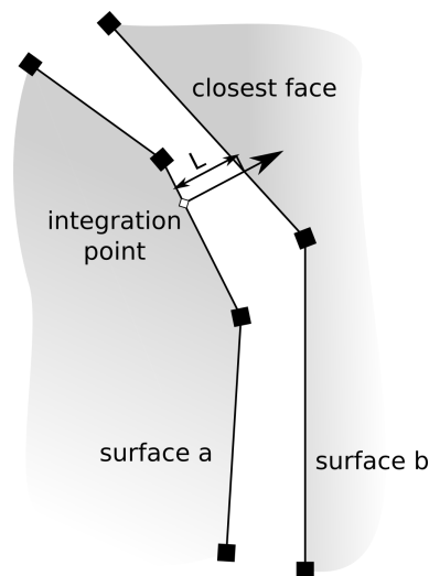
Figure 24.1-1.. Calculation of contact distance per integration point.
