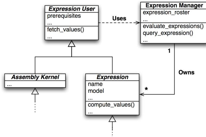
Figure 44.2-1.. Schematic UML class diagram for the Expression subsystem.
