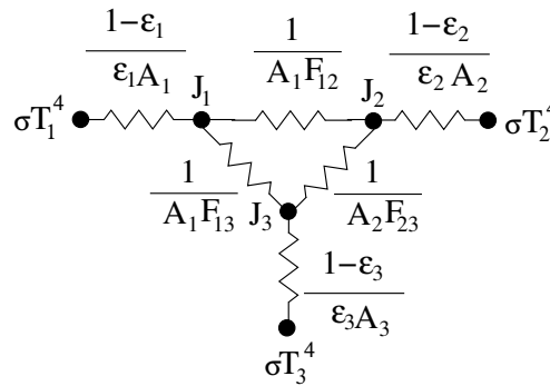
Figure 22.5-8.. Three Surface Network Model
