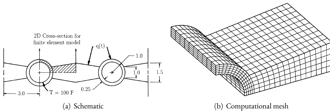
Figure 16.2-1.. Geometry and mesh of finned radiator problem. Dimensions are in inches.
