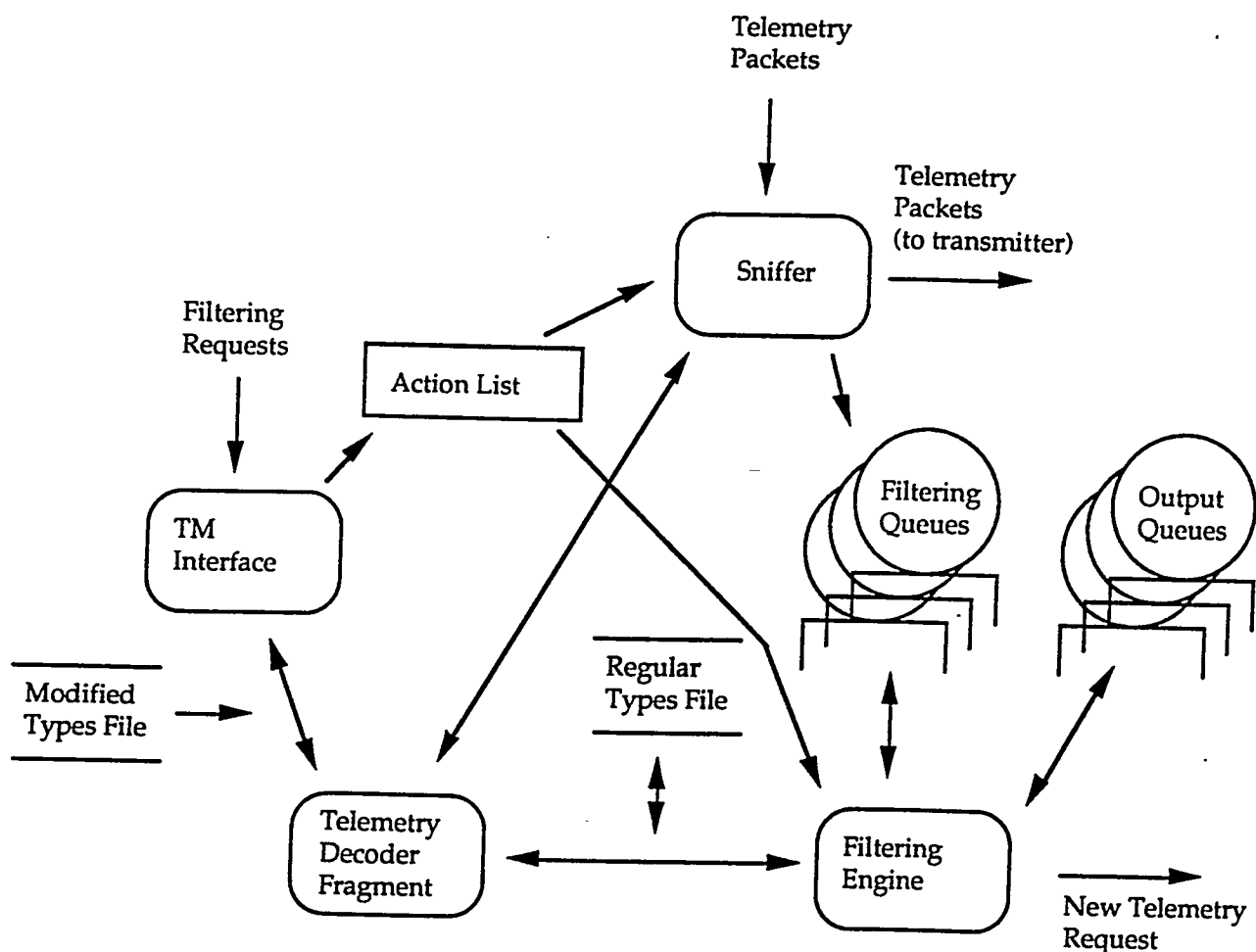
Figure 5. Elements of a Telemetry Monitor.
