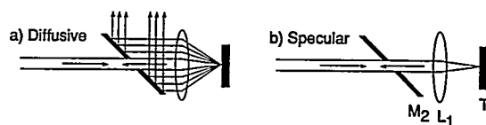
Figure 5. Hole vignetting when mirror ( M_2 ) is close to lens ( L_1 ) of target (T). a) For a diffusively scattering target the vignetting is not substantial and is roughly independent of target position. b) For a specularly reflective target oriented normal to the illuminating beam the vignetting is complete when the target is at the focal point of the lens. An astigmatic lens would not significantly reduce hole vignetting when the mirror is close to the lens.
