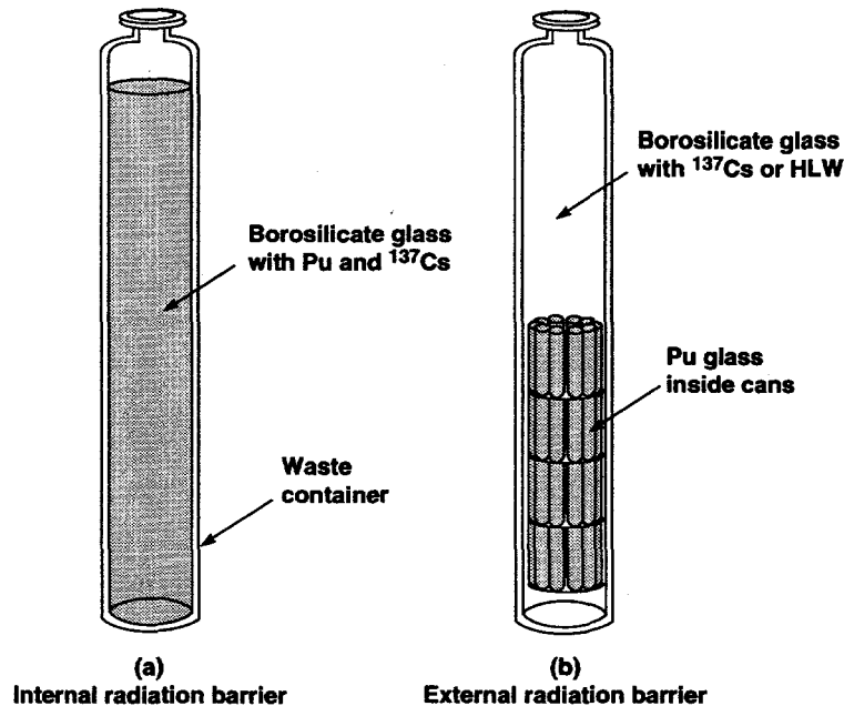
Figure 3. Two options for vitrification of Pu.
