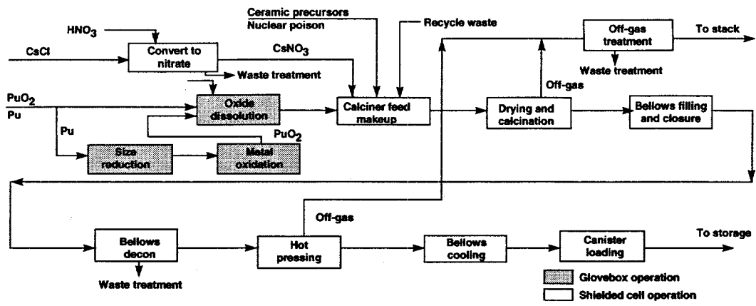
Figure 6. Ceramic immobilization block flow diagram
