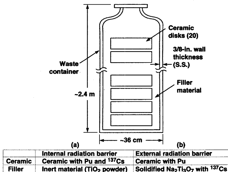
Figure 4. Two options for immobilizing Pu in a ceramic.
