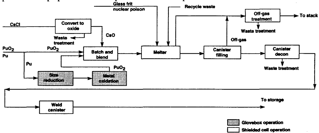
Figure 5. Vitrification block flow diagram.
