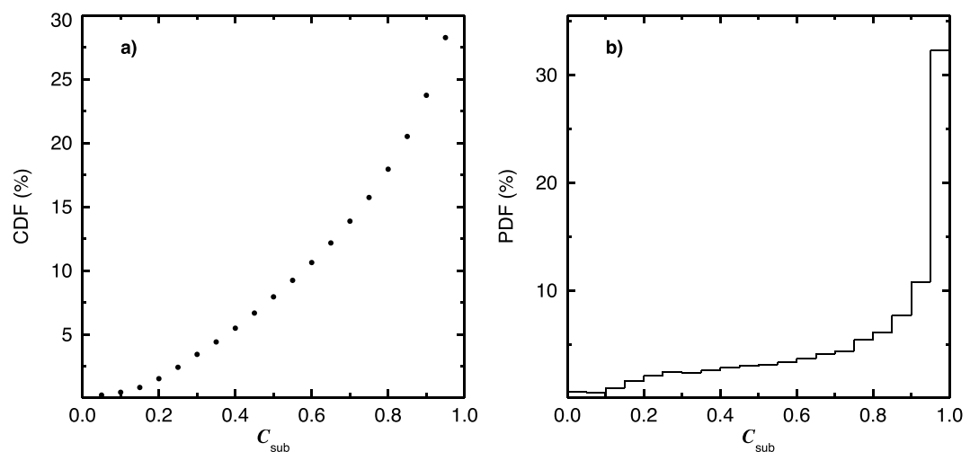
Figure 2. (a) Cumulative density function (CDF) of C_{sub} for all cloudy pixels (for visibility reasons the last data point at 100% is not shown). Data are from 48 altocumulus and broken cumulus scenes sampled off the coast of California. The horizontal resolution at the pixel level is 960 m. (b) Probability density function (PDF) of C_{sub} for all partially cloudy pixels.
