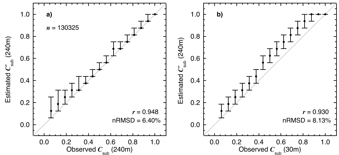
Figure 6. (a) Comparison between the actually observed subpixel cloud cover ( C_{sub} ; based on the extensive cloud masking scheme described in section 2) derived from 240-m data and the estimated results ( C_{sub}^* ; based on equation (2)). The pixel level scale is 960 m. The number of observations ( n ), correlation coefficient r , and normalized root-mean-square deviation between the C_{sub} and C_{sub}^* (nRMSD) is given. (b) Same as (a) but C_{sub} is derived from observations at a horizontal resolution of 30 m.
