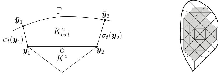
Figure 3: Left: A boundary edge e with corresponding element K^e and region K^e_{ext} . Right: \Omega^h_{ext} := \cup_{e \in \mathcal{E}_h^\partial} K^e_{ext} (white region).
