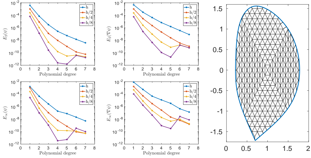
Figure 6: Convergence plots for Example 3 (NSTX) for successive refinements of the computational grid and increasingly higher polynomialonclusion degrees. Left column: E_2 (top) and E_\infty (bottom) errors for the poloidal flux \psi . Center column: E_2 (top) and E_\infty (bottom) errors for \nabla\psi . Right column: Confinement region and sample grid corresponding to the second level of refinement (red curve in the convergence plot). The reader is referred to the on-line version of the manuscript for the color scheme.
