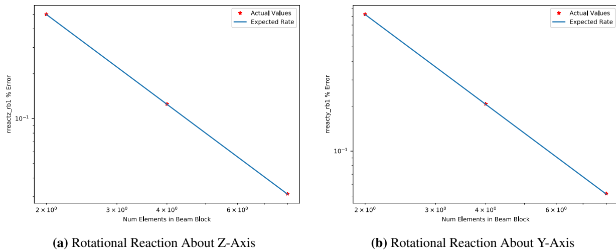
Figure 3-49. Reaction Load Convergence
