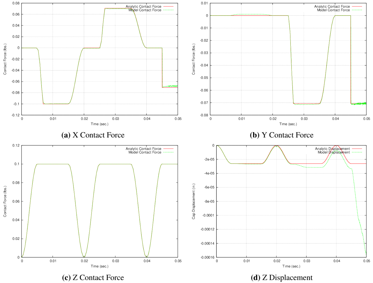
Figure 2-34. Static Kinematic
