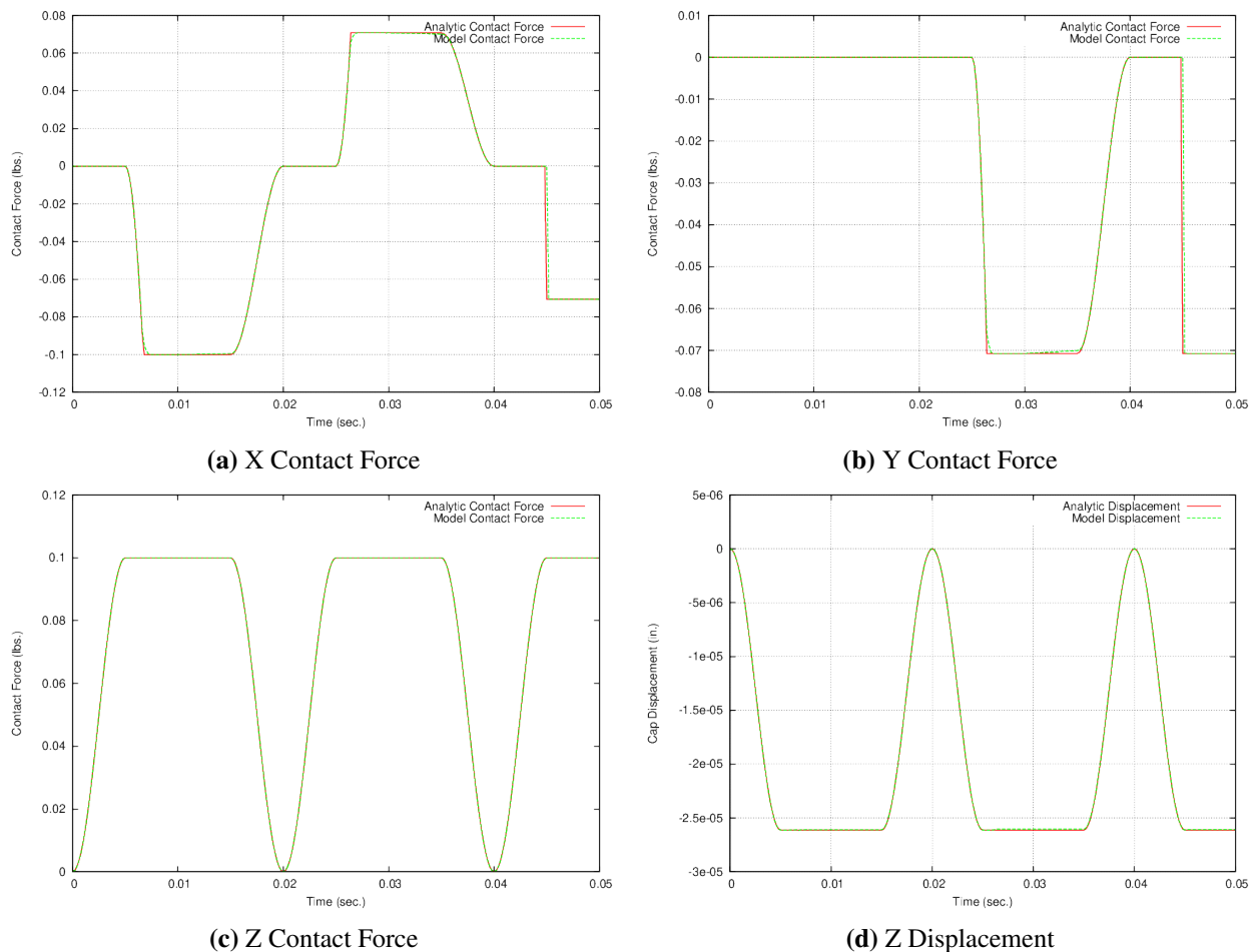
Figure 2-31. Static Node-Face
