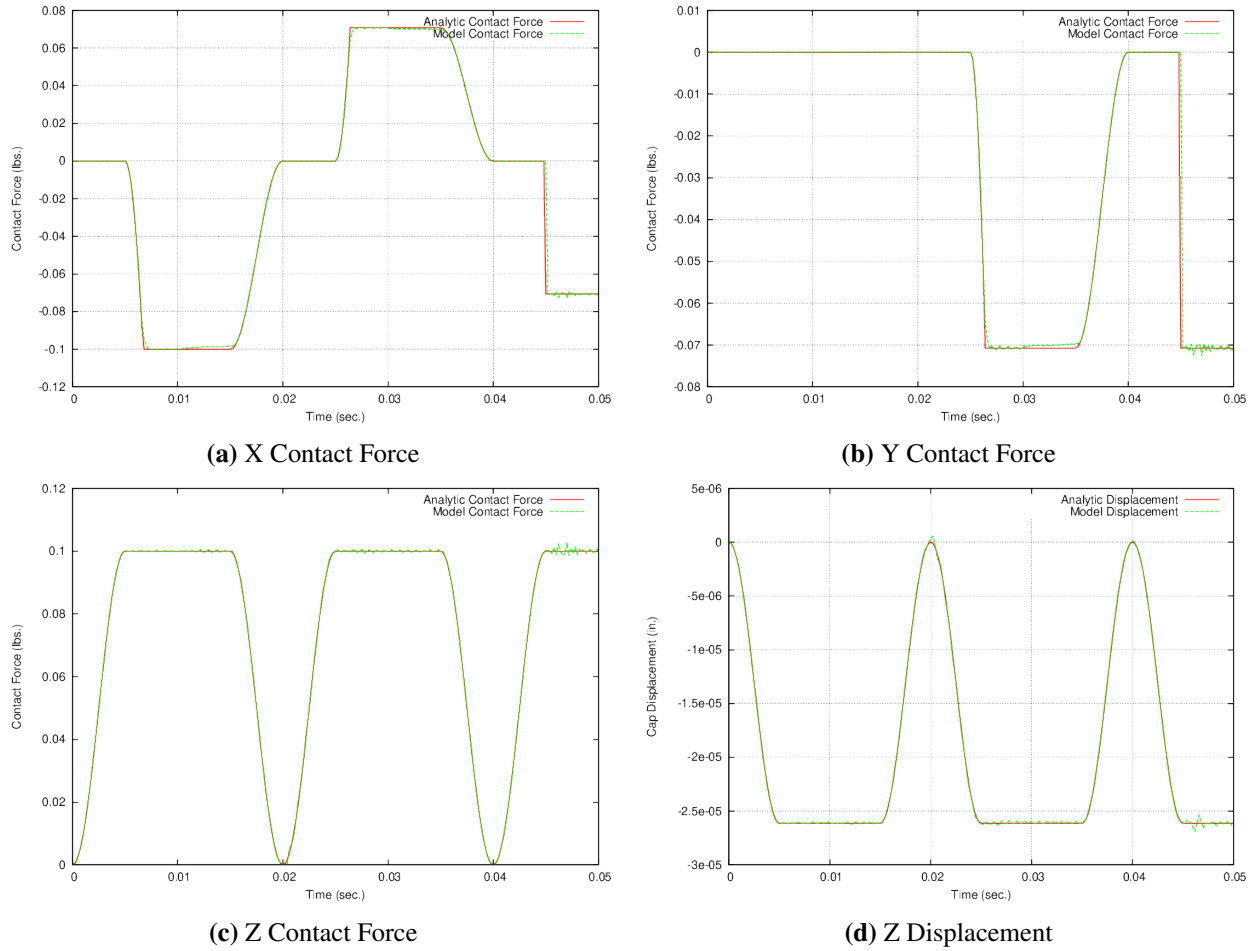
Figure 2-35. Implicit Dynamics Node-Face
