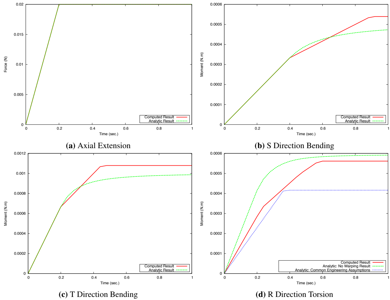
Figure 3-44. Bar Section
