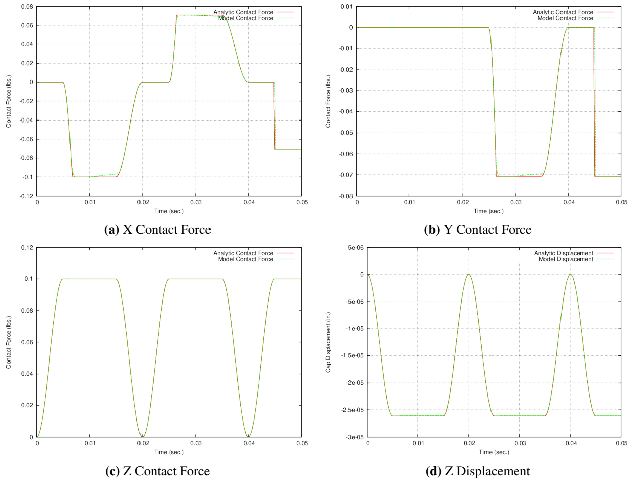
Figure 2-32. Static Face-Face
