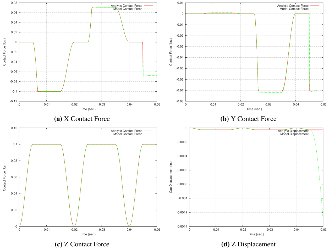
Figure 2-33. Static ARS
