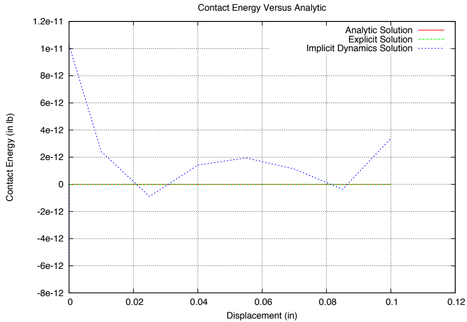
Figure 4-2. Energy-Displacement curve
