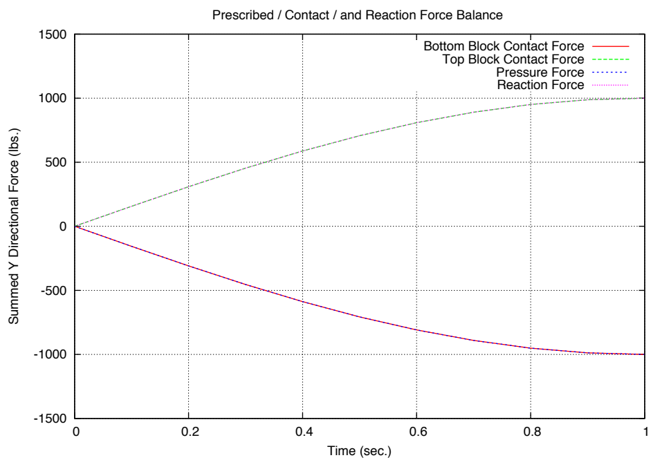
Figure 2-1. Force Balance
