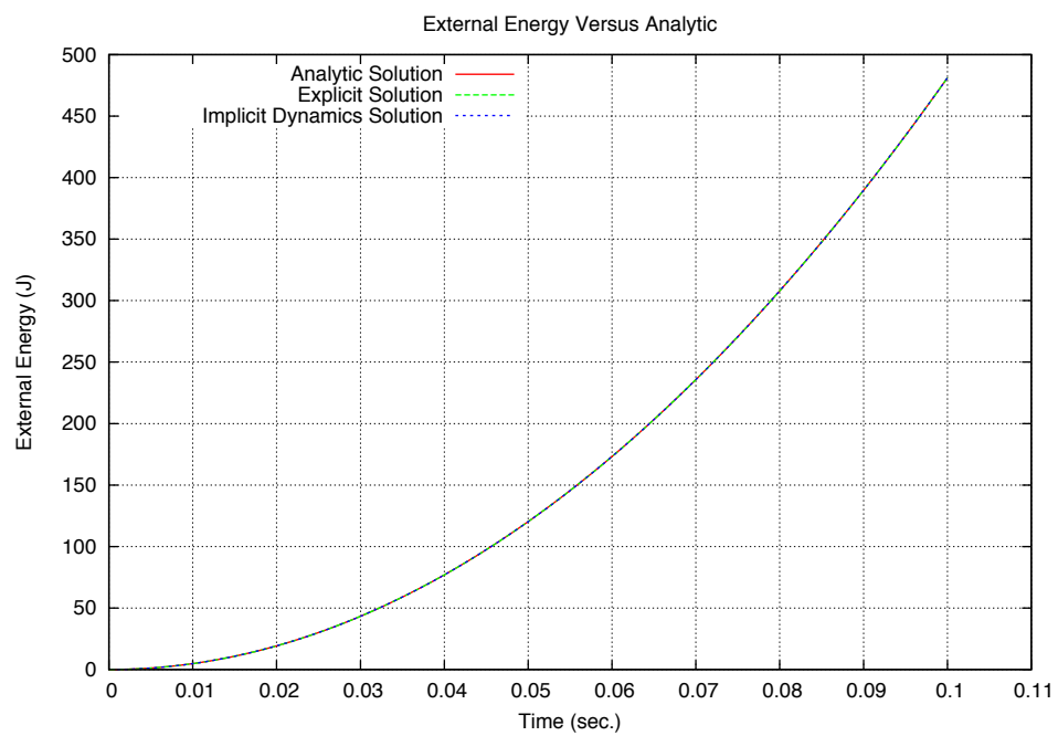
Figure 4-3. Energy-time curve
