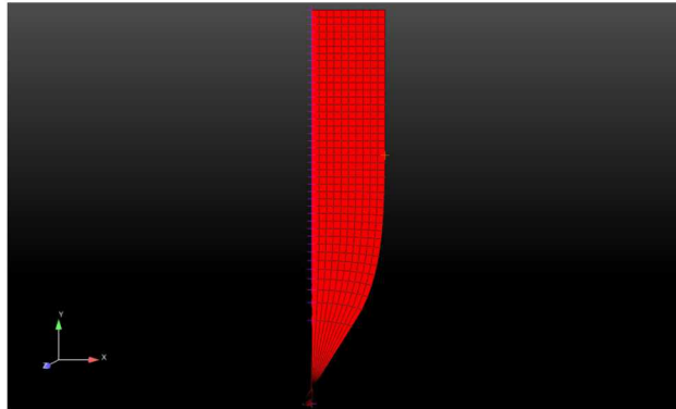
Figure 3-26. Mesh after stretching without remeshing
