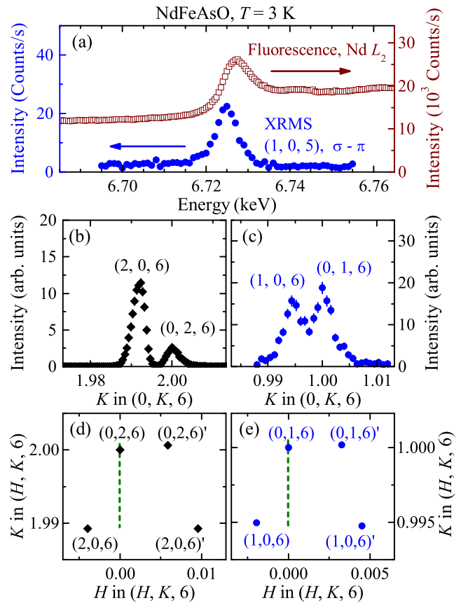
FIG. 1. (Color online) (a) Energy scans through the (1, 0, 5) magnetic Bragg peak (filled circles) in the \sigma - \pi scattering geometry at T = 3 \text{ K} and the measured fluorescence (open squares) under the same experimental conditions without a polarization analyzer. (b) [0, K, 0] scan through the structural Bragg position at T = 3 \text{ K} . (c) [0, K, 0] scan through the magnetic Bragg position at T = 3 \text{ K} . (d) and (e) plot of the structural and magnetic peak positions in the H and K planes, respectively. The dashed lines indicate the scan path in (b) and (c).
