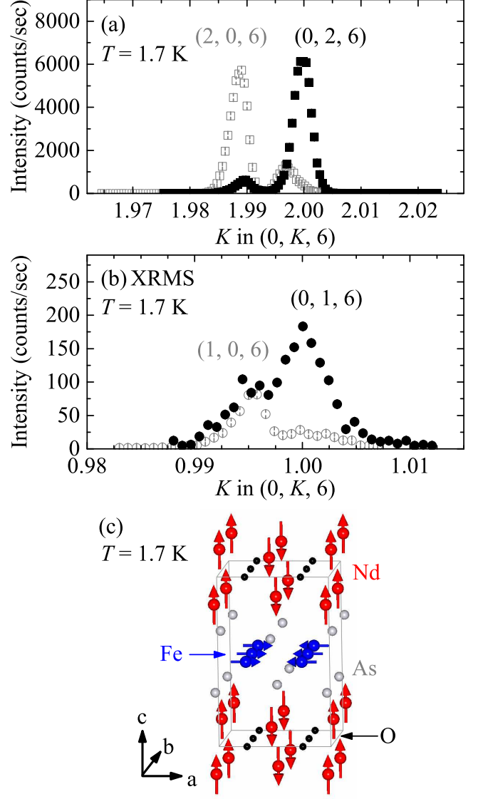
FIG. 2. (Color online) Distribution of (a) structural Bragg peaks measured along [0, K, 0] after the alignment is optimized for \mathbf{Q} = (2, 0, 6) (open squares) and for (0, 2, 6) (filled squares), respectively and (b) magnetic Bragg peaks measured along [0, K, 0] after the alignment is optimized for \mathbf{Q} = (1, 0, 6) (open circles) and for (0, 1, 6) (filled circles), respectively. (c) Proposed magnetic structure at T = 1.7 K.
