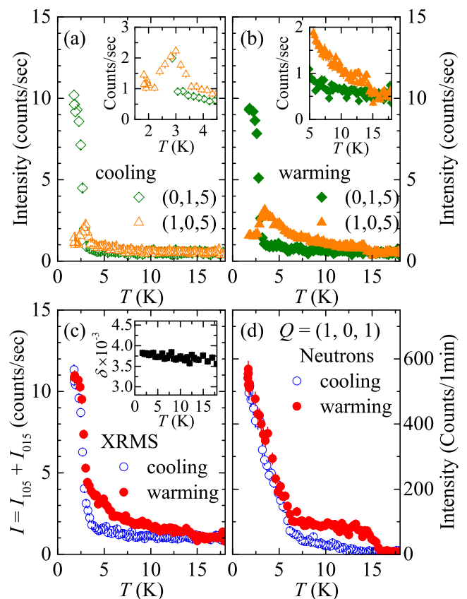
FIG. 3. (Color online) Temperature dependence of the magnetic order parameters of the magnetic (1, 0, 5) (triangles) and (0, 1, 5) (diamonds) Bragg peaks during (a) cooling (open symbols) and (b) warming (filled symbols). Insets in panel (a) and (b) show the temperature range between 1.7 K and 5 K and between 5 K and 18 K, respectively. (c) Total scattering intensity by sum of intensities of (1, 0, 5) and (0, 1, 5) Bragg peaks during cooling (open circles) and warming (filled circles). Inset shows the orthorhombicity \delta = (a - b)/(a + b) in the same temperature range. (d) The magnetic order parameter at Q = (1, 0, 1) from our previous neutron diffraction measurement 15 during cooling (open circles) and warming (filled circles).
