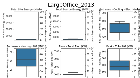
Figure 10: Box-whisker plot of energy performance index for the large office at the 2013 vintage.
