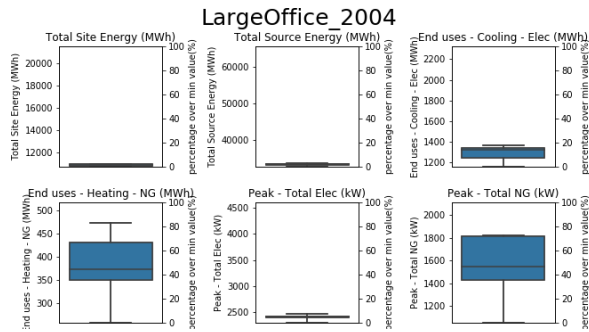
Figure 9: Box-whisker plot of energy performance index for the large office at the 2004 vintage.
