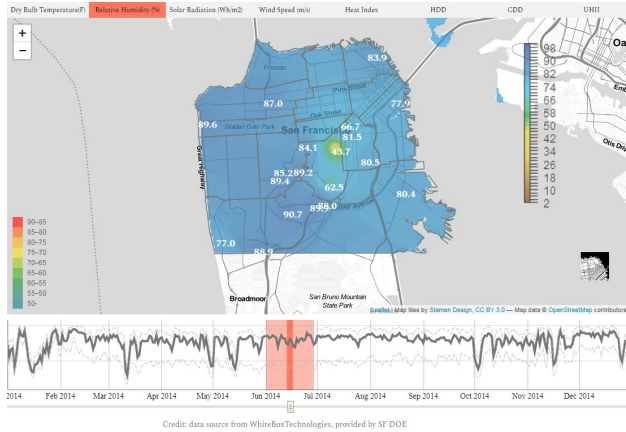
Figure 6: Spatial heterogeneity of relative humidity
