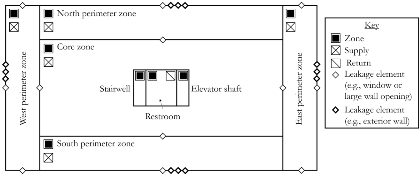
Figure 1 CONTAM model of a medium office building (icons enlarged for clarity)
