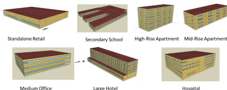
Figure 2. Renderings of the seven commercial prototype building models available in the calculator.
