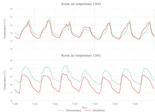
Figure 10: Room air temperature comparison for test 1 (upper: best case, lower: worse case)
