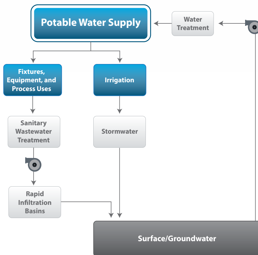
Figure 2. Net Zero Water Concept
