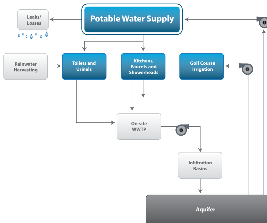
Figure 4.2 Fort Buchanan's Proposed Net Zero Water Concept
