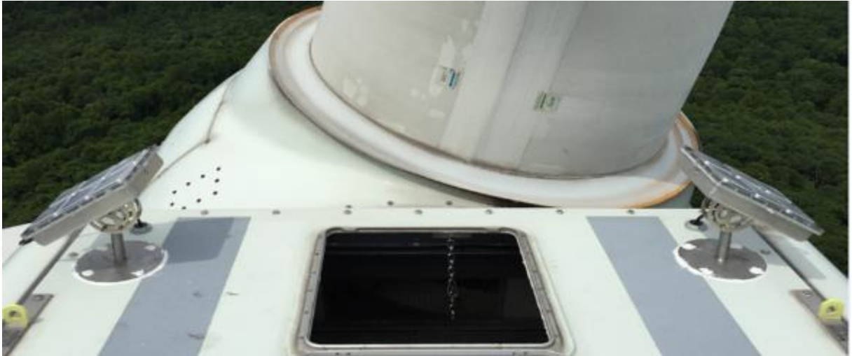
Figure 8. Photograph of two prototype UADs on the top of the nacelle, positioned near the rotor.
