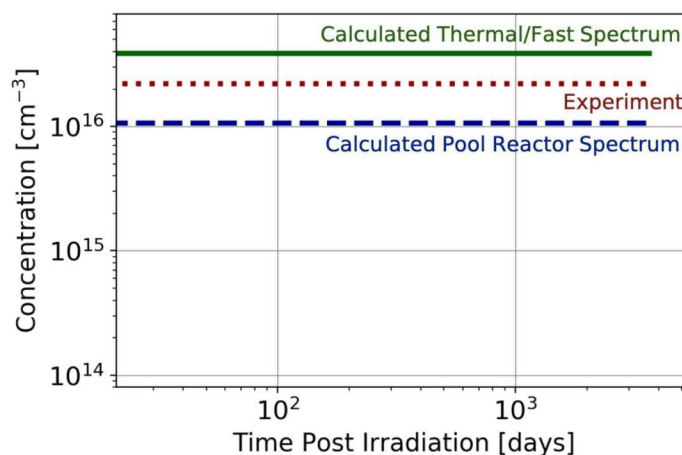
Fig. 2 Comparison between experimentally observed 26 and computed Ge concentration resulting from GaN neutron irradiation with thermal and fast neutron fluence of 1.5 \times 10^{17} neutrons/cm 2 for pure thermal and pure fast neutron spectra and for a similar thermal pool-type light water reactor as was used for experimental irradiation. Concentrations are shown starting at 3 weeks post-irradiation, as this was when the experiment was performed.
