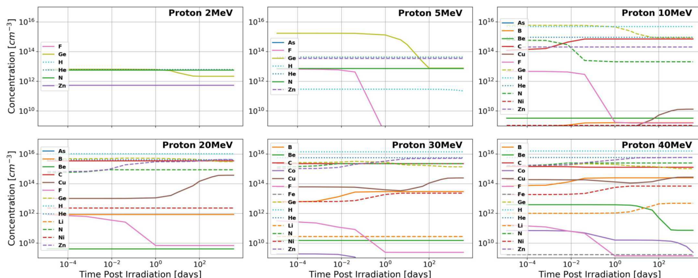
Fig. 5 Total concentrations of impurity elements introduced in \text{Ga}_2\text{O}_3 as a function of time following quasi-monoenergetic 2, 5, 10, 20, 30, and 40 MeV proton irradiation. Substantial dopants of note include Ge, N, and Zn for most proton energies ( E_p ), with the inclusion of C for E_p \geq 10 MeV, Cu and Ni for E_p \geq 20 MeV, B for E_p \geq 30 MeV, and Li for E_p \geq 40 MeV. All results are shown in tabular format in the Supplementary Material †.
