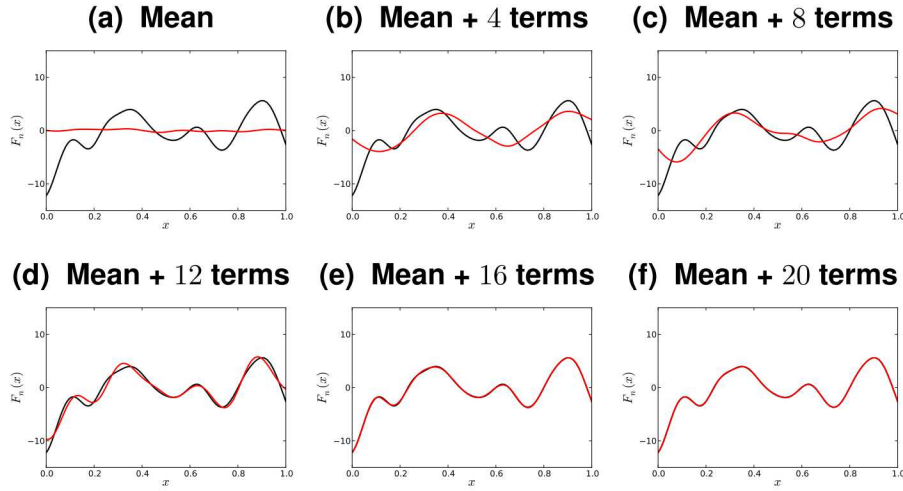
Figure 5-37. Reconstructing realizations with an increasing number of KL expansion terms for c_l = 0.10
