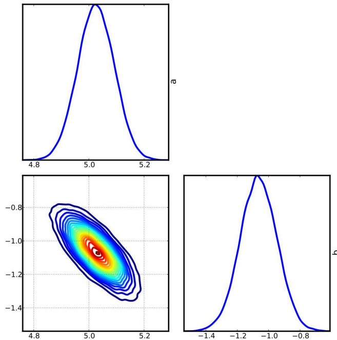
Figure 5-22. Marginal posterior distributions for all variables, as well as marginal joint posteriors
