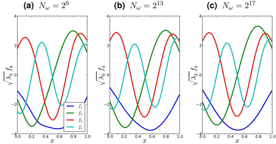
Figure 5-33. Illustration of first 4 KL modes, computed based on a numerical covariance matrices using three sets of RF realizations with c_l = 0.20
