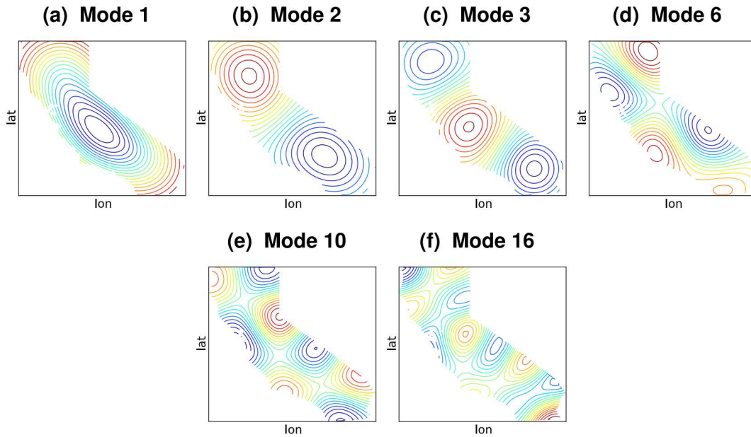
Figure 5-49. Illustration of select KL modes, computed based on a numerical covariance matrix estimated using 2^{16} 2D RF realizations on an unstructured grid with c_l = 2^\circ .
