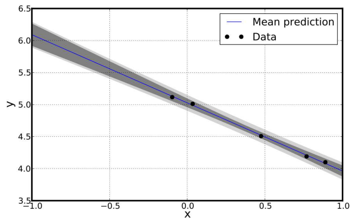
Figure 5-20. The pushed forward posterior distribution (dark grey) and posterior predictive distribution (light grey).
