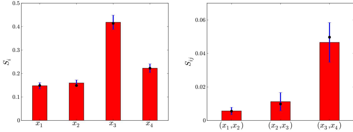
Figure 5-27. First-order (left frame) and joint (right frame) Sobol indices for the model given in Eq. (5.35). The black circles show the theoretical values, computed analytically, and the error bars correspond to \pm\sigma computed based on an ensemble of 10 runs.
