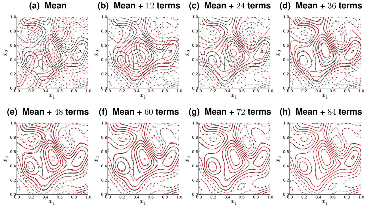
Figure 5-43. Reconstructing 2D realizations with an increasing number of KL expansion terms for c_l = 0.2
