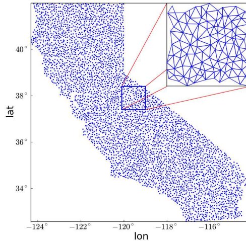
Figure 5-45. Unstructured grid generated via Delaunay triangulation overlaid over California.
