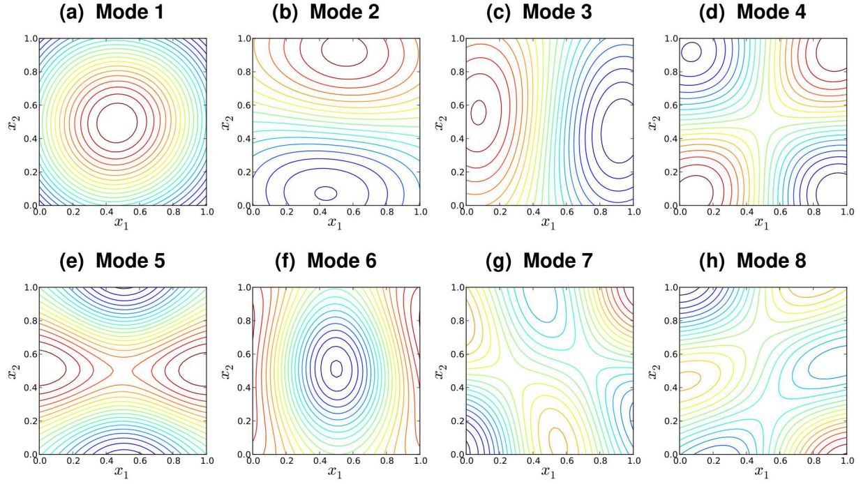
Figure 5-42. Illustration of first 8 KL modes, computed based on a numerical covariance matrix estimated using 2^{12} 2D RF realizations with c_l = 0.5
