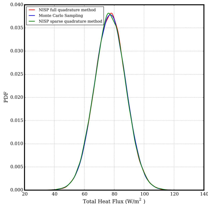
Figure 5-13. Sample results of rad_heat_transfer_atm_pce.py with nord = 2
