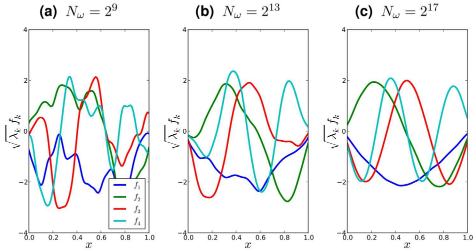
Figure 5-32. Illustration of first 4 KL modes, computed based on a numerical covariance matrices using three sets of RF realizations with c_l = 0.05
