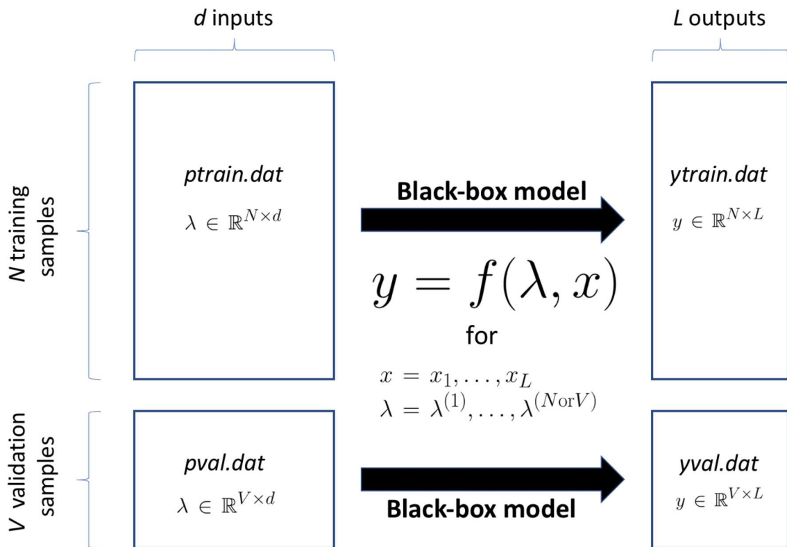
Figure 5-26. Sketch of the expected input-output structure of the black-box model.
