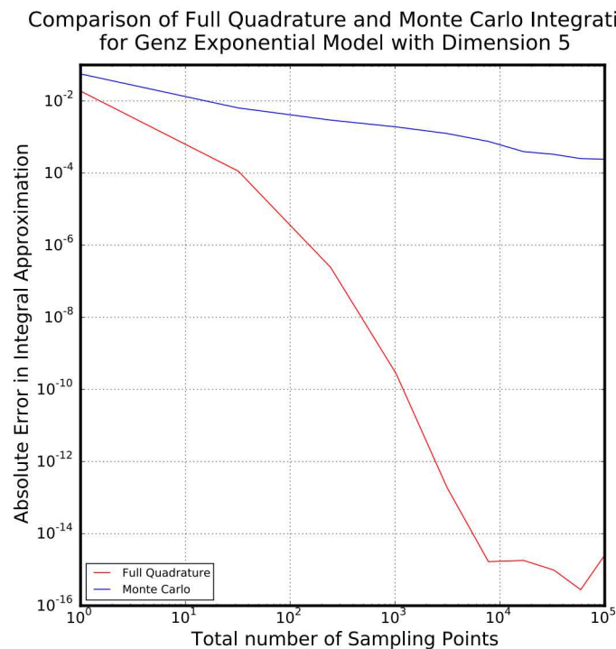
Figure 5-9. Sample results of full_quad.py
