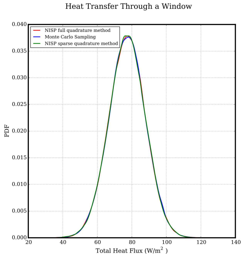
Figure 5-12. Sample results of rad_heat_transfer_atm_pce.py
