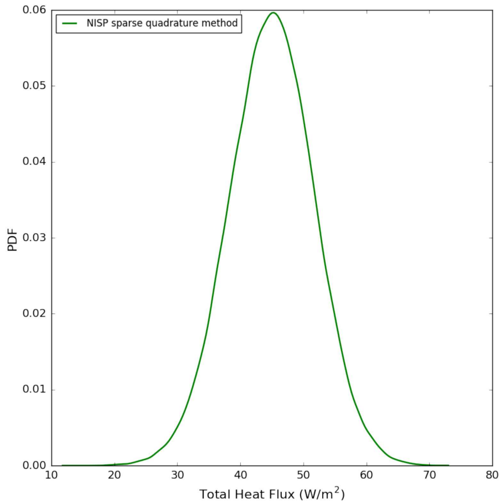
Figure 5-15. Sample results of highd_sparse.py
