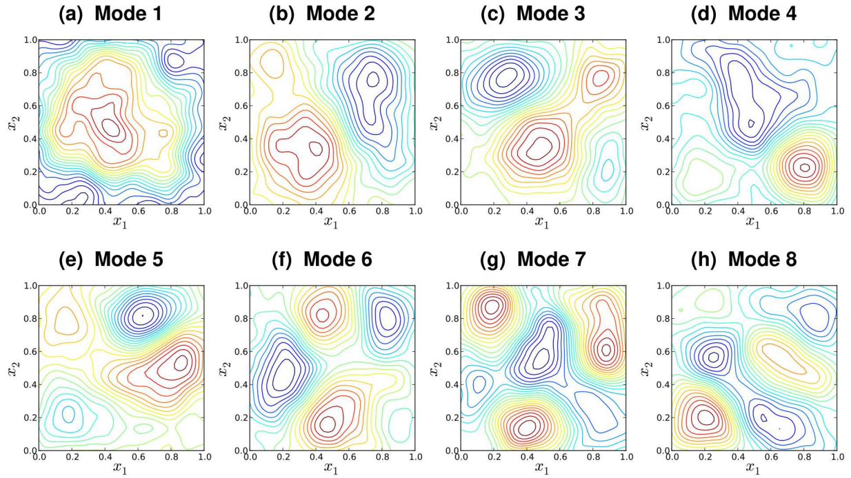
Figure 5-40. Illustration of first 8 KL modes, computed based on a numerical covariance matrix estimated using 2^{12} 2D RF realizations with c_l = 0.1
