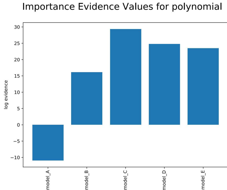
Figure 5-5. Importance Evidence Values for the Polynomial Model. As you can see, model C has the highest evidence value, implying the best fit. This is good because our true solution is of order 3.
