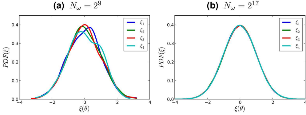
Figure 5-34. Probability densities for \xi_k obtained via KDE using samples obtained by projecting RF realizations onto KL modes. Results correspond to c_l = 0.05 .
