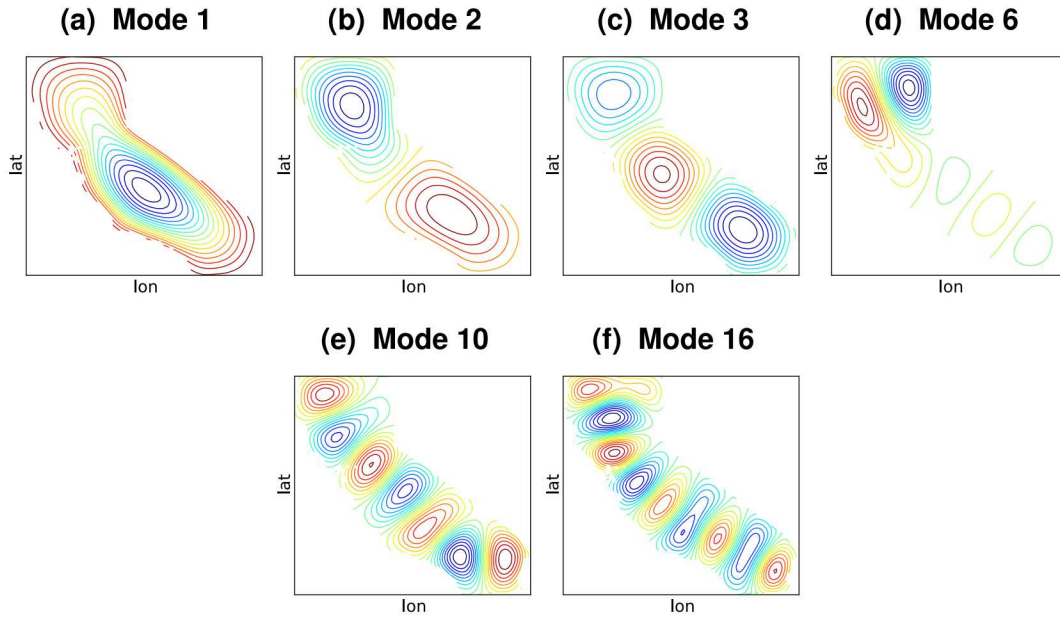
Figure 5-48. Illustration of select KL modes, computed based on an analytical covariance matrix for 2D RF realizations on an unstructured grid with c_l = 0.5^\circ and a square-exponential form.
