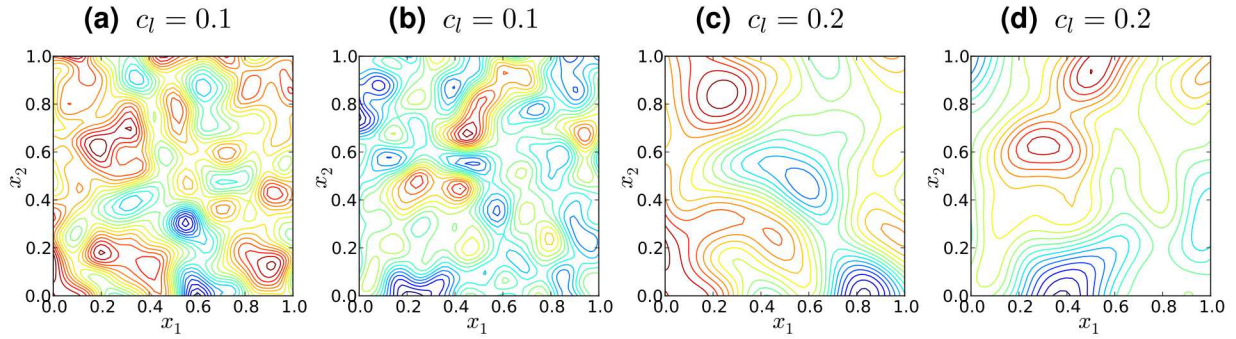
Figure 5-39. Sample 2D random field realizations for c_l = 0.1 and c_l = 0.2 .
