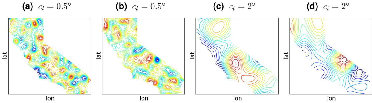
Figure 5-46. Sample 2D random field realizations on an unstructured grid for c_l = 0.5^\circ and c_l = 2^\circ .
