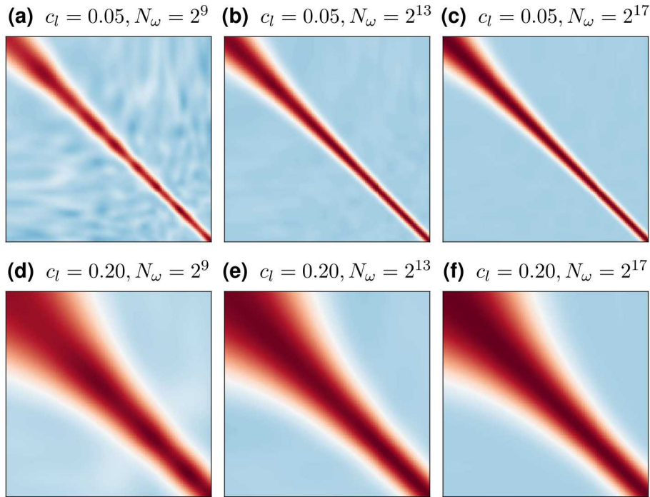
Figure 5-30. Illustration of covariance matrices computed from 1D RF realizations. Red corresponds to large values, close to 1, while blue corresponds to small values, close to 0.
