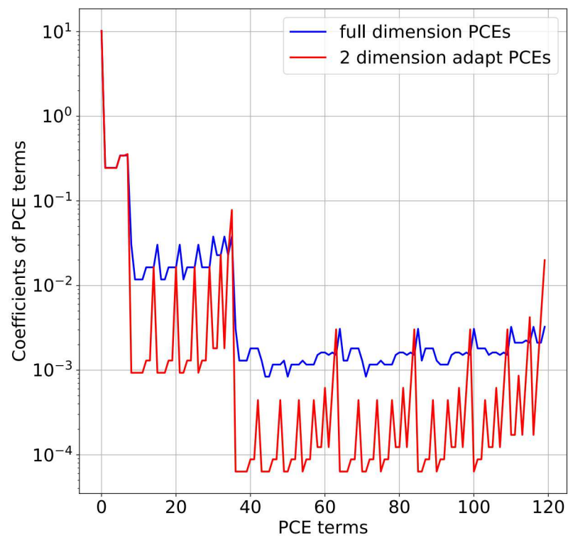
Figure 5-18. Coefficients comparison of adaptation method and full dimension PCE
