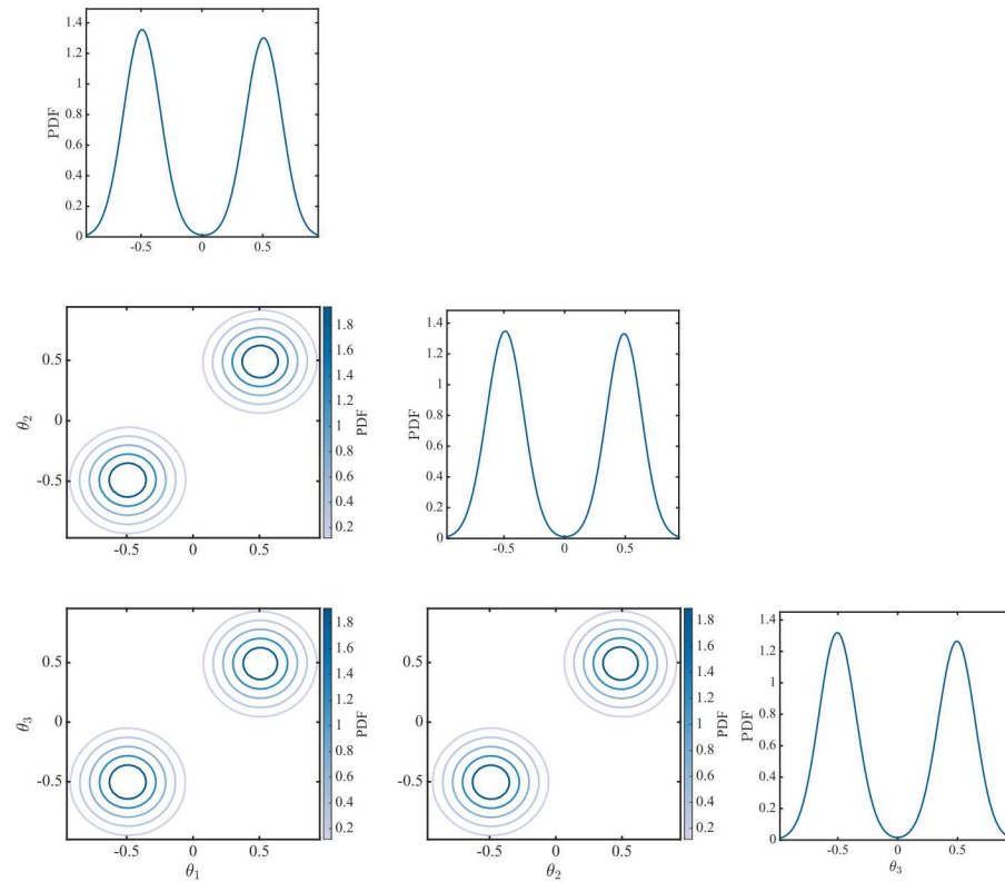
Figure 5-25. Marginal posterior distributions for all variables, as well as marginal joint posteriors
