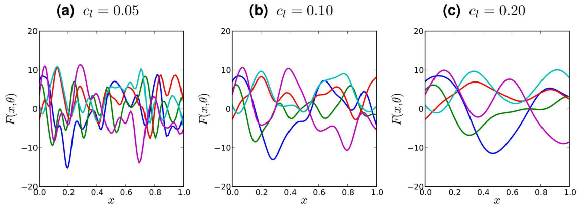
Figure 5-29. Sample 1D random field realizations for several correlation lengths c_l .
