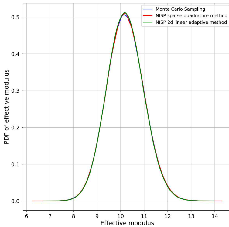
Figure 5-19. PDFs of effective modulus generated with different methods
