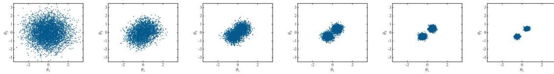
Figure 5-24. 2-dimensional scatter plots of intermediate TMCMC samples, from prior to posterior
