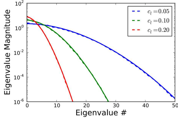
Figure 5-31. KL eigenvalues estimated with two sets of RF realizations: 2^9 = 512 (dashed lines) and 2^{17} = 131072 (solid lines).
