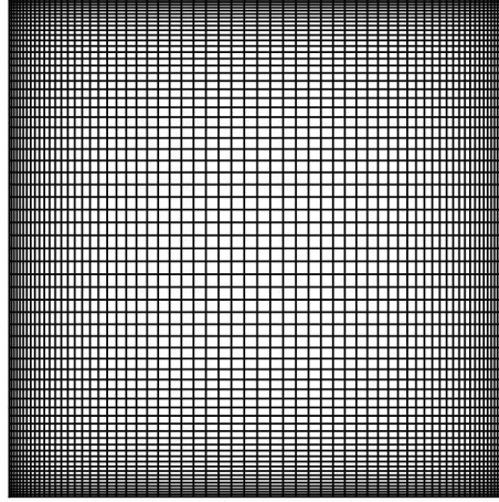
Figure 5-38. Structured grid employed for 2D RF examples.
