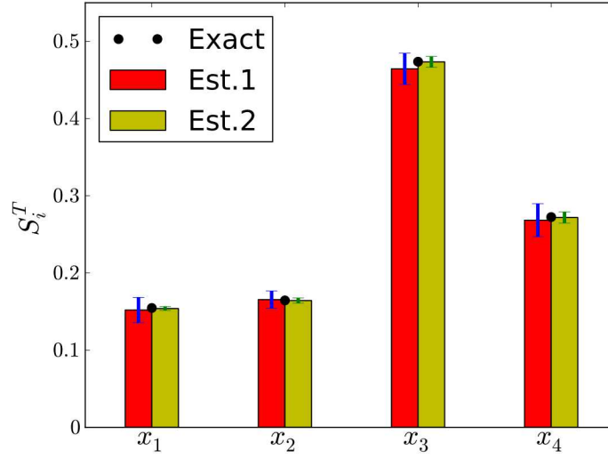
Figure 5-28. Total-order Sobol indices for the model given in Eq. (5.35). The red bars shows results based on Eq. (5.33) while the yellow bars are based on Eq. (5.34). The black circles show the theoretical values, computed analytically, and the error bars correspond to \pm\sigma computed based on an ensemble of 10 runs. For this model, Eq. (5.34) provides more accurate estimates for S_i^T compared to results based on Eq. (5.33).
