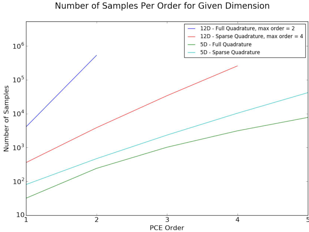
Figure 5-14. Increase in number of samples with change in order.
