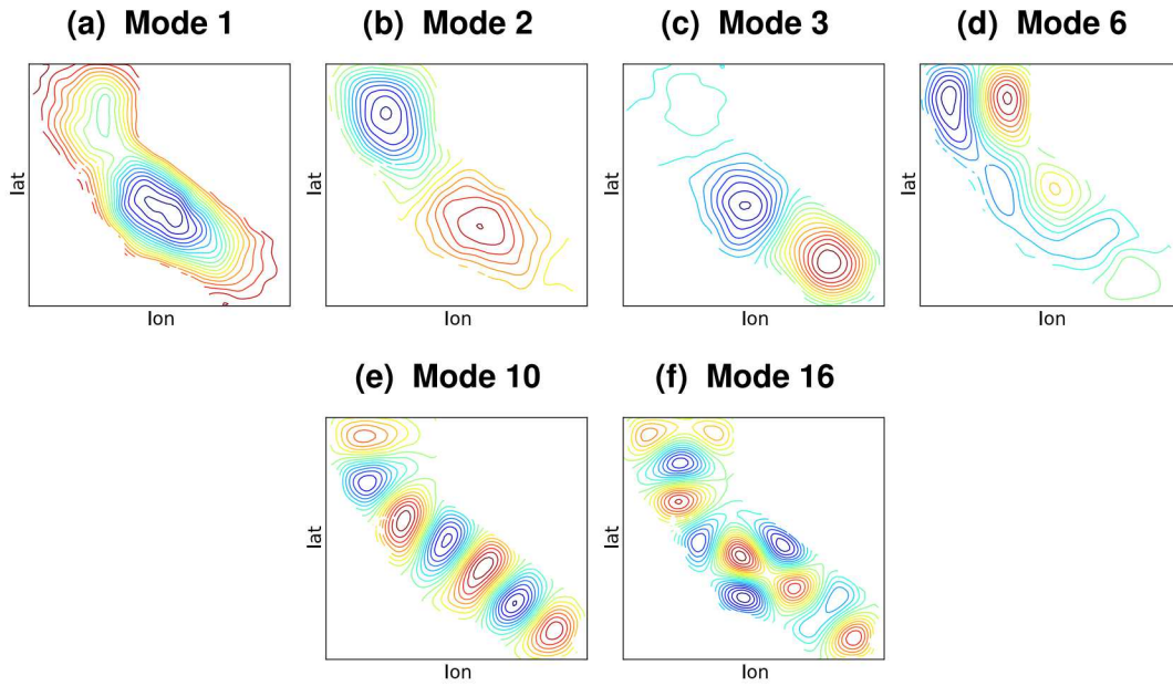
Figure 5-47. Illustration of select KL modes, computed based on a numerical covariance matrix estimated using 2^{16} 2D RF realizations on an unstructured grid with c_l = 0.5^\circ .
