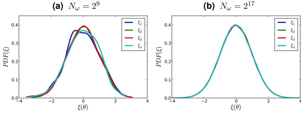
Figure 5-35. Probability densities for \xi_k obtained via KDE using samples obtained by projecting RF realizations onto KL modes. Results correspond to c_l = 0.20 .
