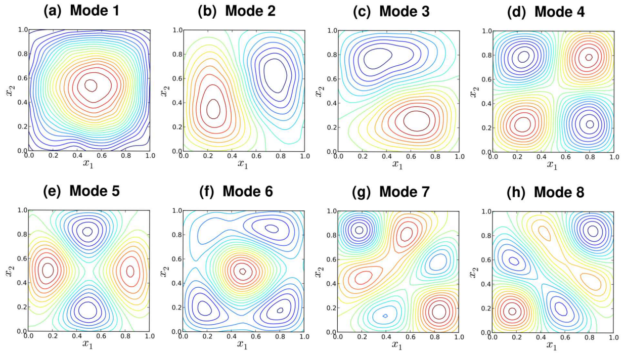
Figure 5-41. Illustration of first 8 KL modes, computed based on a numerical covariance matrix estimated using 2^{16} 2D RF realizations with c_l = 0.1
