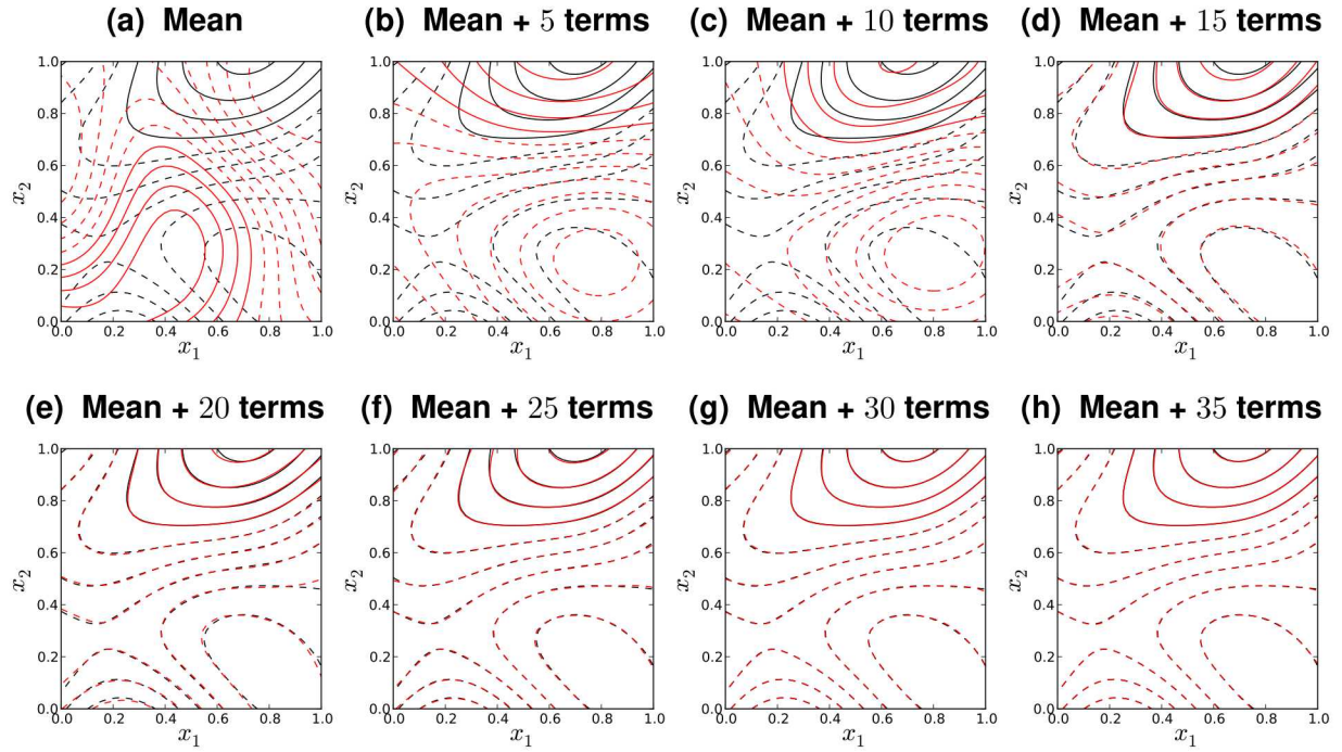
Figure 5-44. Reconstructing 2D realizations with an increasing number of KL expansion terms for c_l = 0.5
