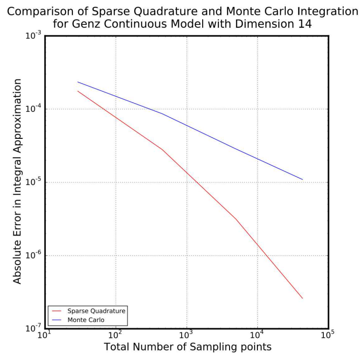
Figure 5-10. Samples results of sparse_quad.py
