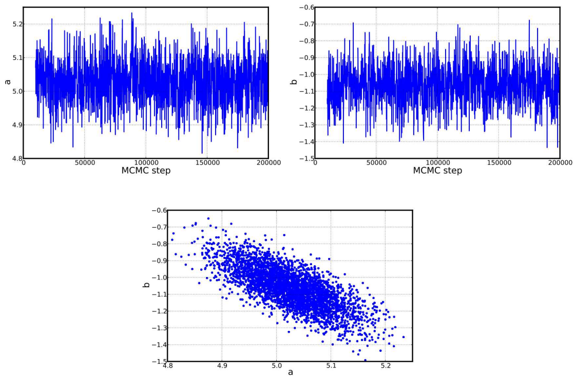
Figure 5-21. MCMC chains for parameters a and b , as well as a scatter plot for a and b
