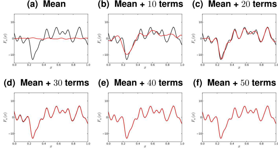
Figure 5-36. Reconstructing realizations with an increasing number of KL expansion terms for c_l = 0.05
