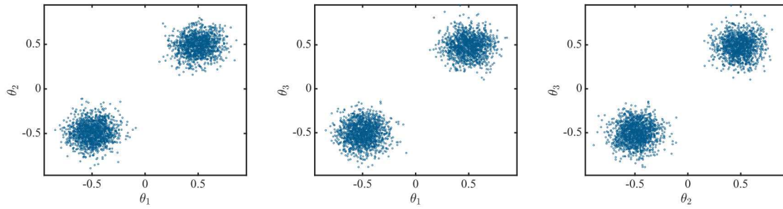
Figure 5-23. 2-dimensional scatter plots of posterior samples
