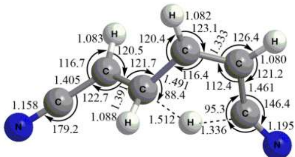
Figure 5. Optimized Cartesian coordinates (distances are given in Å and angles in degrees) of various intermediates, transitions states, and products.
