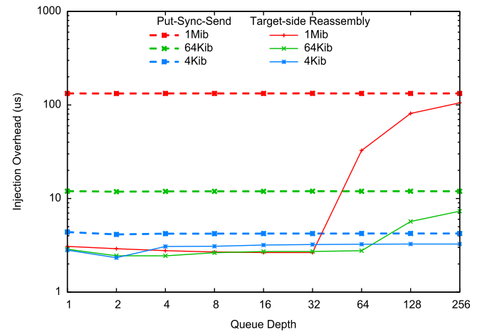
Figure 3. AM Long Injection Overhead Comparison
