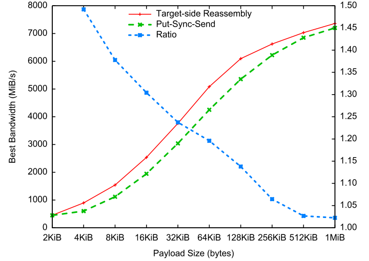
Figure 1. AM Long Ping-Pong Bandwidth Comparison
