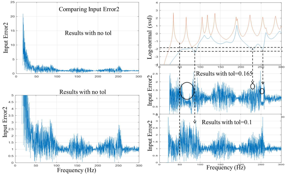
Figure 4. Input Error with Noise =10 and Effect of Regularization Parameter
