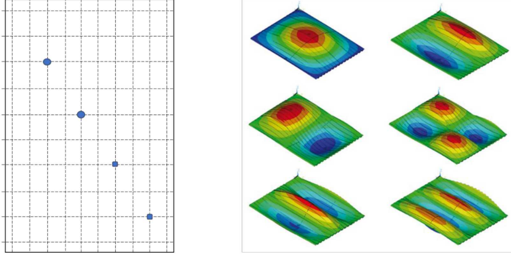
Figure 1. Simply-Supported Plate with Input and Output Locations and Mode Shapes
