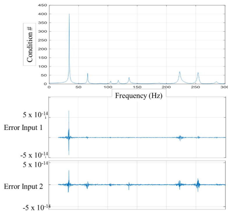
Figure 2. Condition # vs. Input Error with Zero Noise
