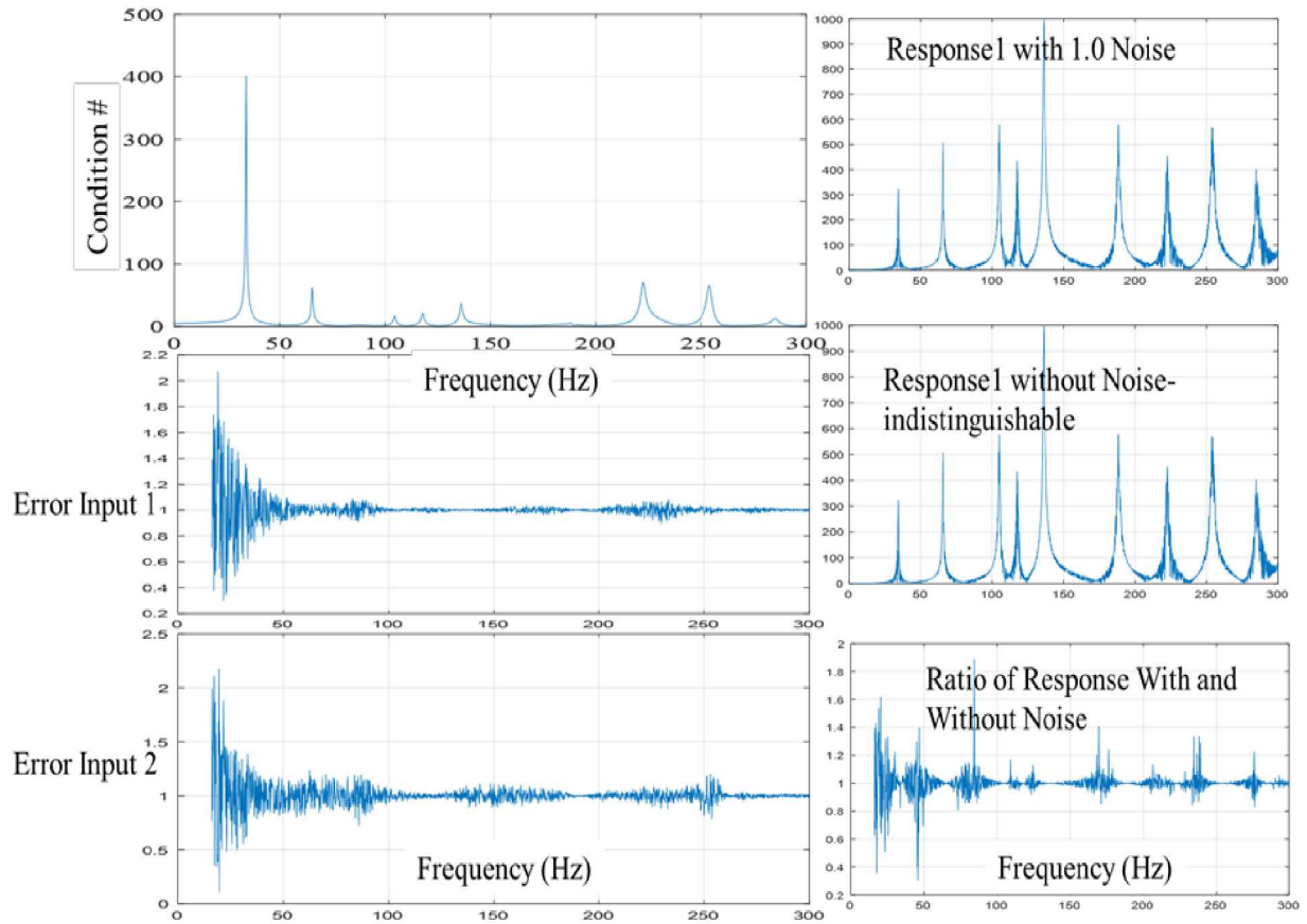
Figure 3. Condition # vs. Input Error with Noise =1.0
