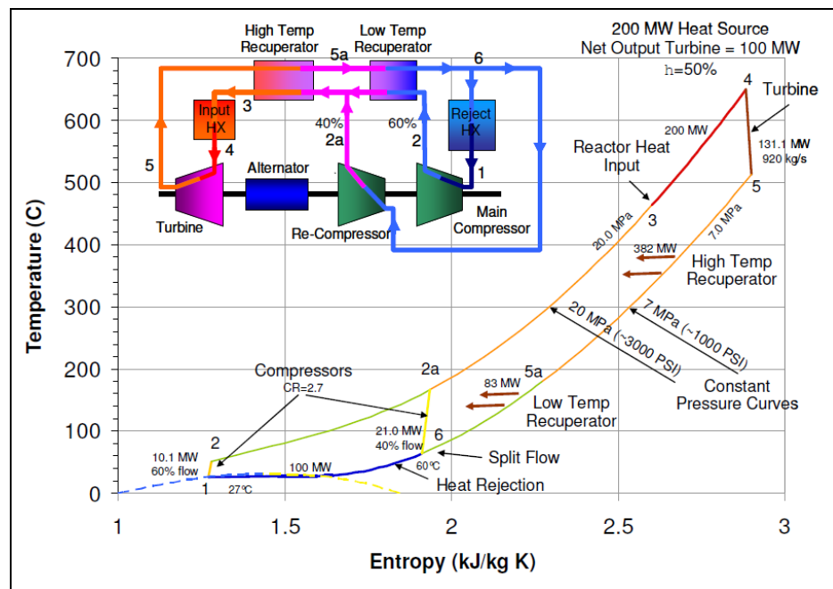
Figure 2. Diagram of SNL's sCO 2 Split Flow Recompression Brayton Cycle [23]
