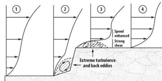
Figure 2-3. Behavior of wind over a bluff (NREL Small Wind Site Assessment Guidelines)
