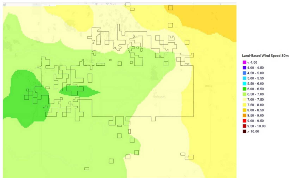
Figure 3-1. Land-Based Wind Speed (m/s) at 80 m over the Turtle Mountain reservation. (NREL Wind Prospector)
