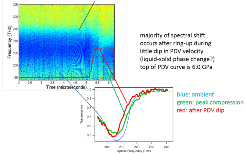
Figure 7. STL experiment results. Absorption curve shown in units of optical frequency instead of wavelength.
