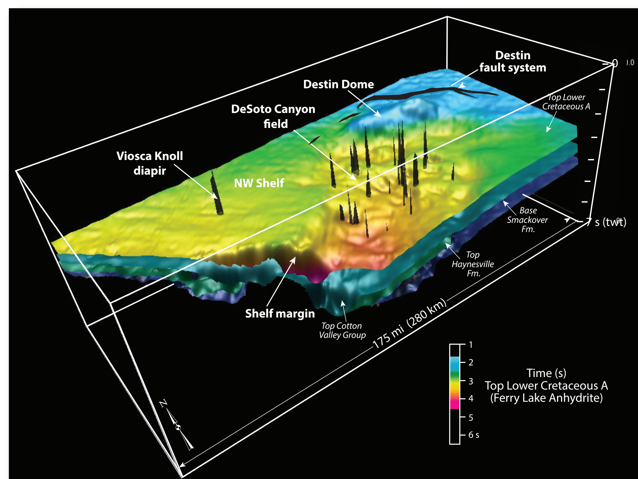
3D visualization of the top of the Ferry Lake Anhydrite showing major structural features of the DeSoto Canyon Salt Basin.
