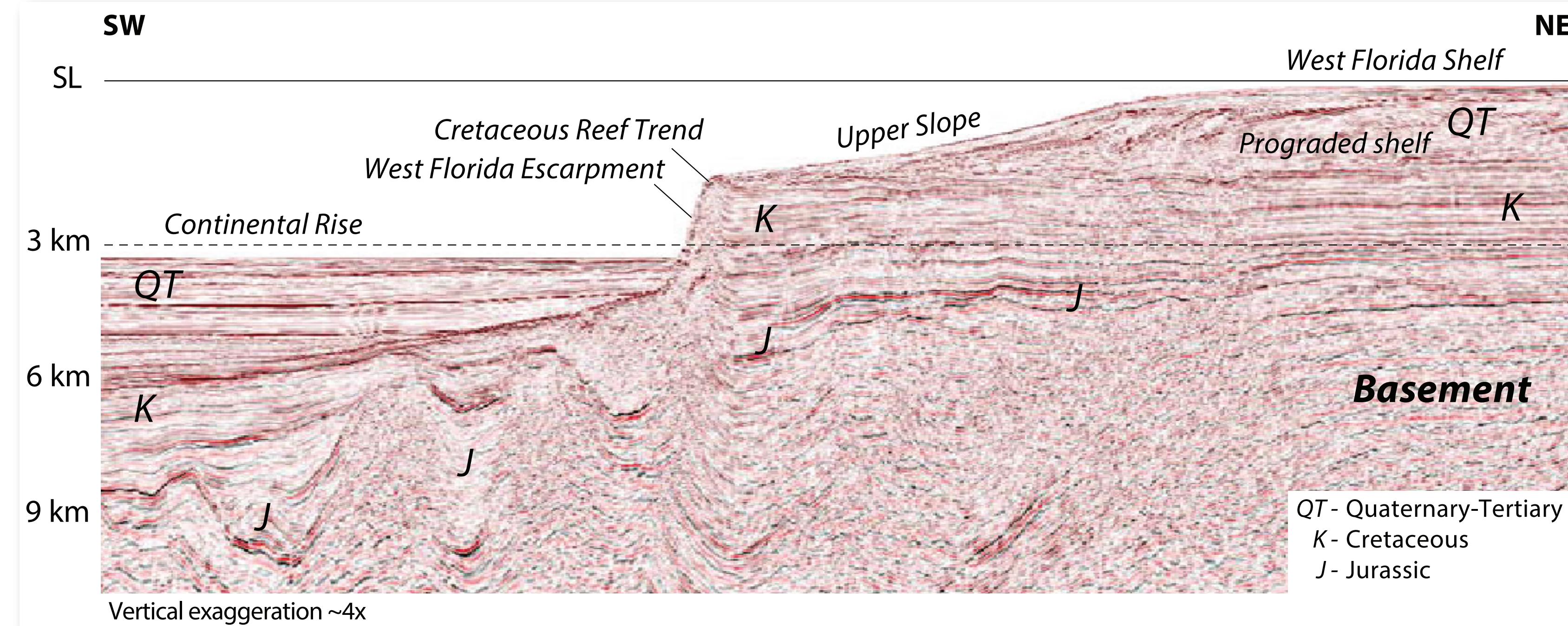
Pre-stack, depth-converted seismic profile showing geologic architecture along a transect from the West Florida Shelf to the continental rise (after Roberts and Erickson, 2009). Note major carbonate platform bounded by Cretaceous reef trend and overlain by prograded shelf. Structures southwest of platform include apparent Mesozoic minibasins below subhorizontal Cenozoic strata of the continental rise.
