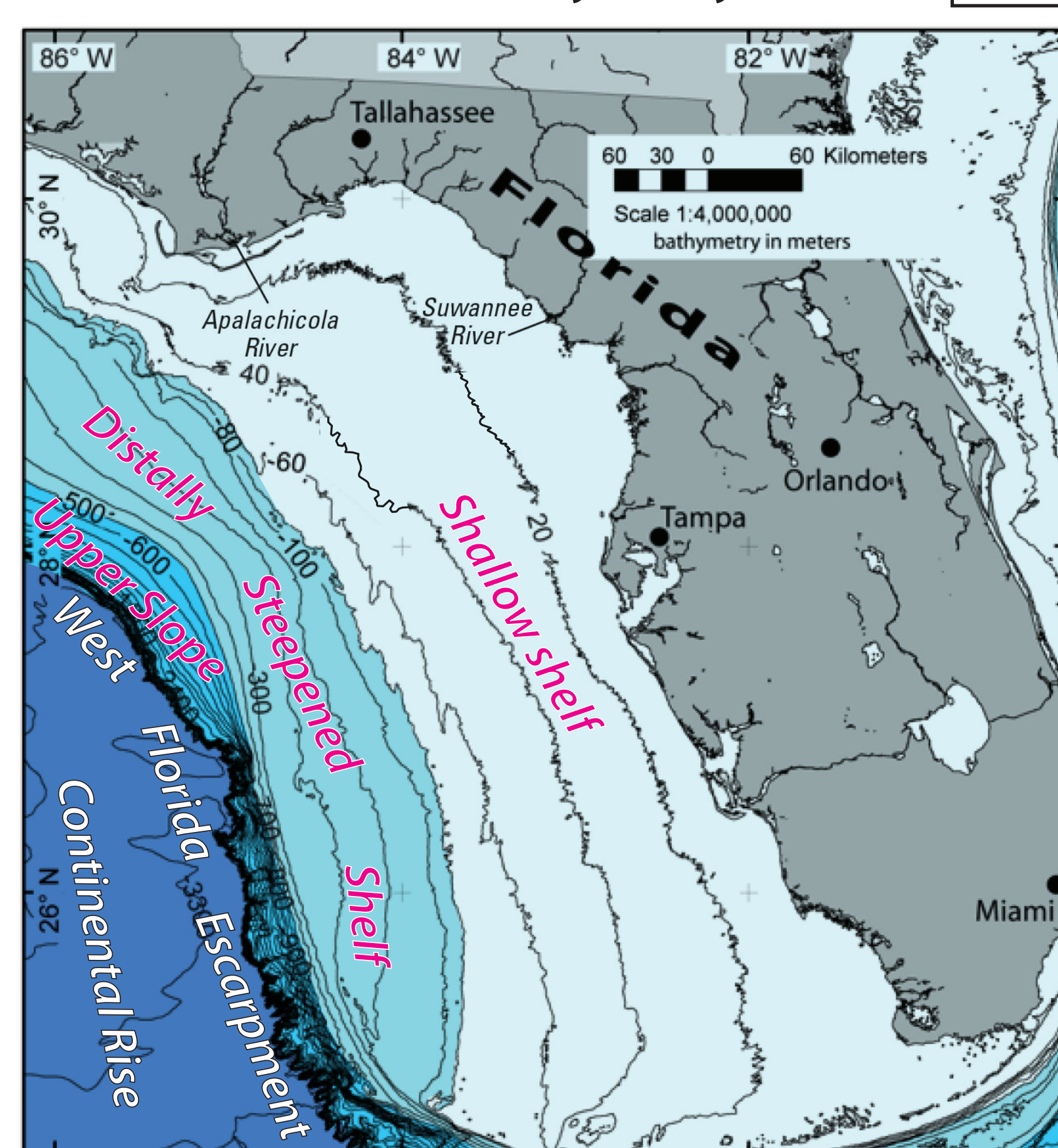
Bathymetric map of the West Florida Shelf (source: USGS). Note progressive steepening of the continental slope, culminating in the West Florida Escarpment.
