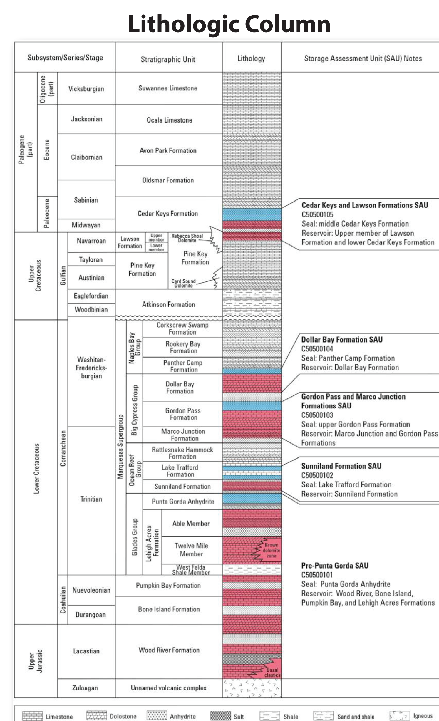
Stratigraphic column of the onshore South Florida Basin showing predominance of carbonate formations (after Roberts-Ashby et al., 2015). Prospective CO 2 sinks in red; evaporite seals in blue.
