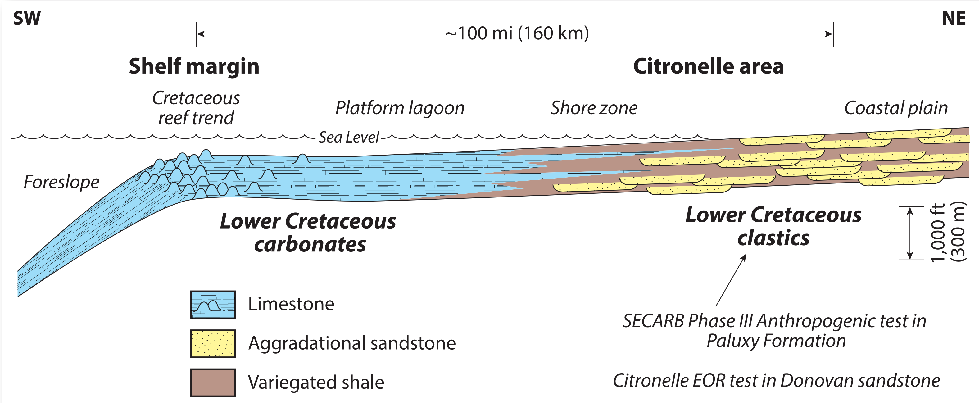
Cretaceous facies in the region are dominated by siliciclastic coastal plain deposits that pass basinward into reef-rimmed carbonate platform deposits. Siliciclastic strata include formations that have been tested for CO 2 storage potential onshore, whereas the storage potential of carbonate formations is less certain.
