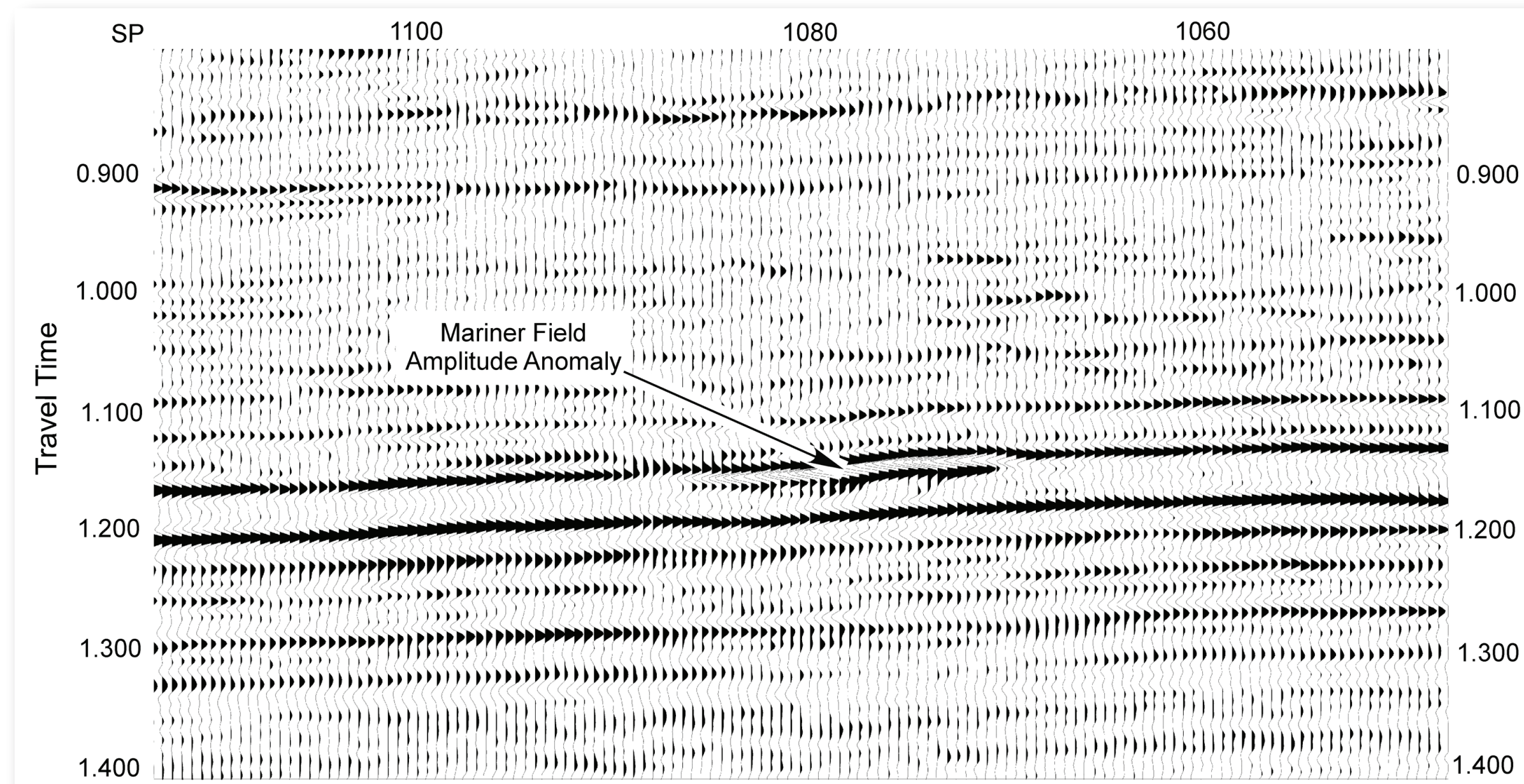
Seismic profile from Mariner Field, southern Mississippi showing amplitude anomaly (bright spot) associated with natural gas accumulation (after Handford and Baria, 2003). Preliminary analysis indicates that the bulk of the storage capacity in Miocene sandstone resides in saline formations below the commercial gas accumulations.
