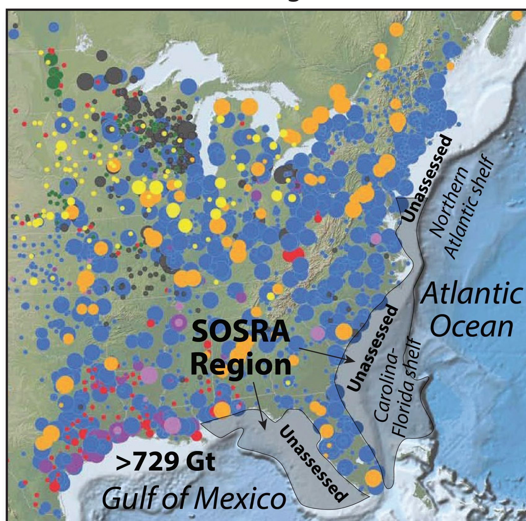
Map showing location of SOSRA region in relation to point source CO 2 emissions in the eastern United States (after NETL, 2012; SSEB, 2014).
