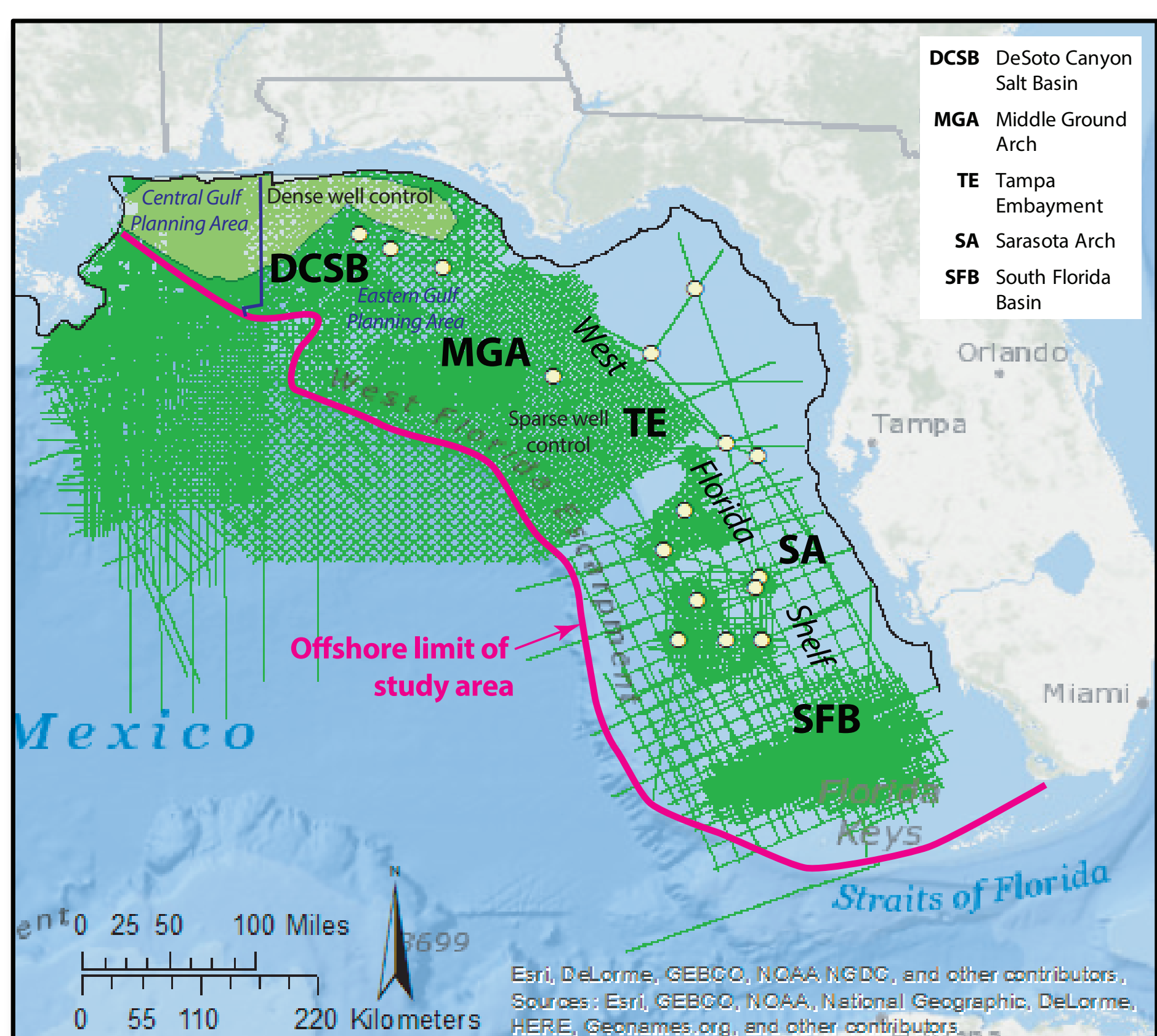
Map of eastern Gulf of Mexico focus area showing major geologic provinces. Green lines show reflection seismic control, yellow circles and shaded area indicate well control. Offshore limit of study area defined largely by location of Cretaceous reef trend.
