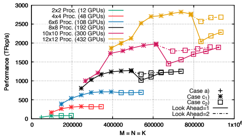
Figure 25: Strong-scaling performance of the matrix-matrix multiplication (PDGEMM)
