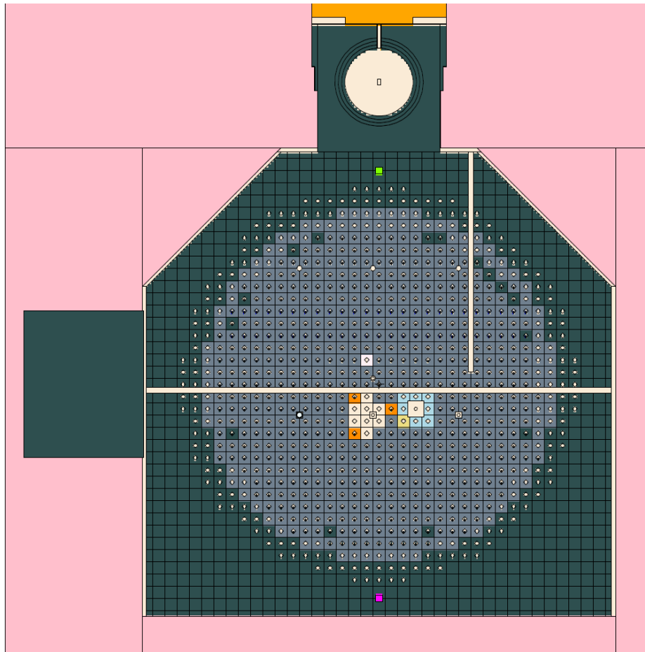
FIG. 83. (Color online) Computational model of the Mol-BR1 irradiation facility. The 1m diameter cavity within the thermal column is shown at the top of the figure.
