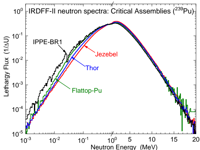
FIG. 96. (Color online) Neutron spectra for several critical assemblies containing ^{239}\text{Pu} from the ICSBEP Handbook [141]: Jezebel, Flattop-Pu, Thor and IPPE-BR-1. The spectra are presented in the 725 energy groups and normalized to unity. Note that the scale changes from log to linear above 1 MeV.
