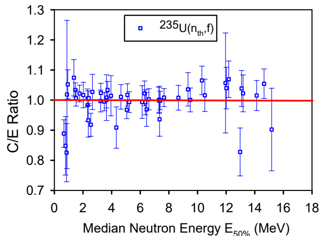
FIG. 116. (Color online) Least-squares-based C/E as a function of median energy E_{50\%} for the activity measurements in the ^{235}\text{U}(\text{n}_{th},\text{f}) reference neutron benchmark field. Uncertainties bars reflect the combined rms uncertainty contributions from the measurement, cross sections, and spectrum. Plotted values are listed in Table 39.
