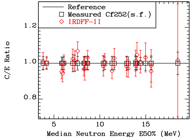
FIG. 99. (Color online) C/E relative to median energy E_{50\%} for the IRDF-II cross sections averaged in the ^{252}\text{Cf}(s.f.) neutron field measured at Řež near Prague. Plotted values are listed in Table 19.
