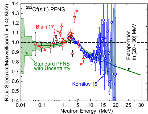
FIG. 66. (Color online) Standard ^{252}\text{Cf}(\text{s.f.}) prompt fission neutron spectrum (PFNS) and its uncertainties [33] as a ratio to the Maxwellian distribution with kT = 1.42 MeV (both spectra are normalised to unity). Spectrum extrapolation from 20 MeV to 30 MeV is shown by dash line. The recent new measurements [96] and [97] are plotted as symbols. Note that the scale changes from log to linear above 5 MeV.
