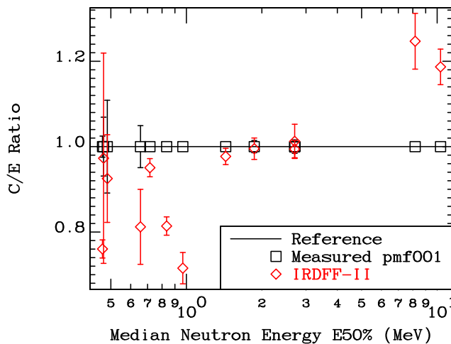
FIG. 109. (Color online) Ratio of Calculated and Measured SI in the central region of PMF001 (Jezebel) assembly.
