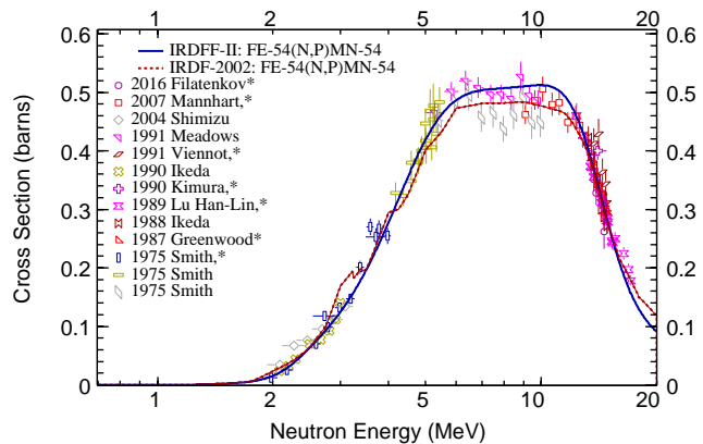
(a) Comparison to selected experimental data from EXFOR [73].
