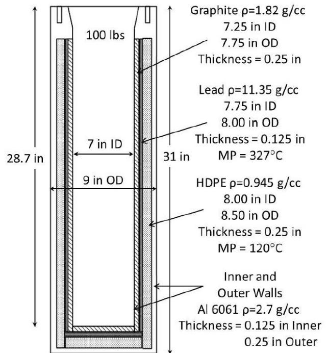
FIG. 81. "Bucket" used to tailor the ACRR-PLG neutron spectrum.
