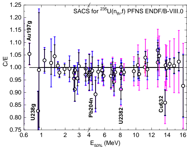
FIG. 100. (Color online) C/E as a function of median energy E_{50\%} for the IRDF-II cross sections averaged in the ^{235}\text{U}(n_{th},f) PFNS field are shown as circles. Uncertainty bars reflect a r.m.s. combination of uncertainty contributions from the measurement (black), IRDF-II cross sections (blue) and spectra (pink). Plotted values are listed in Table 20. Only outlying C/E values are labelled with reaction IDs from Table 20.
