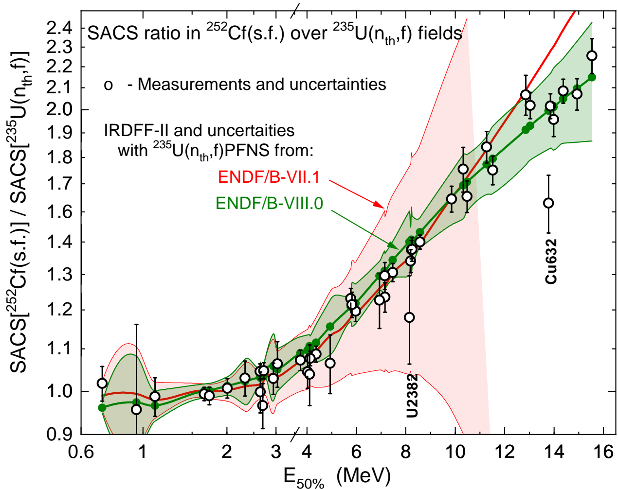
FIG. 101. (Color online) Ratio of SACS for the ^{252}\text{Cf} SFNS and ^{235}\text{U}(n_{th},f) PFNS fields as a function of median energy E_{50\%} : empty circles - measurements, filled circles and lines - computed with the IRDFF-II cross sections. Plotted values are calculated as ratios of SACS from Tables 18 and 19 to SACS listed in Table 20. Uncertainty bands associated with spectrum uncertainties are shown for ENDF/B-VII.1 and ENDF/B-VIII.0 ^{235}\text{U}(n_{th},f) PFNS fields.
