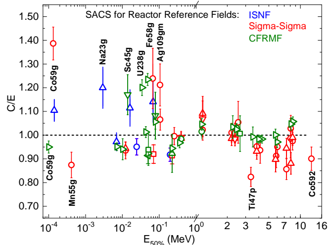
FIG. 113. (Color online) C/E ratios for SACS and spectral indices (SI) measured in the reference reactor fields: ISNF (blue symbols), CFRMF (green symbols), Sigma-Sigma (red symbols). Plotted C/E values are listed in Table 34. Outlying C/E values are labelled using reaction IDs from Table 34.
