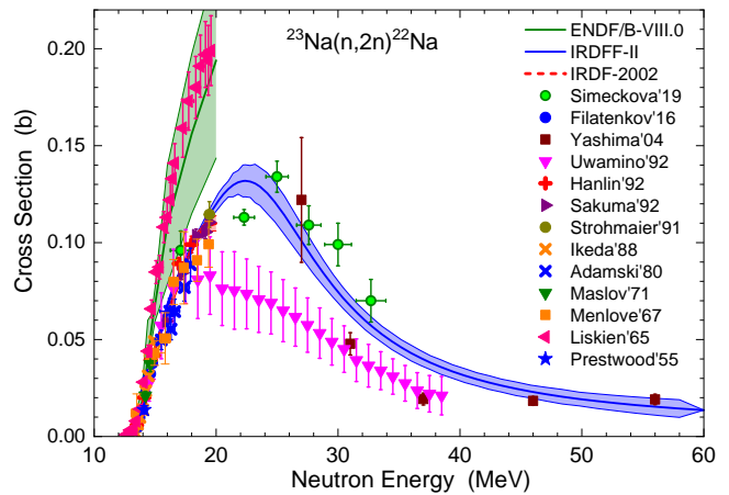
(a) Comparison to selected experimental data from EXFOR [73] and new data from Ref. [87] (Simeckova'19).
