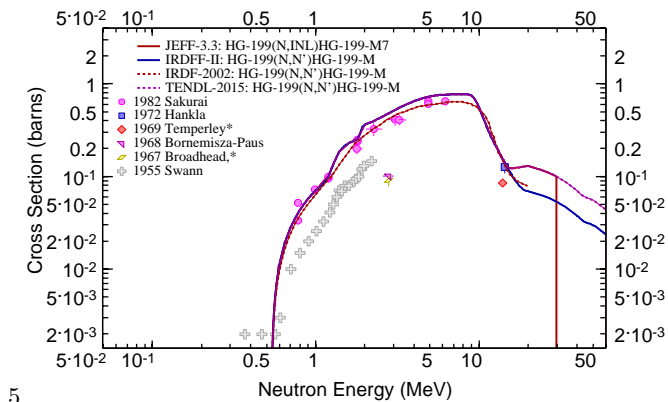
(a) Comparison to selected experimental data from EXFOR [73].
