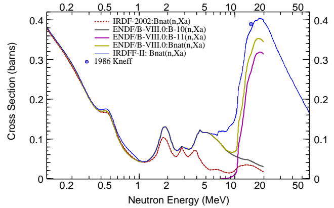
FIG. 65. (Color online) Comparison of the IRDF-II ^4\text{He} gas-production cross sections in neutron induced reactions on ^{\text{nat}}\text{B} target relative to Kneff et al. measurement [91].
