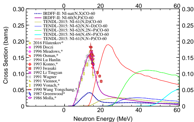
FIG. 8. (Color online) Contributing reactions to the ^{60}\text{Co} production from neutrons incident on a ^{\text{nat}}\text{Ni} target. Note that the cross sections are not scaled by the isotopic abundance.
