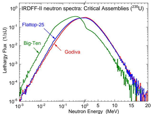
FIG. 94. (Color online) Neutron spectra for several critical assemblies containing ^{235}\text{U} from the ICSBEP Handbook [141]: Godiva, Flattop-25 and Big-Ten. The spectra are presented in the 725 energy groups and normalized to unity. Note that the scale changes from log to linear above 1 MeV.
