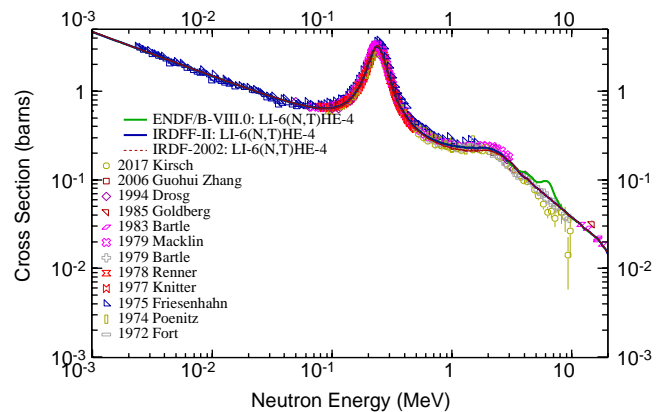
FIG. 55. (Color online) Comparison of ^6\text{Li}(n,t)^4\text{He} cross sections with other evaluations and experimental data from EXFOR.
