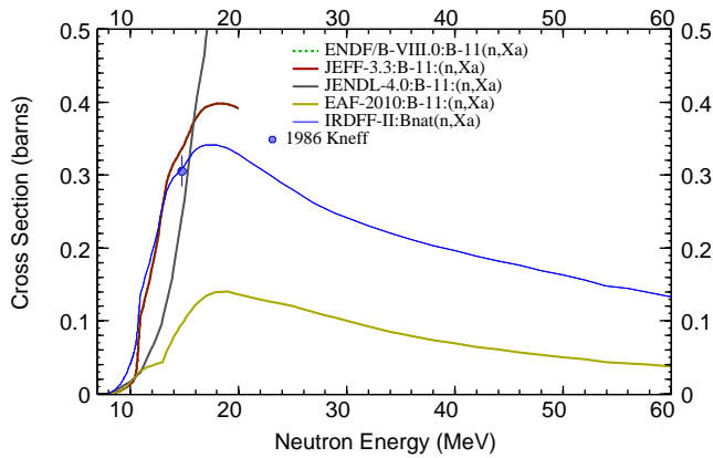
(a) Comparison of data from evaluated libraries relative to Kneff et al. measurement [91].
