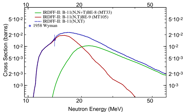
FIG. 63. (Color online) Comparison of the ^4\text{He} gas-production cross sections for the n+^{11}\text{B} reaction in the IRDF-II library.
