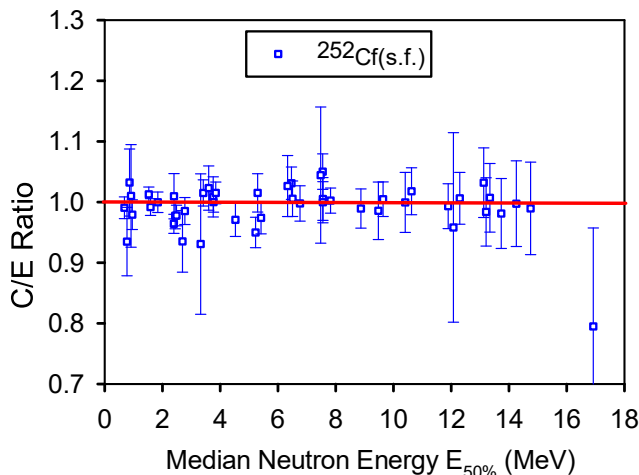
FIG. 115. (Color online) Least-squares-based C/E as a function of median energy E_{50\%} for the activity measurements in the ^{252}\text{Cf}(\text{s.f.}) standard neutron benchmark field. Uncertainties bars reflect the combined rms uncertainty contributions from the measurement, cross sections, and spectrum. Plotted values are listed in Table 38.
