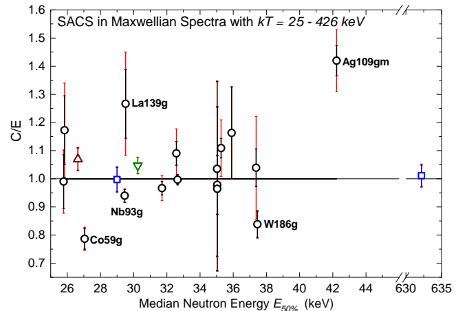
FIG. 114. (Color online) C/E ratios for SACS measured and calculated in the (25–426) keV Maxwellian spectra as a function of the median energy E_{50\%} . Plotted values are listed in Table 37. Experimental data: \circ - KADoNiS-1.0 [211], red triangle - P. Jimenez-Bonilla et al. [214], green triangle - G. Feinberg et al. [213], blue squares - A. Wallner et al. [215]. Uncertainties resulting from measurements and IRDF-II cross sections are shown by black and red bars. Only the outlying C/E values are labelled with reaction IDs from Table 37.
