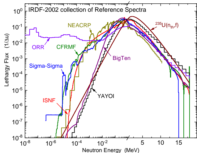
FIG. 91. (Color online) Neutron reference reactor spectra available in the IRDF-2002 collection [136]. Note that the scale changes from log to linear above 1 MeV.
