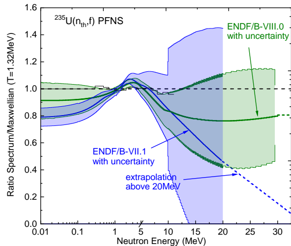
FIG. 68. (Color online) Reference ^{235}\text{U}(n_{th},f) prompt fission neutron spectrum (PFNS) [100–102] and its uncertainties as a ratio to the Maxwellian distribution with kT = 1.32 MeV (the spectra are normalised to unity). Red curve - from ENDF/B-VIII.0 [31], black curve - from ENDF/B-VII.1 [34]. Extrapolations beyond 20 MeV or 30 MeV are shown by dashed lines. Note that the scale changes from log to linear above 5 MeV.
