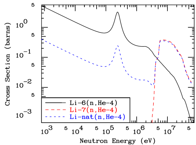
FIG. 60. (Color online) Comparison of the IRDF-2 {}^4\text{He} gas-production cross sections in neutron induced reactions on {}^6\text{Li} , {}^7\text{Li} , and {}^{nat}\text{Li} targets.
