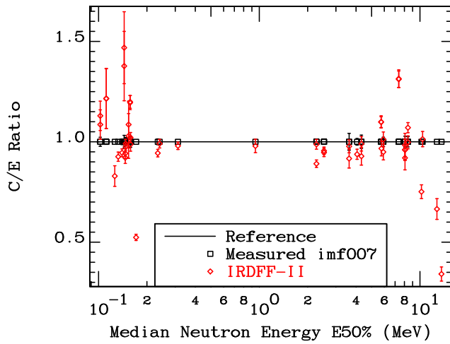
FIG. 108. (Color online) Ratio of Calculated and Measured SI in the central region of IMF007 (Big-Ten).
