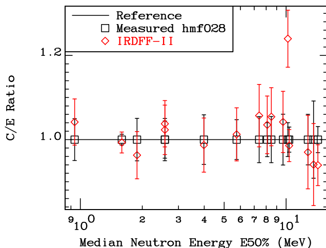
FIG. 107. (Color online) Ratio of Calculated and Measured SI in the central region of HMF028 (Flatop-25).
