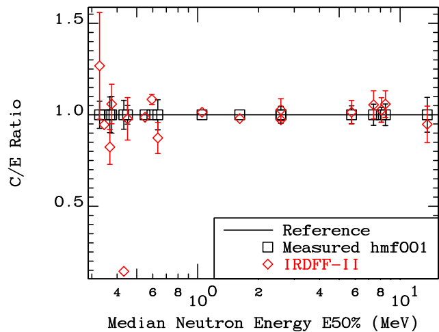
FIG. 106. (Color online) Ratio of Calculated and Measured SI in the central region of HMF001 (Godiva).
