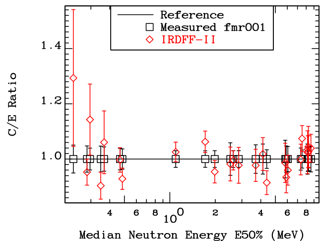
FIG. 112. (Color online) Ratio of Calculated and Measured SI in the central region of FMR001 assembly (formally designated FUND-IPPE-FR-MULT-RRR-001 in ICSBEP).
