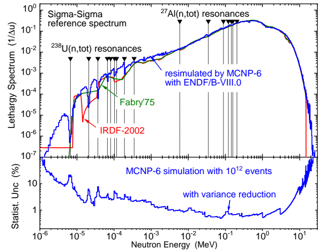
FIG. 92. (Color online) The Sigma-Sigma reference spectrum: original from IRDF-2002 (red curve), published by Fabry [130] (green) and recalculated in this work (blue). The bottom part shows the statistical uncertainties obtained in the Monte-Carlo simulations with variance reduction techniques.
