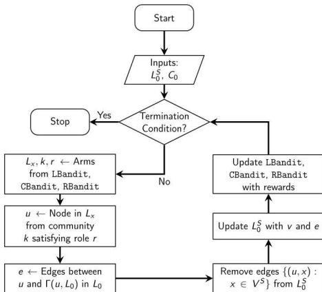
Figure: The flowchart for MABSample.
