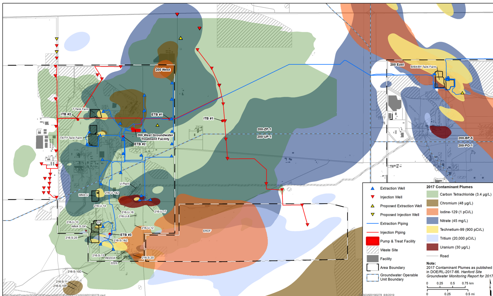
Figure 4. 200 West Area contaminant plumes and pump-and-treat system wells (adapted from DOE 2018b).
