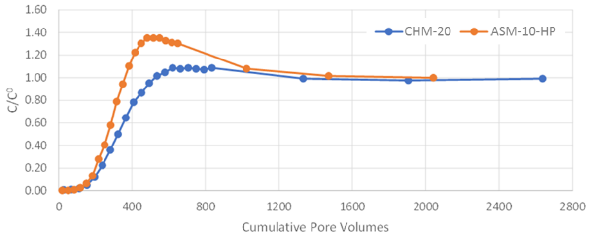
Figure 6. Column effluent concentration of iodate expressed as a ratio to the influent concentration for the cerium-based resin (CHM-20) and the ferrihydrite-based resin (ASM-10-HP) (adapted from Szecsody et al. 2019).
