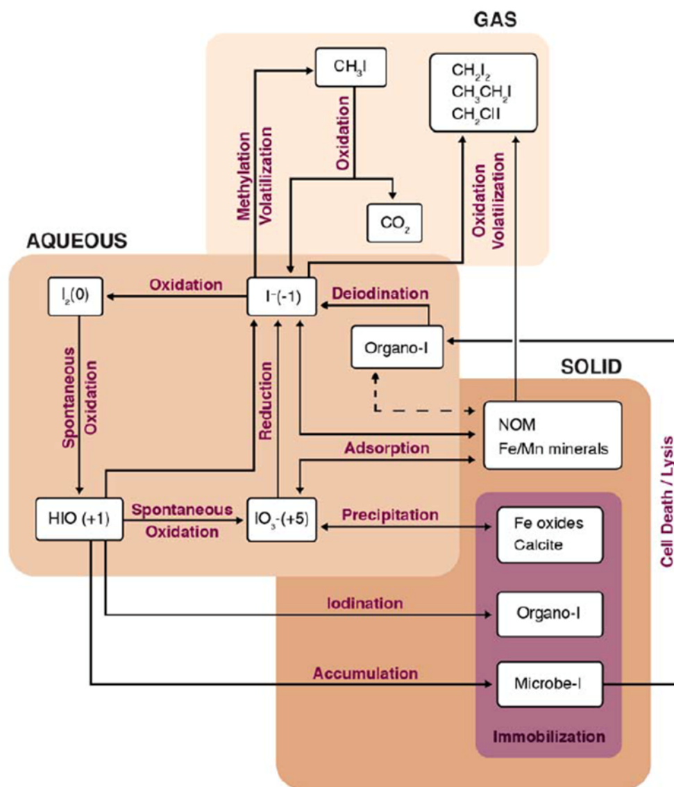
Figure 5. Hanford site biogeochemical process for iodine (adapted from Neeway et al. 2019)
