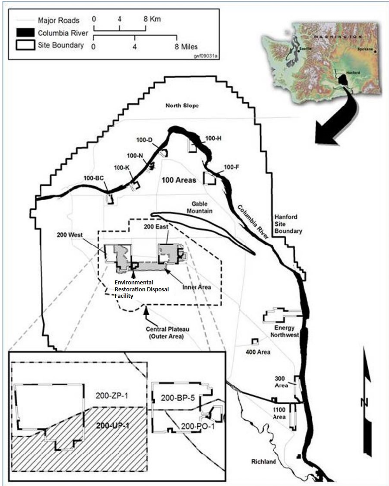
Figure 2. Location of 200-UP-1 Operable Unit on the Central Plateau at the Hanford Site (DOE 2013)
