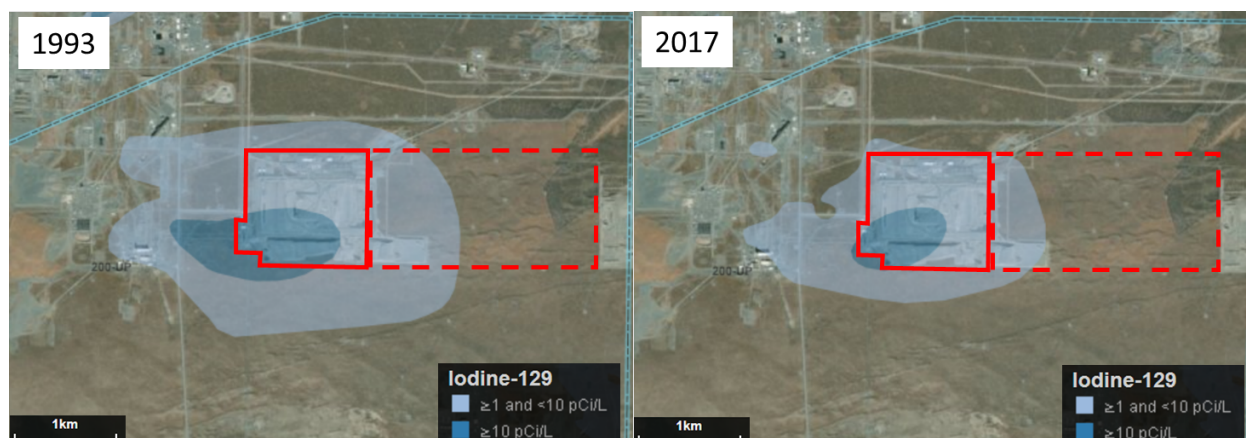
Figure 3. Plume maps for I-129 for 1993 and 2017 from DOE (2018a) as displayed by the PHOENIX web application plume animator ( https://phoenix.pnnl.gov/apps/plumes/index.html ). Solid red line show the current Environmental Restoration Disposal Facility (ERDF). The dotted red line shows the eastward future expansion area of ERDF.
