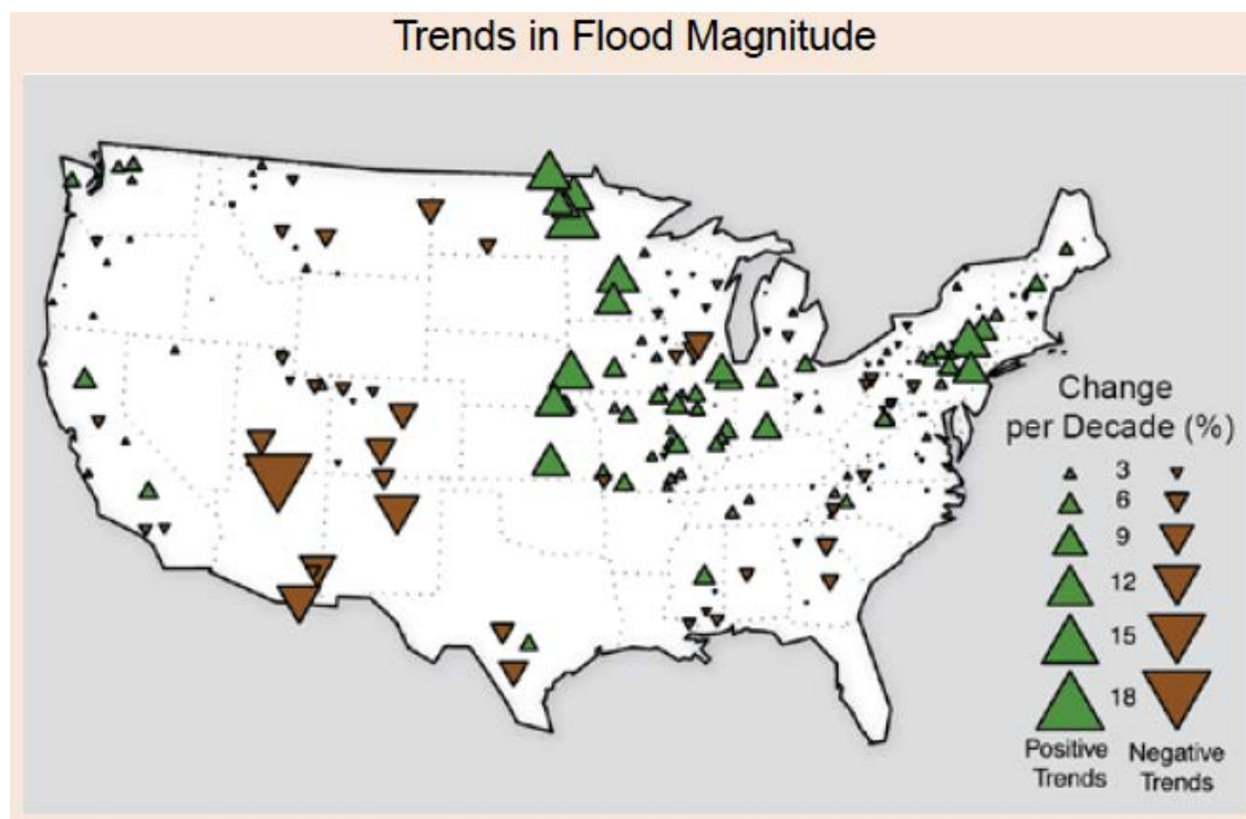
Figure 3.11. Trends of Annual Flood Magnitude from 1920s through 2008. (Source: Melillo et al. 2014, Figure 2.21 and Peterson et al. 2013)
