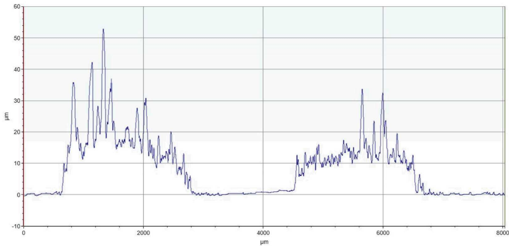
Figure 4. Profilometry measurement of additivity manufactured inductor.
