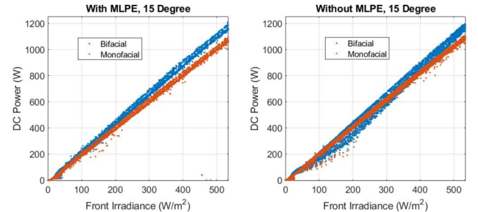
Fig. 5. Power (temperature corrected) as a function of front irradiance at the low irradiance range.
