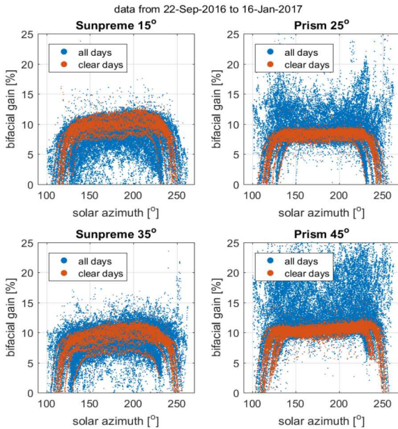
Fig. 3. Bifacial gain on each of the rows of the test field, typically between 7% and 10%.
