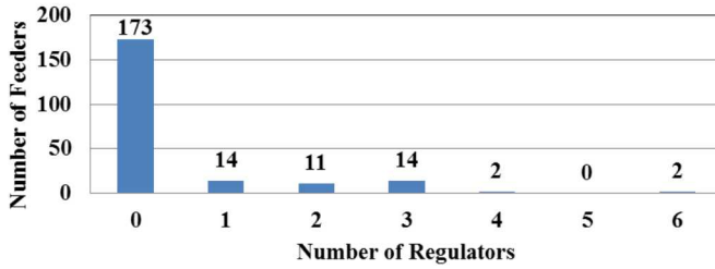
Figure 1. Histogram of the number of voltage regulators on each feeder.
