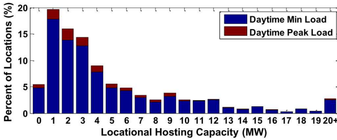
Figure 6. Stacked histogram of locational hosting capacity colored by the load level that determined the hosting capacity of that location.
