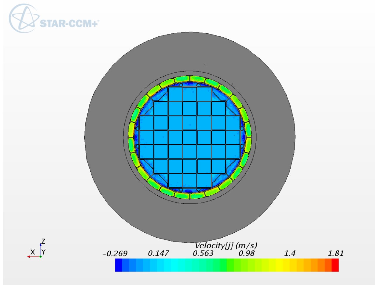
Figure 7-7. Distribution of Vertical Component of Velocity at Mid-Height of Basket
