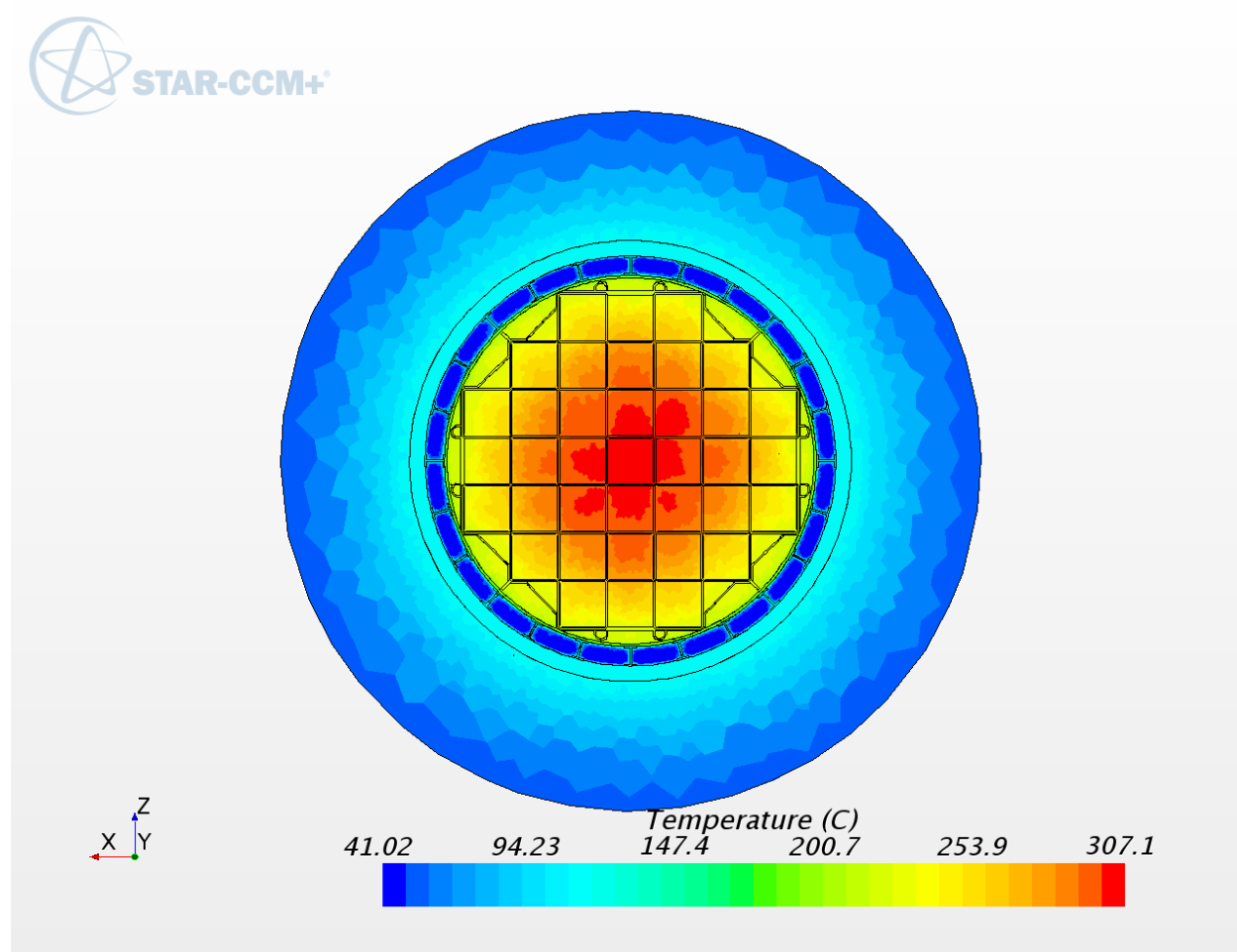
Figure 7-4. Radial Temperature Distribution
