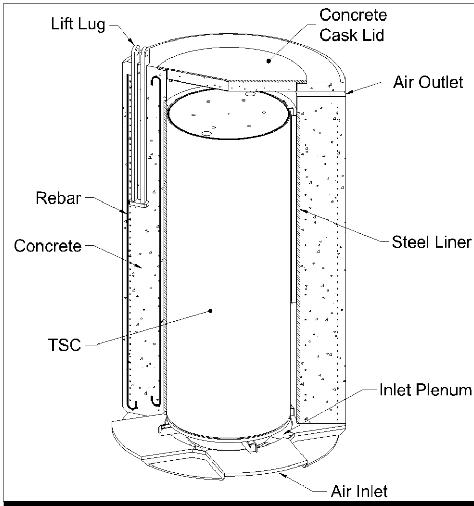
Figure 2-1. MAGNASTOR Storage System
