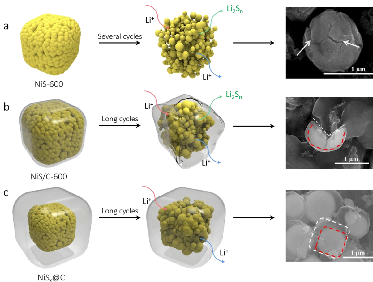
Figure 6. The illustration of structure changes and ex-situ SEM of a) NiS-600, b) NiS/C-600, and c) NiS x @C during cycling process.
