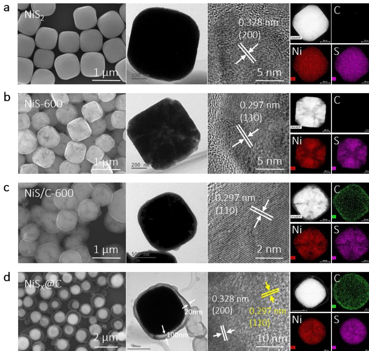
Figure 2. The SEM, TEM, HRTEM images and EDS elemental mappings of a) \text{NiS}_2 , b) \text{NiS-600} , c) \text{NiS/C-600} , and d) \text{NiS}_x\text{@C} , respectively.
