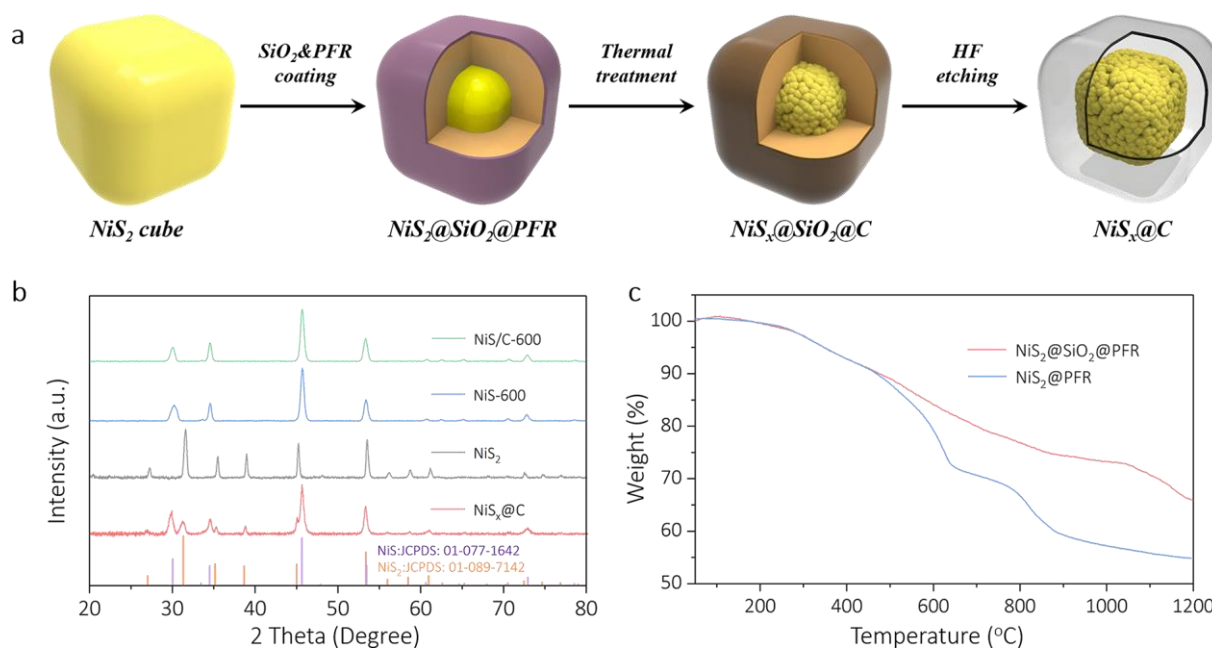
Figure 1. a) The schematic illustration of the synthesis procedure of \text{NiS}_x\text{@C} . b) XRD patterns of \text{NiS/C-600} , \text{NiS-600} , \text{NiS}_2 and \text{NiS}_x\text{@C} . c) TGA curves of \text{NiS}_2\text{@SiO}_2\text{@PFR} and \text{NiS}_2\text{@PFR} .
