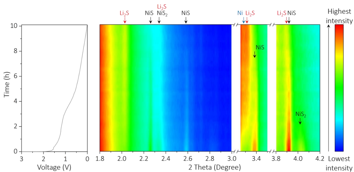
Figure 3. In-situ synchrotron HEXRD of \text{NiS}_x@C electrode during the first discharge process.
