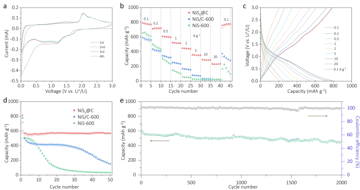
Figure 4. a) Cyclic voltammograms of NiS x @C at a scan rate of 0.1 mV s -1 . b) Rate performance of NiS x @C, NiS/C-600, and NiS-600. c) The corresponding discharge/charge curves of NiS x @C at different current density. d) Cycling performance of NiS x @C, NiS/C-600, and NiS-600 at 1 A g -1 . e) Long cycle performance of NiS x @C at 1 A g -1 .
