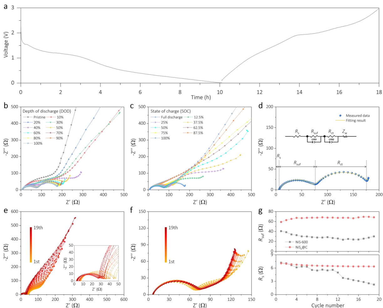
Figure 5. In-situ electrochemical impedance spectra characterization of the NiS x @C electrode in comparison with the NiS-600 electrode in three-electrode cells. a) Initial discharge/charge curve of NiS x @C electrode for in-situ EIS tests. In-situ time-lapse EIS profiles of NiS x @C electrode at different depths of discharge (DOD) (b) and different states of charge (SOC) (c) during the initial discharge/charge. d) Nyquist plot of a.c. impedance spectra for the NiS x @C electrode measured at full discharge state (inset is the equivalent circuit model). In-situ EIS profiles of NiS-600 (e) and NiS x @C (f) at full discharge state from 1 st to 19 th cycles. f) Plots of R s and R surf against cycle number.
