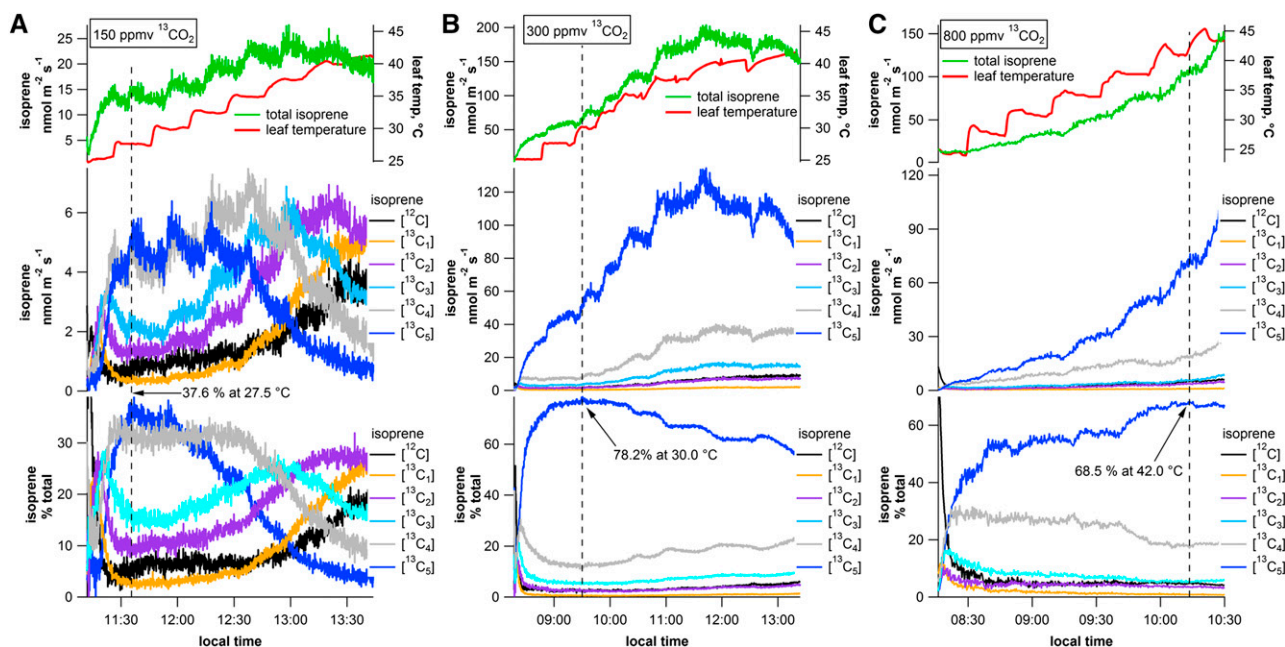
Figure 4. Representative PTR-MS time series plots showing absolute and relative emissions (percentage of total) of [^{12}\text{C}] isoprene and [^{13}\text{C}_{1-5}] isoprene as a function leaf temperature from three separate shimbillo leaves exposed to 150 (A), 300 (B), and 800 (C) ppmv ^{13}\text{CO}_2 . Note that increased ^{13}\text{CO}_2 concentrations strongly enhance the temperature corresponding to the maximum relative emissions of [^{13}\text{C}_5] isoprene (150 ppmv, 27.5°C; 300 ppmv, 30.0°C; and 800 ppmv, 42.0°C).
