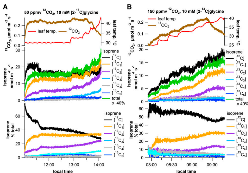
Figure 6. Representative CRDS and PTR-MS time series plots showing the influence of increasing leaf temperature on absolute emissions of photorespiratory ^{13}\text{CO}_2 , [ ^{12}\text{C} ]isoprene, and [ ^{13}\text{C}_{1-5} ]isoprene from detached shimibillo leaves in a 10 mM [2- ^{13}\text{C} ]Gly solution under 50 ppmv ^{12}\text{CO}_2 (A) and 150 ppmv ^{12}\text{CO}_2 (B). Also shown are the relative emissions (percentage of total) of [ ^{12}\text{C} ]isoprene and [ ^{13}\text{C}_{1-5} ]isoprene. Note the general pattern of increasing relative emissions of [ ^{13}\text{C}_{1-4} ]isoprene and a decrease in [ ^{12}\text{C} ]isoprene with temperature.
