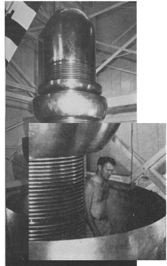
Photos of a three-stage accelerator that came online in 1965 at Los Alamos Scientific Laboratory (now LANL). The instrument accelerated hydrogen, deuterium, and tritium ions to up to 24.5 MeV.
