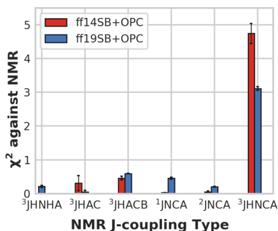
Figure 8. \chi^2 errors in reproducing six NMR scalar coupling data for Ala 5 , with data for ff14SB+OPC (red) and ff19SB+OPC (blue). The MD simulations were run for a total of ~3 \mu s.
