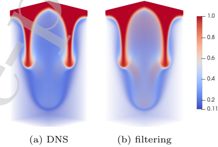
Figure A.3. Comparison of the density field between DNS and simulations with filtering in 3D RTI at Re_p = 450 , A = 0.8 , at \tau = 2.5 . (a) is a DNS on a 128 \times 128 \times 256 grid, and (b) uses filtering on a 64 \times 64 \times 128 grid. The maximum relative difference ( \frac{DNS-filtering}{filtering} ) is 4.78%. Differences in the color rendering is due to the DNS grid being finer with a higher grid-point density, which leads to slightly darker colors despite the pointwise numerical values being almost identical.
