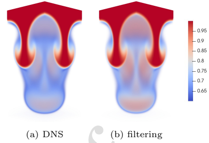
FIG. A.2. Comparison of the density field between DNS and simulations with filtering in 3D RTI at Re_p = 800 , A=0.25 , at \tau=2.5 . (a) is a DNS on a 128 \times 128 \times 256 grid, and (b) uses filtering on a 64 \times 64 \times 128 grid. The maximum relative difference ( \frac{DNS-filtering}{filtering} ) is 0.29%. Differences in the color rendering is due to the DNS grid being finer with a higher grid-point density, which leads to slightly darker colors despite the pointwise numerical values being almost identical.
