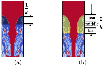
FIG. 13. Plots illustrating the regions used in calculating vorticity \omega_0 = \frac{\int_V \rho |\omega|^2 dV}{2 \int_V \rho dV} , where V is the volume inside the bubble tip. k = 2\pi/l_x is the wavenumber. (a) The gray region is used in Fig. 14, which has a vertical distance of 1/k . (b) The yellow region is composed of three disjoint regions (near, middle and far regions). Each region has a vertical distance of 2/(3k) . The three disjoint regions are used in Fig. 15.
