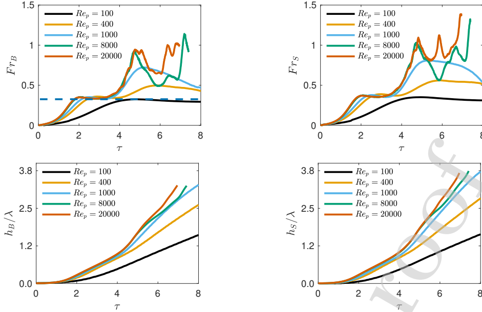
FIG. 3. Effects of Re_p on the bubble velocity Fr_B (top left), the spike velocity Fr_S (top right), the bubble front location h_B (bottom left), and the spike front location h_S (bottom right) in 2D RTI at A = 0.04 . The dashed line shows the potential model prediction of Fr_B = \sqrt{1/(3\pi)} . h_{B/S} is measured relative to the initial interface position z_0 = 0.5L_z . The plots show that the bubble and spike growth (both velocities and heights) are similar at low A and Re_p , however they experience asymmetric growth at late times at the highest Re_p , even at low A = 0.04 cases shown here. A sustainable re-acceleration stage is observed at high Re_p . The results are similar to the incompressible RTI results in Ref. [38]. Note that, \tau here is smaller than the definition used in Ramaprabhu et al. [35, 37] by a factor \sqrt{2\pi} ( \tau = 6 here corresponds to time \approx 15 in [35, 37]).
