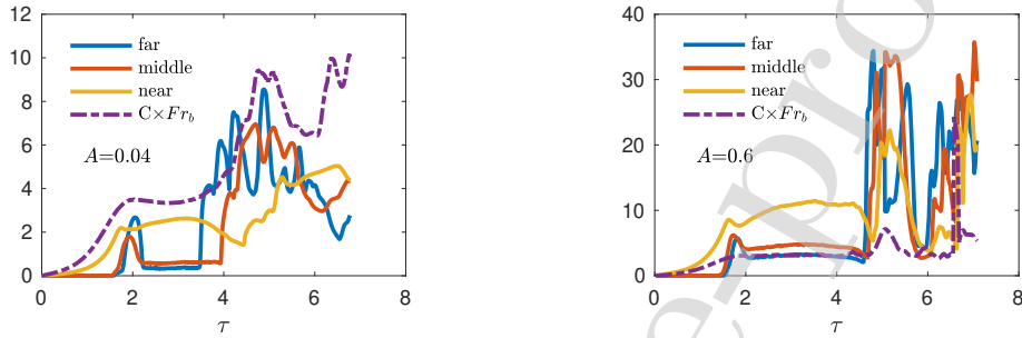
FIG. 15. Time evolutions of averaged vorticity \omega_0 within the three disjoint regions inside the bubble from two 2D Re_p = 20000 simulations. The regions are explained in Fig. 13(b). The vertical distance for each region is 2/(3k) . The dashed line shows Fr_b multiplied by a constant C = 10 for better comparison. Left (right) panel shows A = 0.04 ( A = 0.6 ) results. The results indicate vortices are advected from the bottom towards the bubble tip, and leads to bubble re-acceleration at low A = 0.04 . At high A = 0.6 , the vortices are also advected from the bottom towards the bubble and leads to fluctuations in speed around \tau = 6 .
