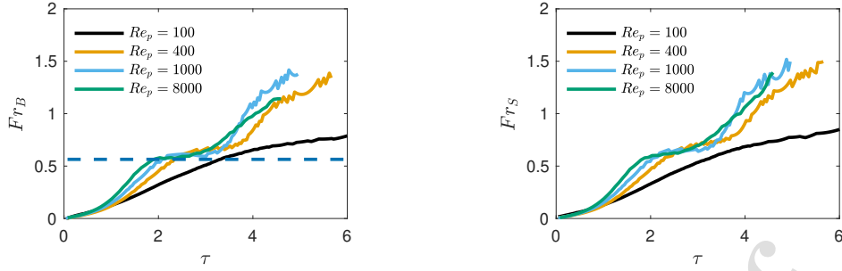
FIG. 8. Time evolutions of bubble (left panel) and spike (right panel) velocities at A = 0.04 and different Re_p in 3D RTI. The dashed line shows the potential model of F_{r_B} = \sqrt{1/\pi} . The plots show 3D RTI develop faster and is easier to re-accelerate than its 2D counterpart. Note that, \tau here is smaller than the definition used in Ramaprabhu et al. [35, 37] by a factor \sqrt{2\pi} ( \tau = 6 here corresponds to time \approx 15 in [35, 37]).
