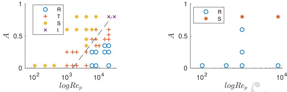
FIG. 10. Re-acceleration A - Re_p phase diagram in 2D (left panel) and 3D (right panel) RTI. The late-time behavior of the bubble front is classified into 4 phases: 1) (R) denotes a robust re-acceleration exists at late times; 2) (T)ransient means the bubble front re-acceleration is temporary and eventually decelerates at late times; 3) (S)aturation phase indicates that the bubble front saturates near the “terminal velocity” after the linear stage, with possible eventual decay at very long times; 4) (I)ntermittent phase means the bubble front velocity is characterized by intermittent large amplitude fluctuations without clear long time trend.
