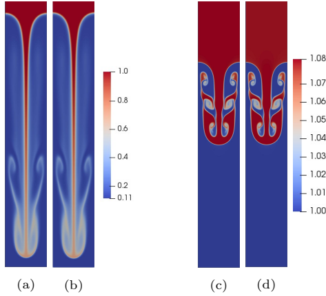
FIG. A.1. Comparison of the density field between DNS and simulations with filtering in 2D RTI. (a) and (b) simulate RTI at Re_p=1100 and A=0.8 at \tau=6 . (a) is a DNS on a 256 \times 2048 grid, and (b) uses filtering on a 128 \times 1024 grid. (c) and (d) simulate RTI at Re_p=8000 , A=0.04 at \tau=4 . (c) is a DNS on a 512 \times 4096 grid, and (d) uses filtering on a 256 \times 2048 grid. Note that the images are cropped in the vertical to save space (domain aspect ratio is 8).
