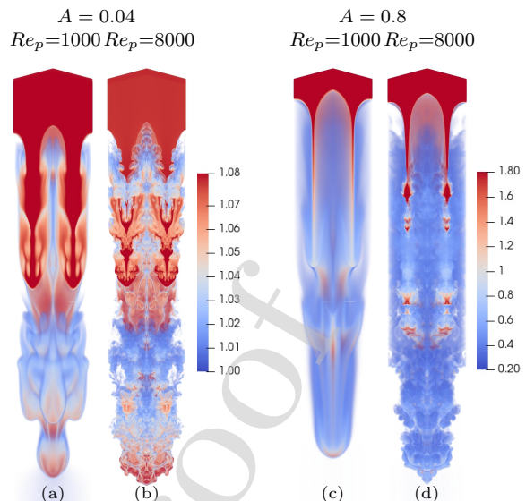
FIG. 7. 3D density \rho visualizations at \tau = 5 . (a), (b) are results at A = 0.04 for Re_p = 1000 and 8000 , respectively. (c), (d) are results at A = 0.8 for Re_p = 1000 and 8000 , respectively. Note the initial interface position is z_0 = 0.5L_z for A = 0.04 and z_0 = 0.75L_z for A = 0.8 . The plots show that 3D RTI generates more vortical structures than 2D RTI.
