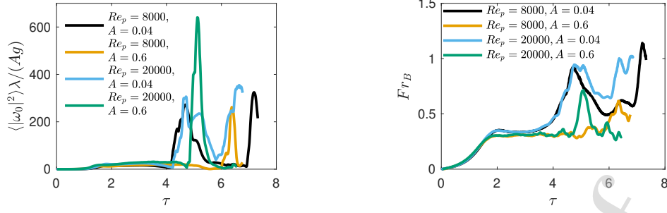
FIG. 14. Comparison between the spatially-averaged normalized vorticity \langle |\omega_0|^2 \rangle \lambda / (Ag) inside the bubble and the bubble velocity Fr_B for 2D simulations. The plots show that there is a strong correlation between vorticity and bubble velocity in the nonlinear stage of the RTI growth.
