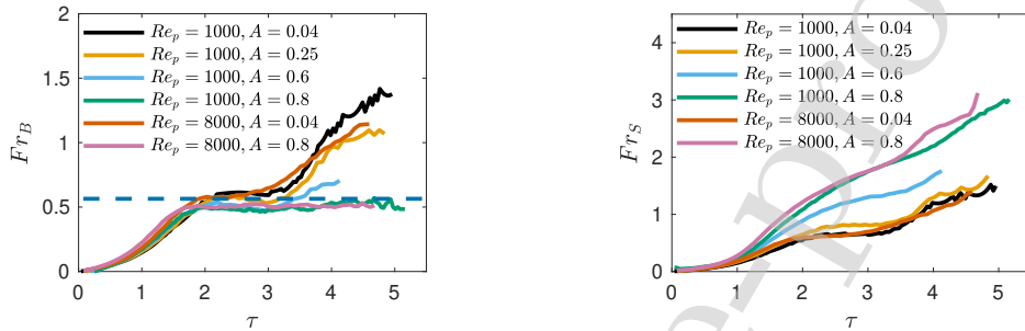
FIG. 9. Time evolutions of the bubble (left panel) and spike (right panel) velocities at different A for two Re_p in 3D RTI. The dashed line shows the potential model of F_{r_B} = \sqrt{1/\pi} . Note that, \tau here is smaller than the definition used in Ramaprabhu et al. [35, 37] by a factor \sqrt{2\pi} ( \tau = 6 here corresponds to time \approx 15 in [35, 37]).
