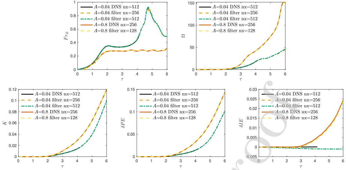
FIG. A.5. Comparison of bubble velocity Fr_B (top left), entropy \Omega (top right), kinetic energy K (bottom left), release of potential energy \delta PE (bottom middle), and change in internal energy \delta IE (bottom right) between DNS and filtering results for 2D RTI. RTI is simulated at A = 0.04 , Re_p = 8000 using DNS on a 512 \times 4096 grid, and filtering on 256 \times 2048 and 512 \times 4096 grids. We also show RTI at A = 0.8 , Re_p = 1100 using DNS on a 256 \times 2048 -grid and filtering on a 128 \times 1024 -grid. Note that the plots of K , \delta P , and \Omega for A = 0.04 are multiplied by 5.
