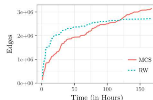
Figure 3: Number of edges found vs time by MCS (red) and random walk (green) using the real Twitter API.
