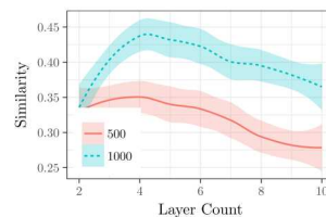
(c) Sensitivity of MCS to number of layers at different budgets.
