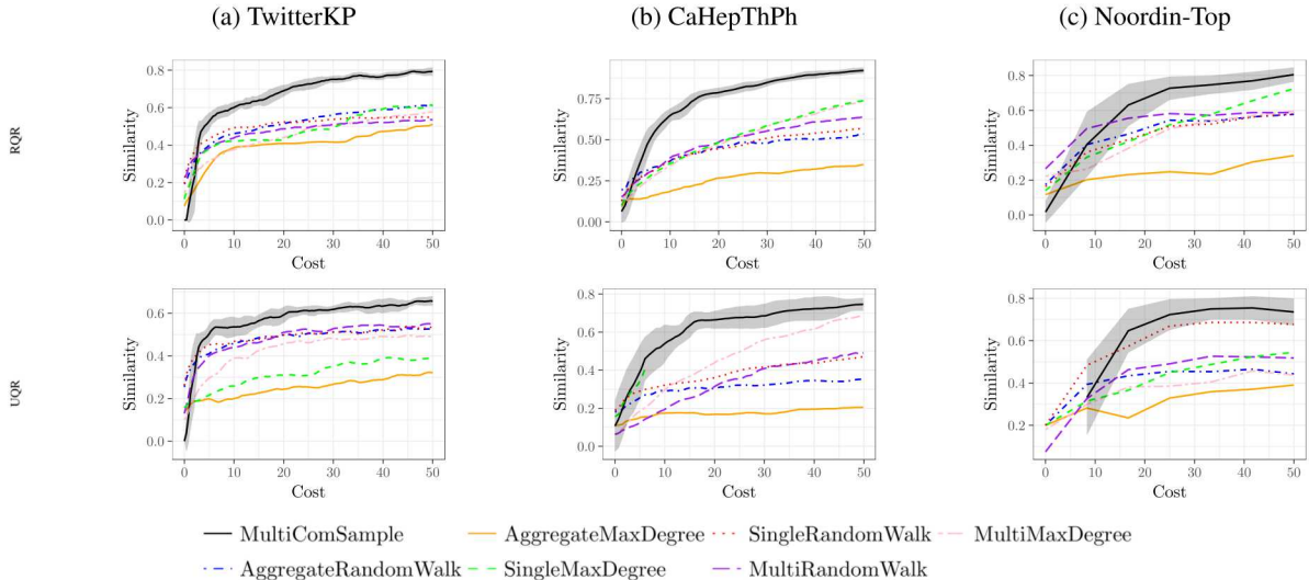
Figure 1: Comparison of MCS against various baseline algorithms on different networks in the case of RQR (top row) and UQR (bottom row). The y -axis is the similarity between the community structure in the sample and the ground truth, and the x -axis is the budget consumed as a percentage of the total budgets required to query all nodes in L_0 .
