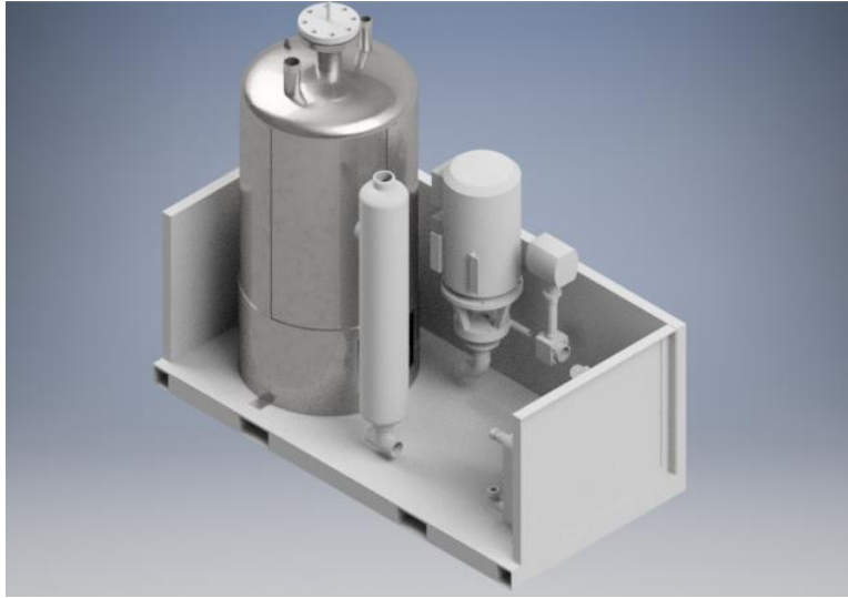
Figure 38. Renderings of the new refrigeration/cooling cold box.
