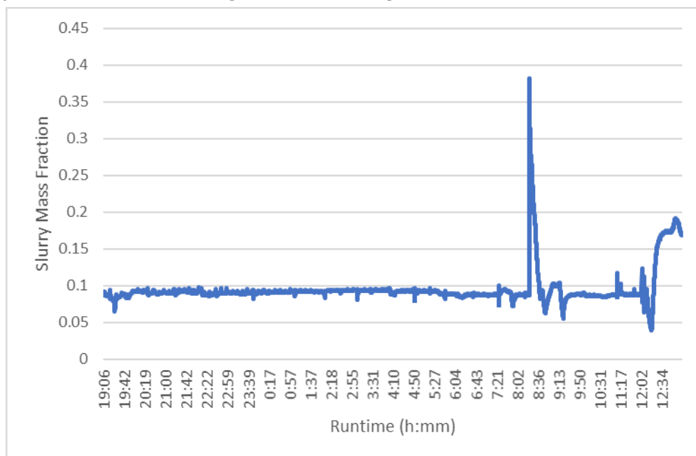
Figure 77. Mass fraction of the slurry over a 24-hour period while the impulse vibrator on the spray tower operates every 10 minutes.
