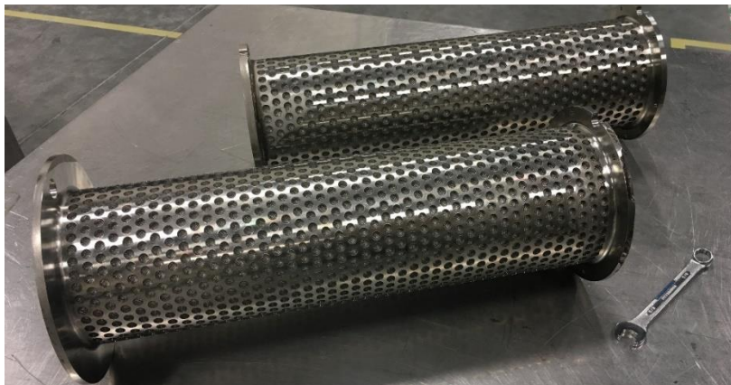
Figure 64. Completed filters for new screw press.
