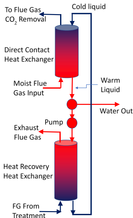
Figure 4. Schematic diagram of DCPC dryer.
