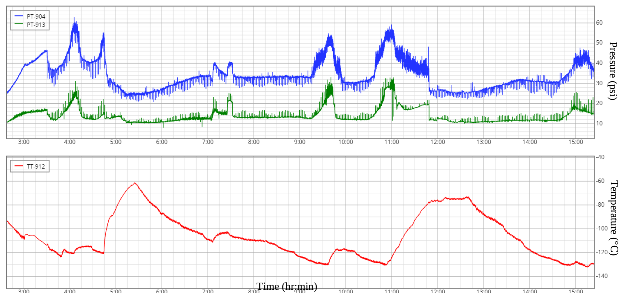
Figure 83. Pressure before (PT-913) and after (PT-904) the contact liquid heat exchanger compared with the contact liquid temperature (TT-912).
