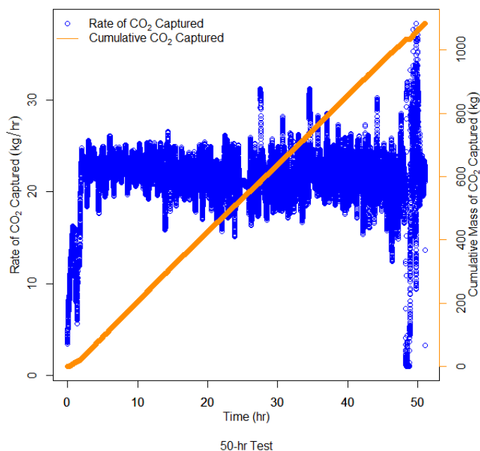
Figure 28. CO 2 capture rate and total cumulative mass captured [6].
