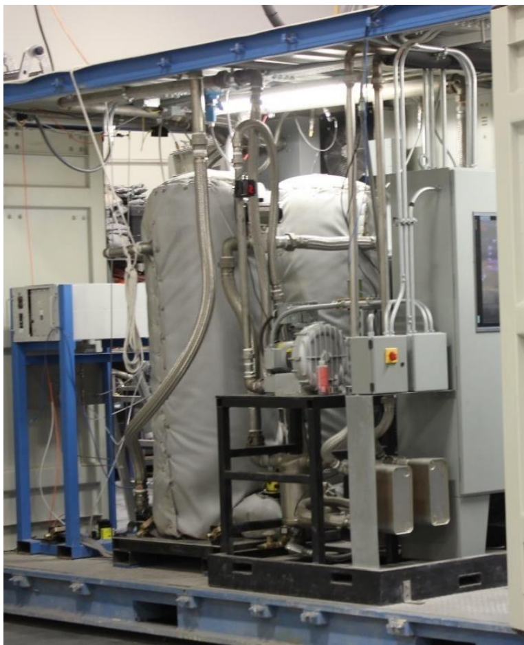
Figure 44. Mol sieve dryer integrated with the CCC ECL™ Skid. Both beds are covered with blankets of gray fiberglass insulation.
