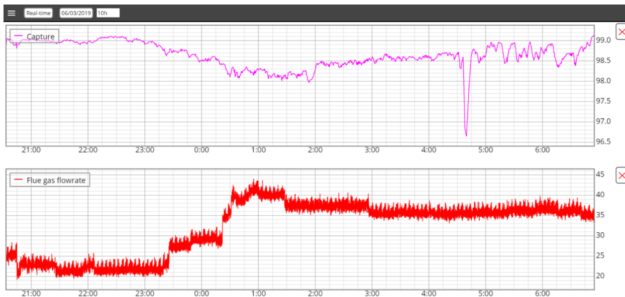
Figure 74. Data output from the SES historian showing data during the test on June 3–4, 2019. Both plots have units of hours and minutes for the x axis. The y axis of the top plot is CO 2 capture (%). The y axis of the bottom plot is flue gas flow rate (kg/hr).
