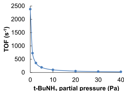
Figure 15. Predicted effect of t -BuNH 2 partial pressure on turnover frequency. T = 473\text{ K} ; P_{C_4} = 32\text{ kPa} ; P_{NH_3} = 69\text{ kPa} .
