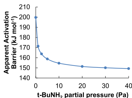
Figure 16. Predicted effect of t -BuNH 2 partial pressure on apparent activation barrier. T = 473\text{ K} ; P_{C_4} = 32\text{ kPa} ; P_{NH_3} = 69\text{ kPa} .
