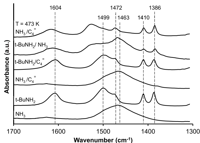
Figure 11. FTIR difference spectra of MFI-15 taken 1 h after introduction of isobutene, \text{NH}_3 , or t\text{-BuNH}_2 . Spectra were taken at 433 K unless otherwise specified.
