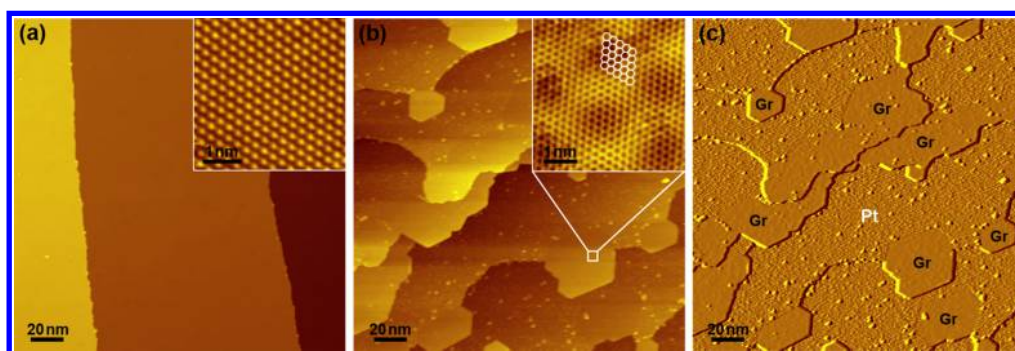
Figure 1. STM images showing graphene nucleation on flat Pt(111) substrate prepared using method 1. (a) STM image of the clean Pt(111) surface with atomic structure resolved in the inset. (b) STM topography and (c) derivative image of the Pt surface after graphene nucleation at 1223 K. Graphene islands (smooth areas) are found and can be distinguished easily in the derivative image (c). The atomic structure of a graphene island is shown in the inset of (b). Imaging parameters: (a) sample bias voltage V_s = 200 mV, tunneling current I_t = 15 pA; (inset) V_s = 27 mV, I_t = 200 pA; (b) V_s = 300 mV, I_t = 14 pA; (inset) V_s = 20 mV, I_t = 400 pA.
