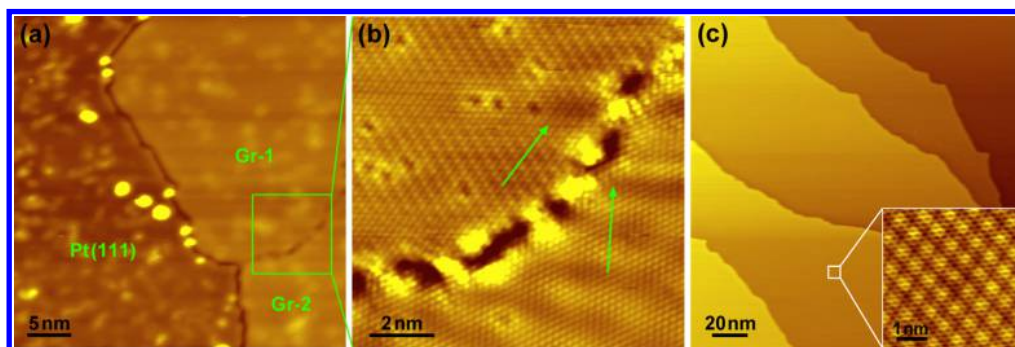
Figure 5. Grain boundary formation during graphene growth on the flat Pt substrate. (a) Two graphene islands merge with different lattice orientations, forming a grain boundary. The sample was grown using method 1. (b) An expanded view of the atomic structure near the boundary, where two grains are rotated \sim 27^\circ with each other. (c) Growth method 2 produced a continuous high-quality graphene film over the Pt terraces, with atomic structure shown in the inset. Imaging parameters: (a, c) V_s = 200 mV, I_t = 14 pA; (b) V_s = 18 mV, I_t = 400 pA; inset in (c): V_s = 16 mV, I_t = 200 pA.
