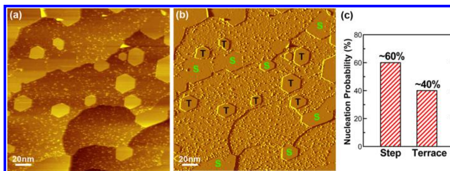
Figure 2. STM topography (a) and derivative (b) images showing the nucleation of graphene islands on the flat Pt(111) substrate using growth method 1. The hexagonal graphene islands are clearly visible in (b), which are marked with "S" or "T" according to their locations (near a step edge or on a terrace). Imaging parameters: V_s = 300 mV, I_t = 14 pA. (c) Statistical data over 300 graphene islands indicate that about 60% of them are located near a step and 40% are on top of a terrace.
