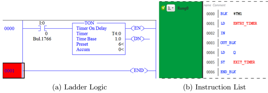
Fig. 1: Different representations of a timer program
