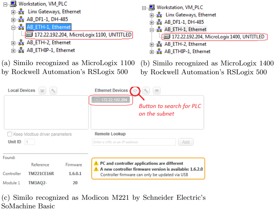
Fig. 7: Similo recognized as a real PLC (MicroLogix 1100 and 1400 and Modicon M221) by two engineering software, RSLogix 500 and SoMachine Basic
